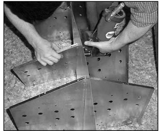
Fasten two partitions to back using THREE rivets.
