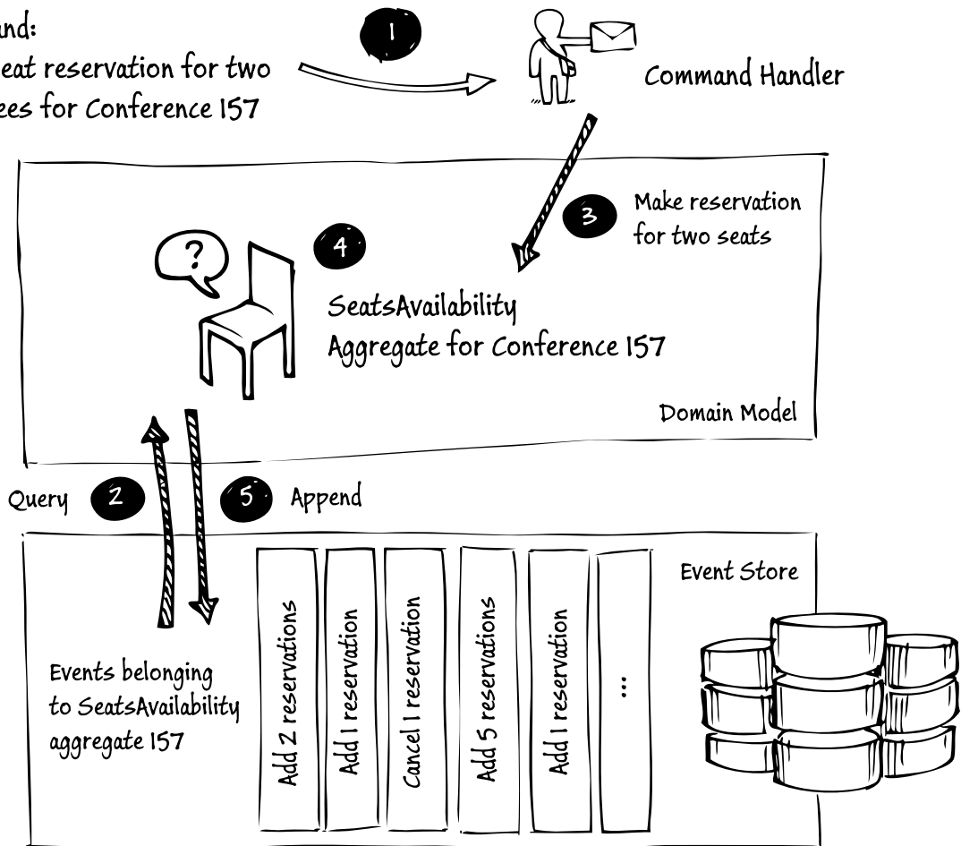
FIGURE 2 Using event sourcing
