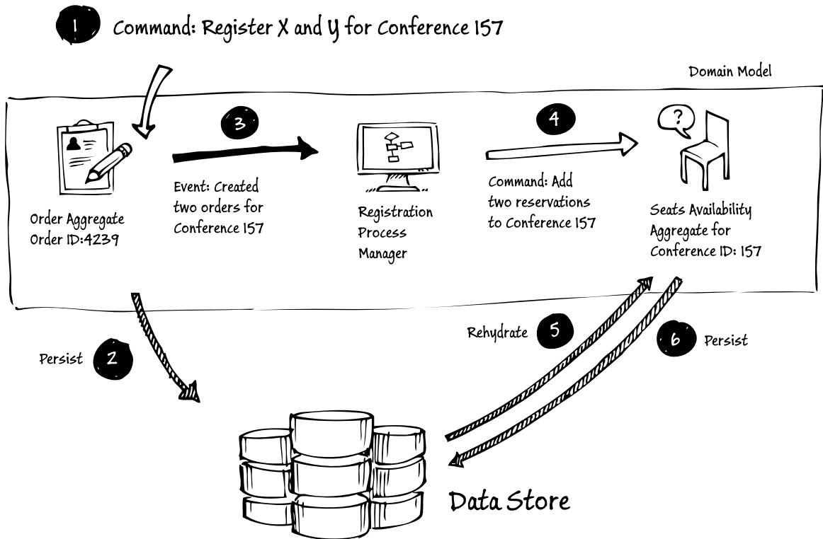
FIGURE 4 Approach 3: Using a process manager
