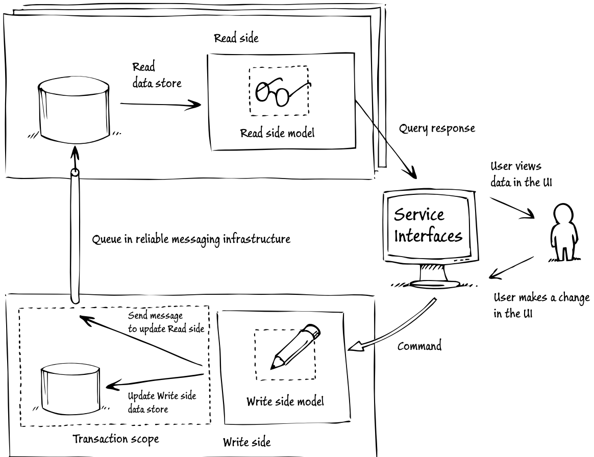
FIGURE 2 Using a reliable message transport
