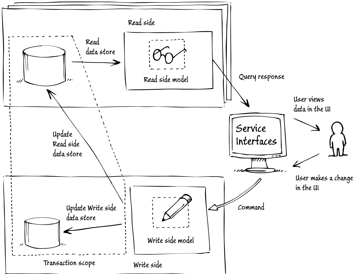
FIGURE 1 Using a distributed transaction to maintain consistency
