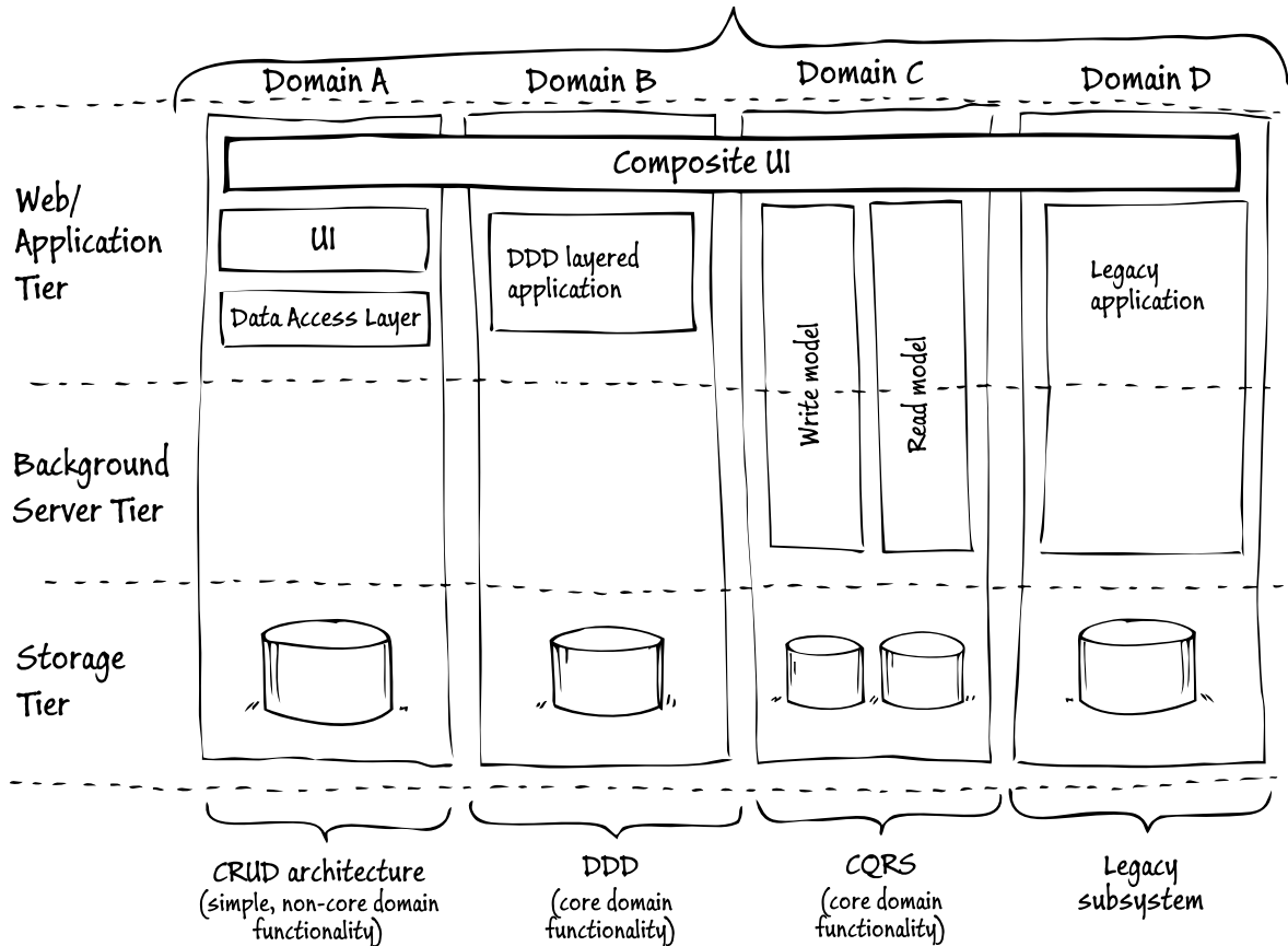
FIGURE 2 Multiple architectural styles within a large, complex application
