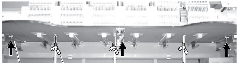
Clamp Upper set screw Table stay Fig. 5
