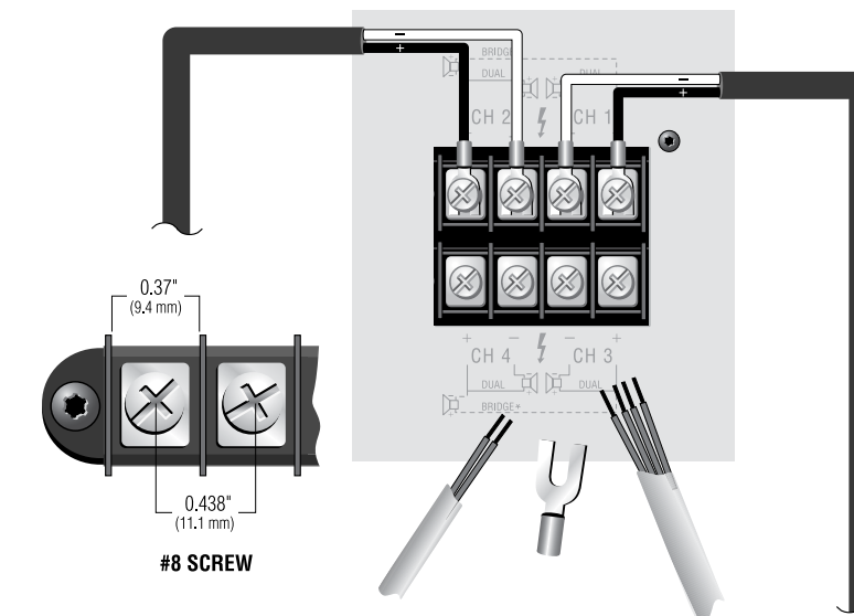
Figure 3.5 Output Connector Wiring (Typical of two channels)
