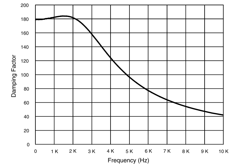
Figure 7.5 CTs 8200 Typical Damping Factor vs. Frequency
