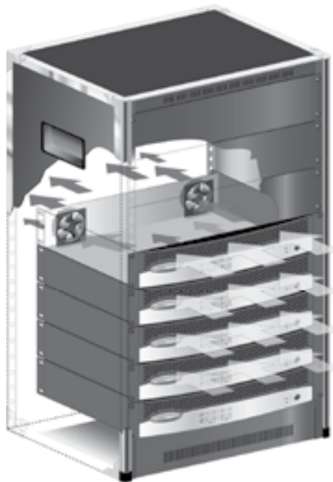
Figure 3.2 Airflow
