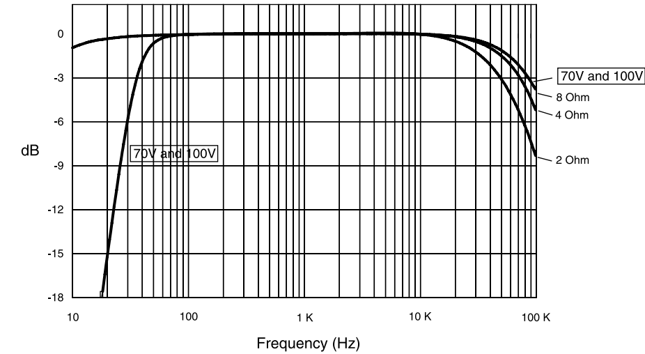
Figure 7.3 CTs 8200 Typical Frequency Response (1 W)
