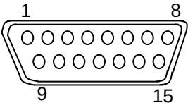
15P Connector(Female) (17JE-13150-02(D8A6)A-CG (DDK)
