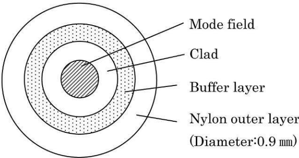
Cross section drawing of optic fiber
