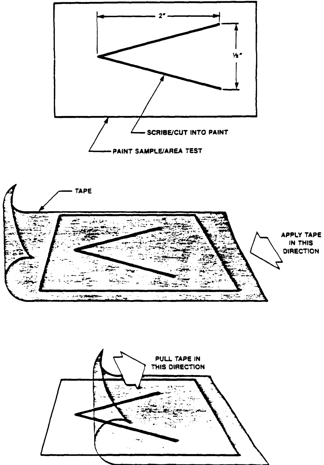
Figure 3-1. Tape Test.
