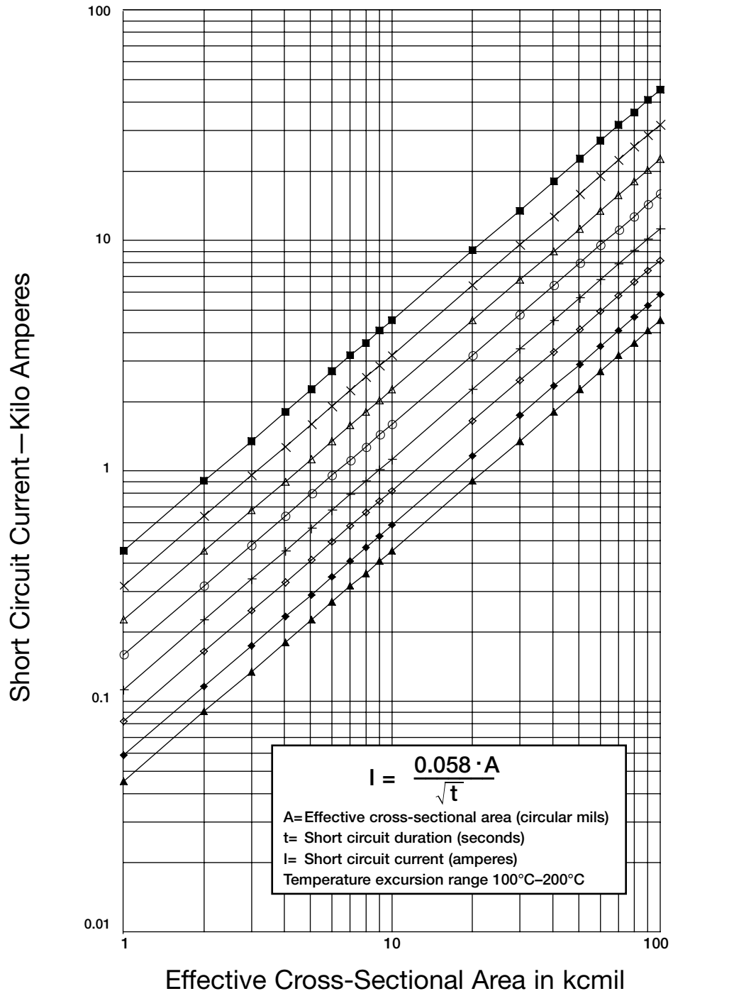
Allowable Copper Shield Short Circuit Currents for 5–15 kV
