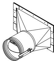
3300-D 45° TAKEOFF with DAMPER
