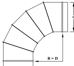
SP6111 90° ELBOW 14" - 38" 5 Piece Gorelock
