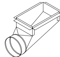
244-F CENTER END BOOT with DRYWALL FLANGE
