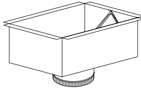
905 RETURN AIR BOX 10" DEEP with "A" RACK for 2 FILTERS
