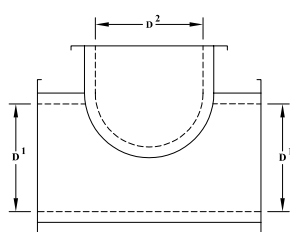
DW6271 90° TEE
