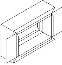
"PR" PASSIVE RETURN AIR SLEEVE
