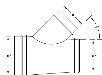
SP6276R REDUCING LATERAL
