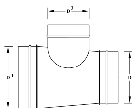
SP6271R REDUCING TEE
