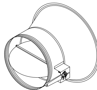
3200-DS CONICAL SPIN-IN with 3/8" SOLID ROD AXIS & 2" STANDOFF (14" - 20")
