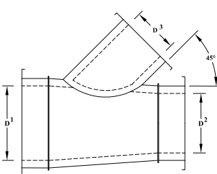
DW6276R REDUCING 45° LATERAL
