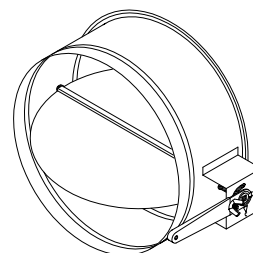
3720-DS SPIN-IN TAKEOFF with \frac{3}{8} " SOLID ROD AXIS & 2" STANDOFF (14" - 20")
