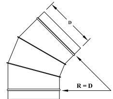
SP6121 45° ELBOW 14" - 38" 3 Piece Gorelock
