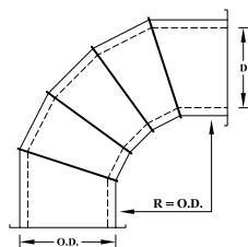
DW6111 90° ELBOW 5 Piece Gorelock
