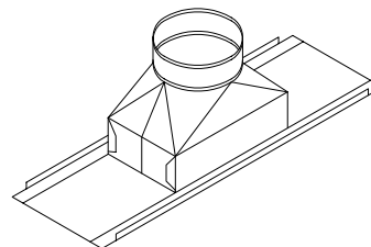
356 PLASTER FRAME with STRAIGHT BOOT INSTALLED
