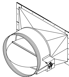
3300-DS 45° TAKEOFF with \frac{3}{8} " SOLID ROD AXIS & 2" STANDOFF (14" - 20")
