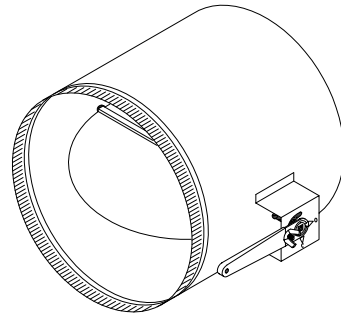
175-XS2 DAMPER SLEEVE with \frac{3}{8} " SOLID ROD AXIS & 2" STANDOFF (14" - 20")
