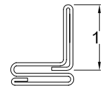
STANDING S-LOCK
