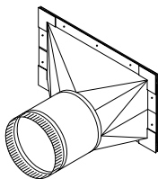
3300 45° TAKEOFF
