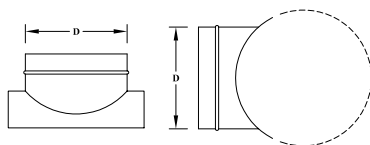
SP6307 90° SADDLE TAP
