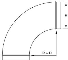
SP6111 90° ELBOW 4" - 12" Die Stamped
