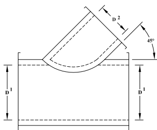
DW6276 45° LATERAL
