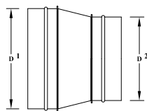
SP6265 REDUCER
