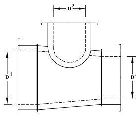
DW6271R REDUCING 90° TEE
