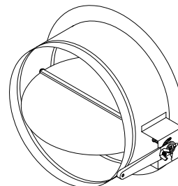
3710-DS TAKEOFF with \frac{3}{8} " SOLID ROD AXIS & 2" STANDOFF (14" - 20")
