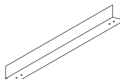
1260 MOUNTING ANGLE 18 GAUGE, 1½" x 1½" x 26" LONG
