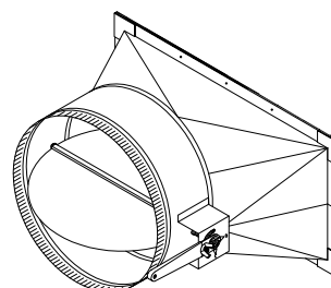
3400-DS TAKEOFF CENTER TAPER with \frac{3}{8} " SOLID ROD AXIS & 2" STANDOFF (14" - 20")
