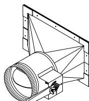
3300-DS2 45° TAKEOFF with \frac{3}{8} " SOLID ROD AXIS & 2" STANDOFF (4" - 12")
