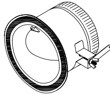
714-DSO with DAMPER and 2" STANDOFF
