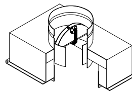
1575-CRD CEILING RADIATION DAMPER BOX TOP ENTRY COLLAR
