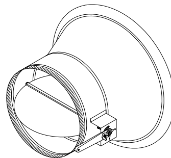
3210-DS CONICAL with \frac{3}{8} " SOLID ROD AXIS & 2" STANDOFF (14" - 20")
