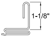
1" STANDING BAR-LOCK
