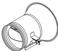
3200-DS CONICAL SPIN-IN with 2" DAMPER HANDLE STANDOFF (4" - 12")
