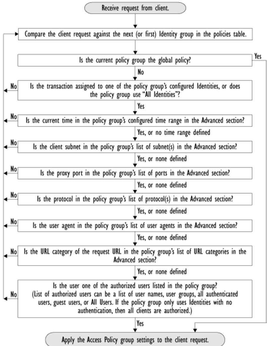
Figure 8-1 Policy Group Flow Diagram for Access Policies
