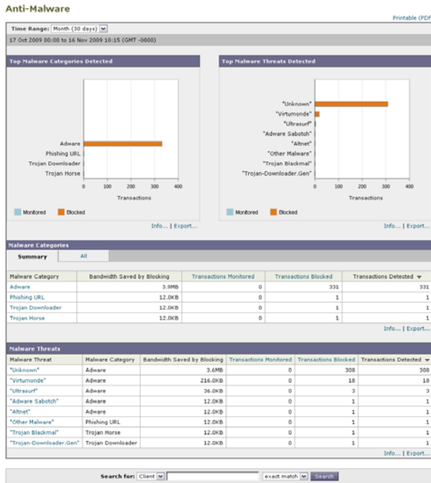
Figure 23-7 Anti-Malware Page
