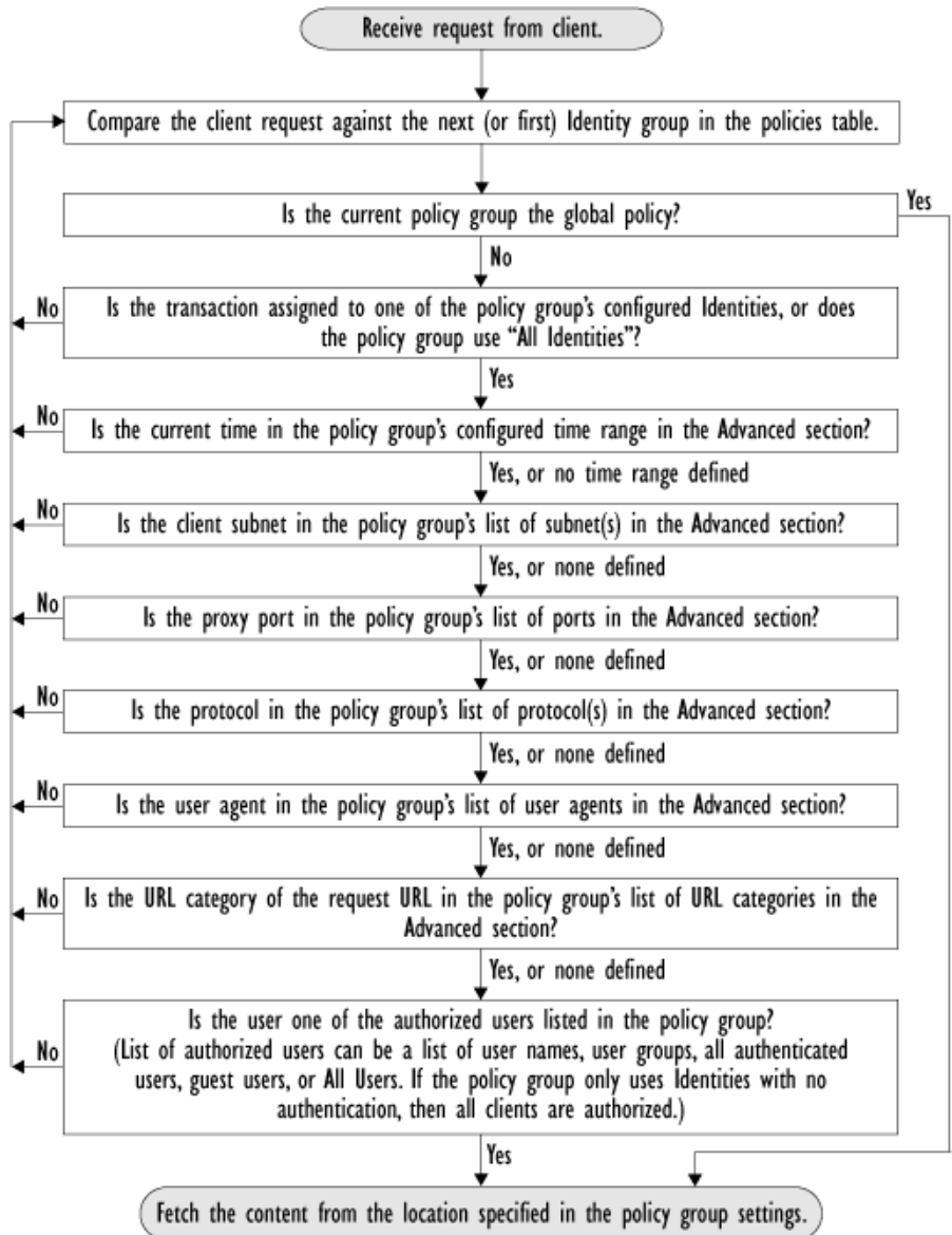
Figure 9-2 Policy Group Flow Diagram for Routing Policies
