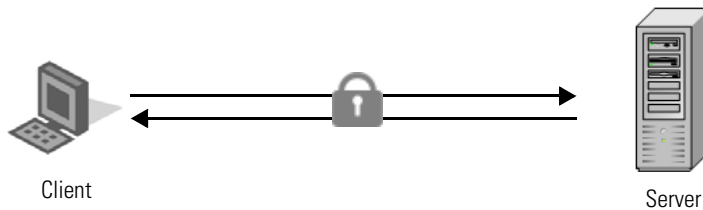
Figure 10-3 HTTPS Connection
