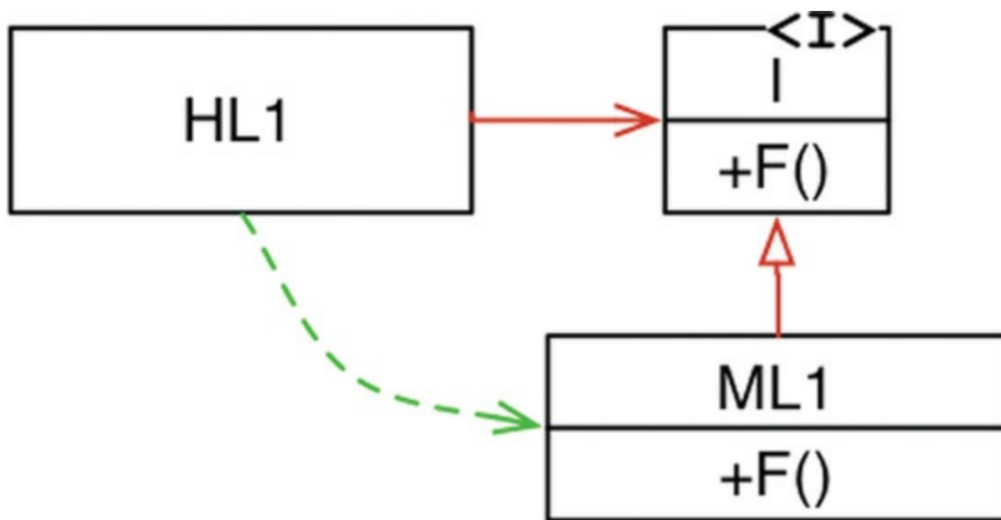
Figure 5.2 Dependency inversion
