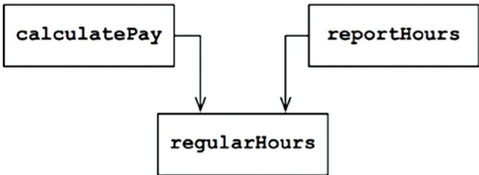
Figure 7.2 Shared algorithm
