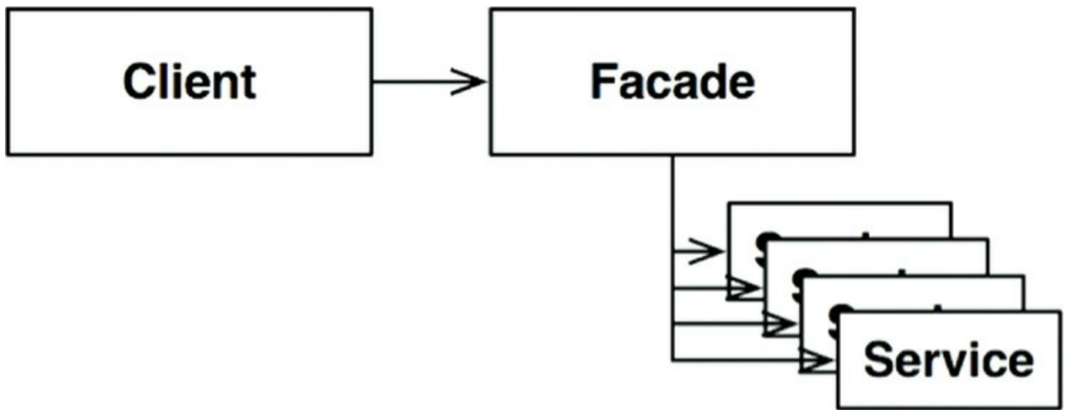
Figure 24.2 The Facade pattern
