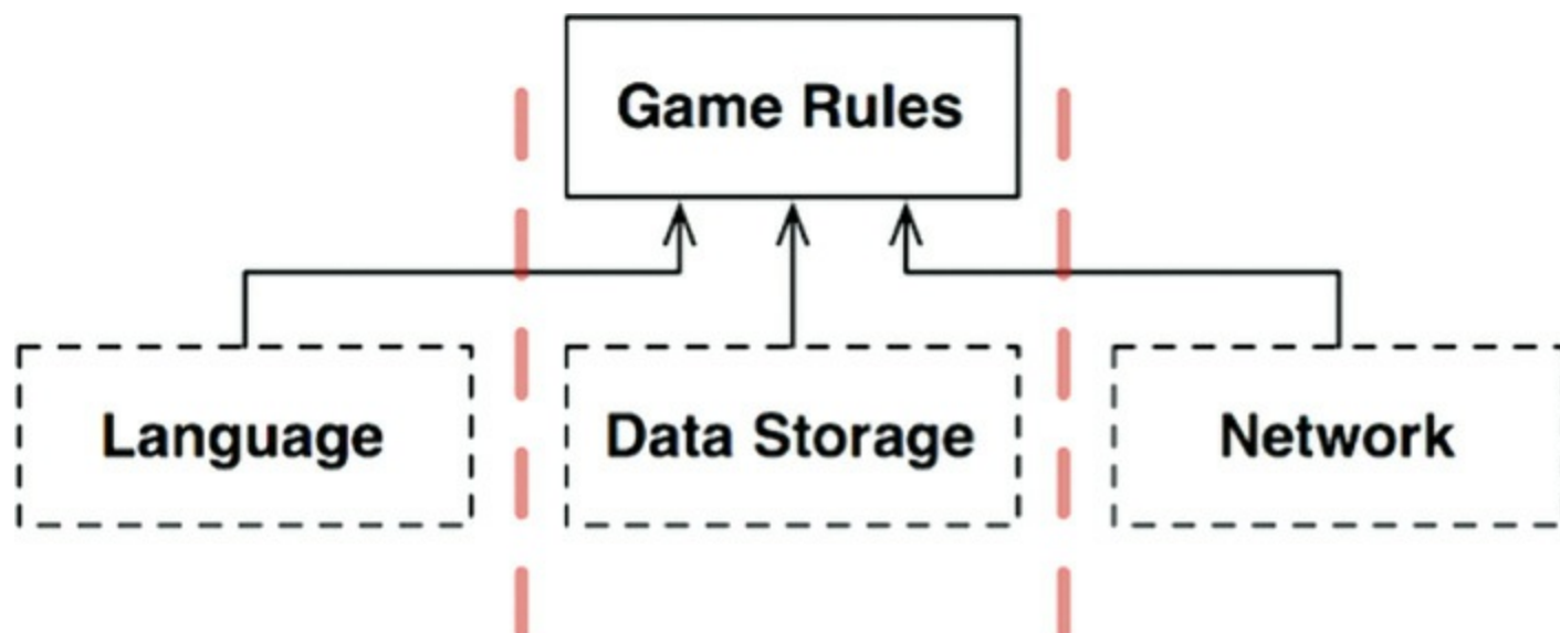
Figure 25.5 Adding a network component
