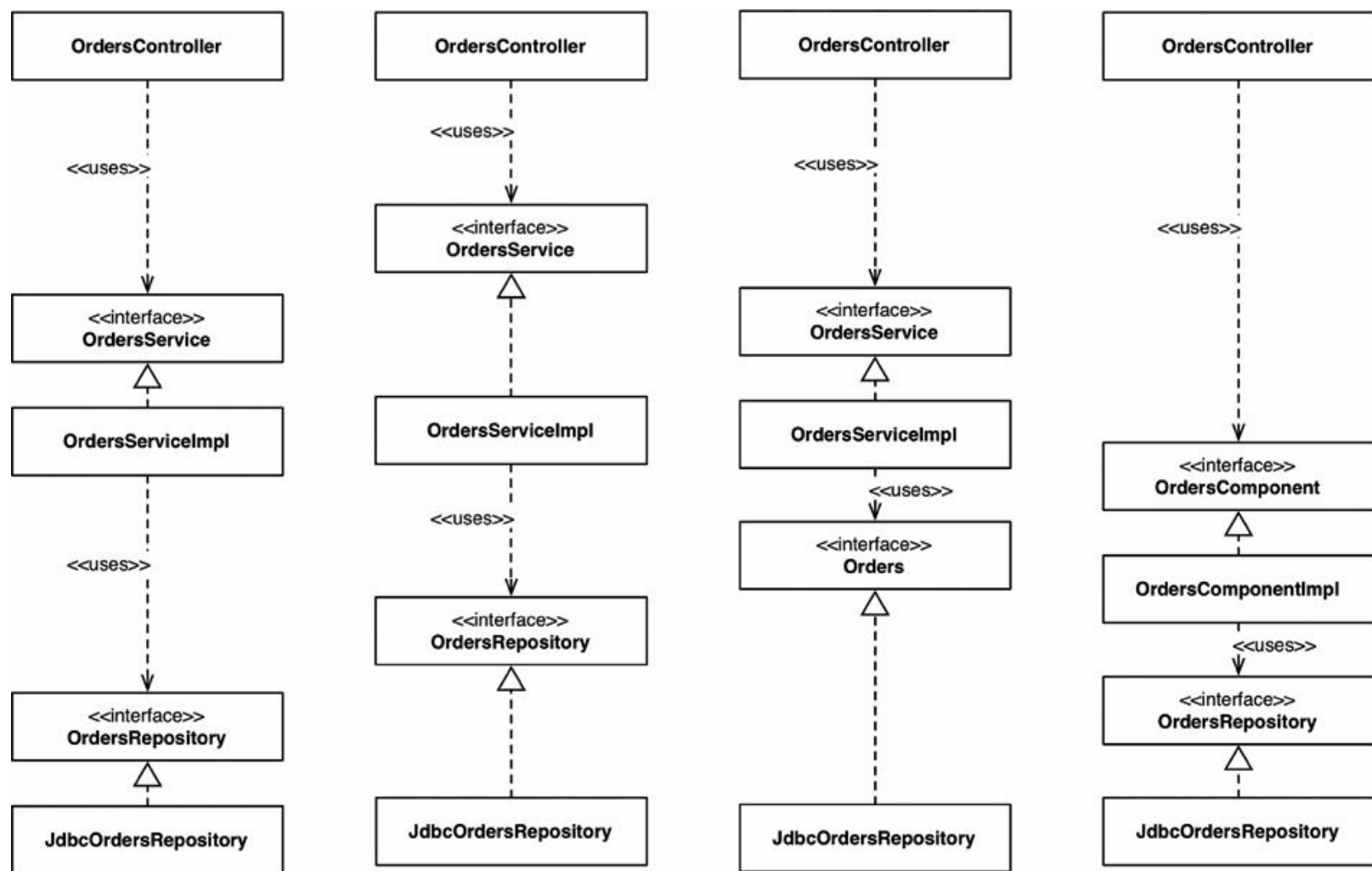
Figure 34.7 All four architectural approaches are the same
