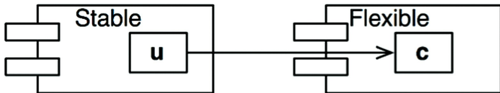
Figure 14.10 U within Stable uses C within Flexible
