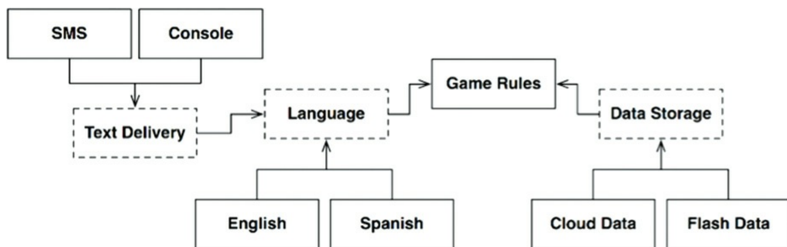
Figure 25.3 The revised diagram
