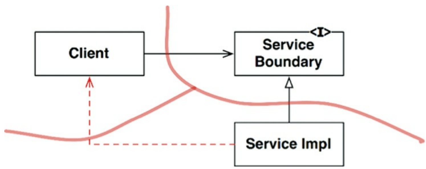
Figure 24.1 The Strategy pattern
