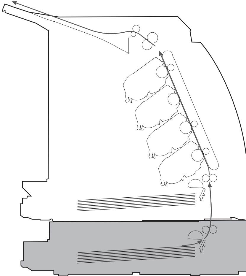
Figure 6-1 Paper path
