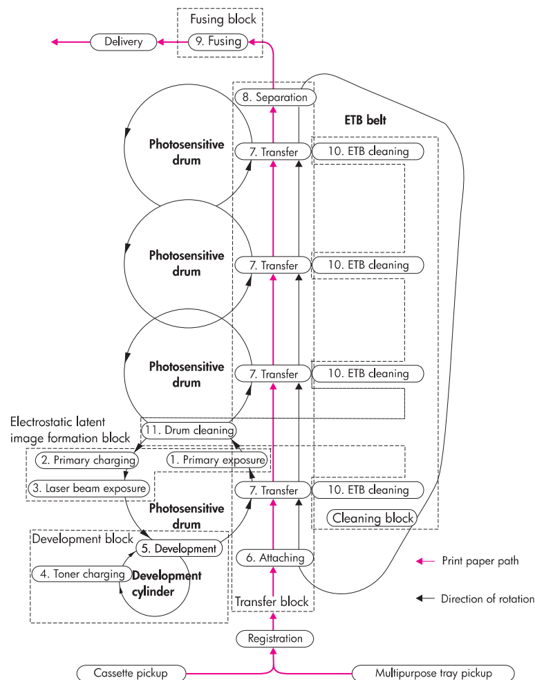
Figure 5-14 Image-formation process
