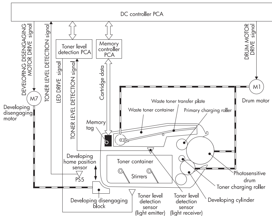
Figure 5-15 Print cartridge
