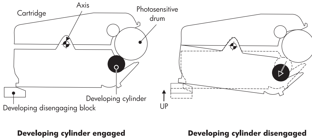
Figure 5-18 Developing cylinder disengaging
