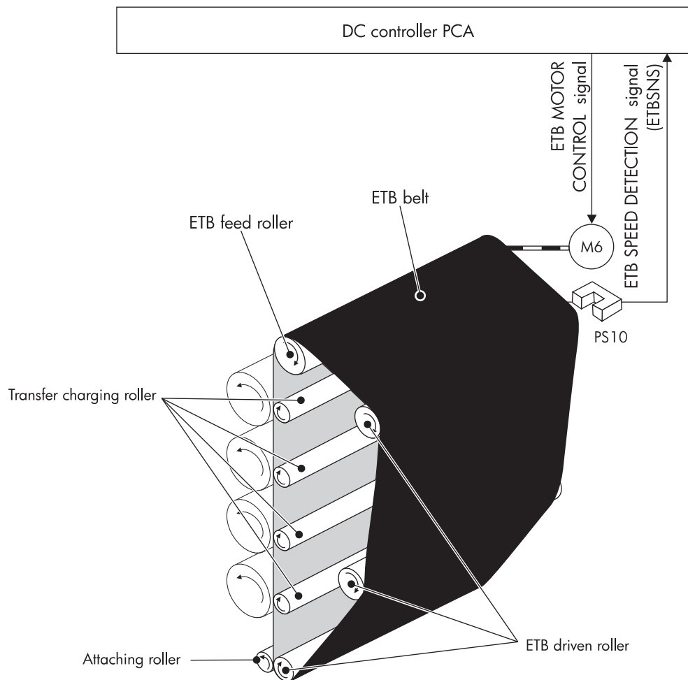
Figure 5-19 ETB unit
