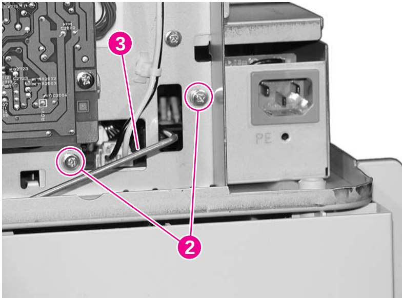
Figure 6-45 Remove the low-voltage power supply (2 of 3)
