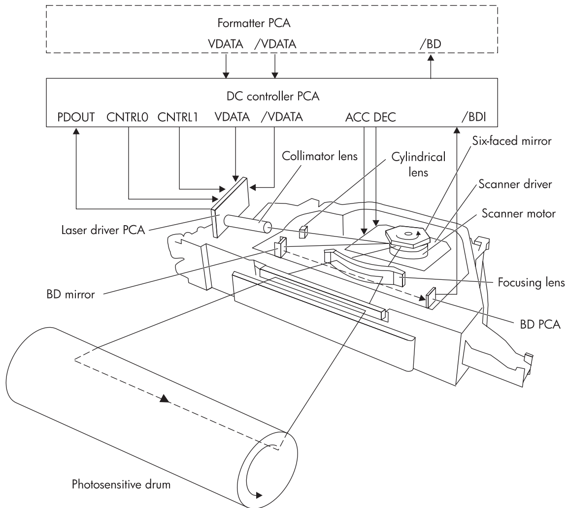
Figure 5-11 Laser/scanner system
