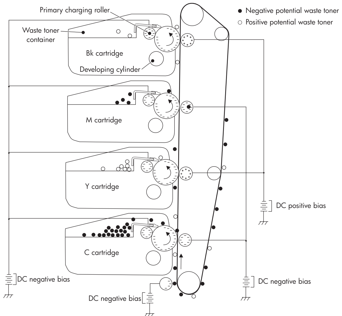
Figure 5-28 ETB cleaning
