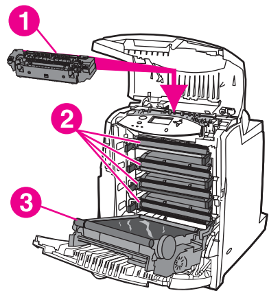
Figure 4-2 Location of supplies
