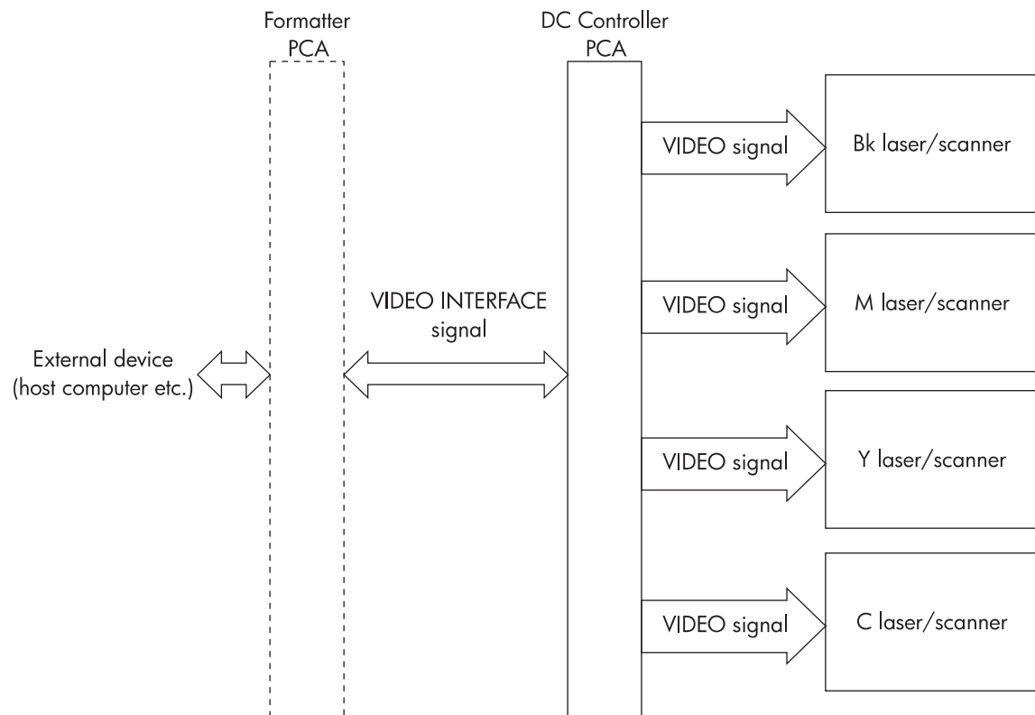
Figure 5-10 Formatter system
