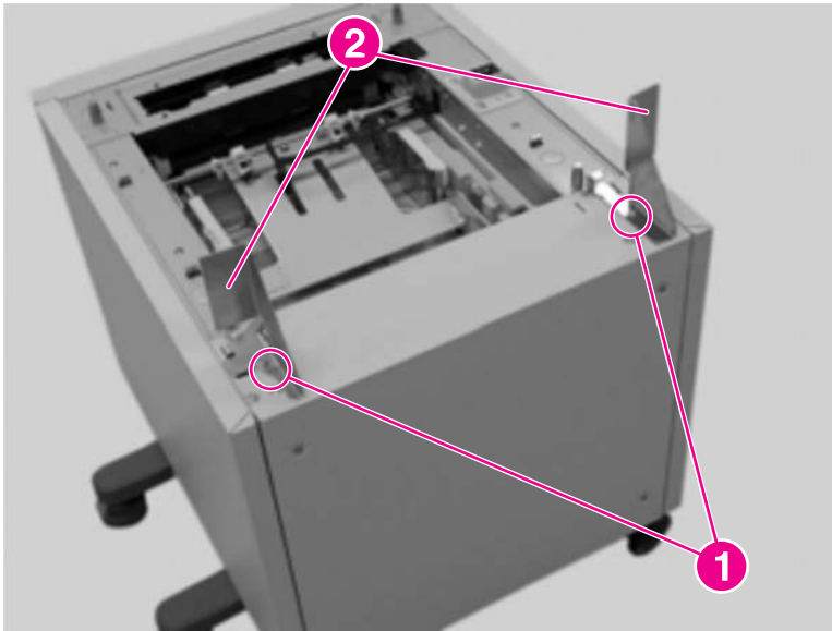
Figure 6-79 Remove the 2 x 500-sheet paper feeder rear cover (1 of 2)
