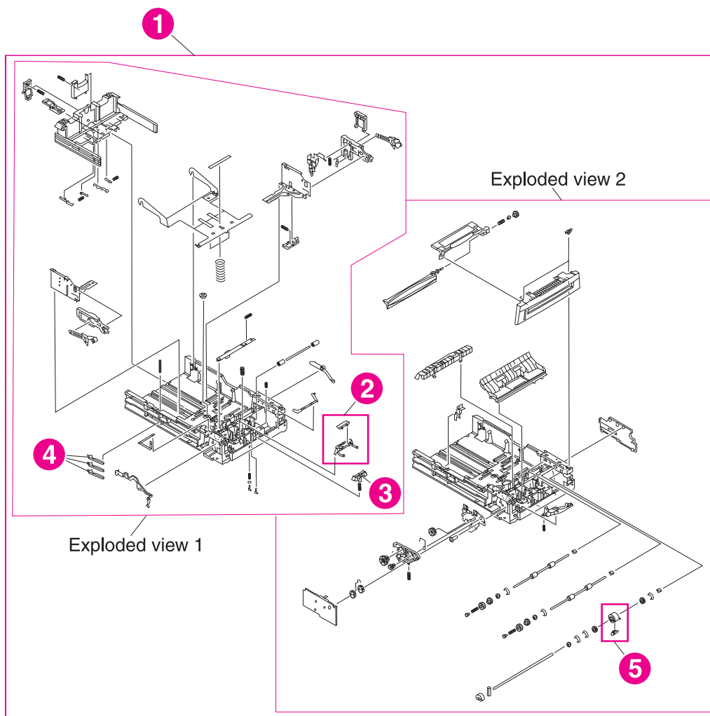
Figure 8-13 Cassette (tray 2)
