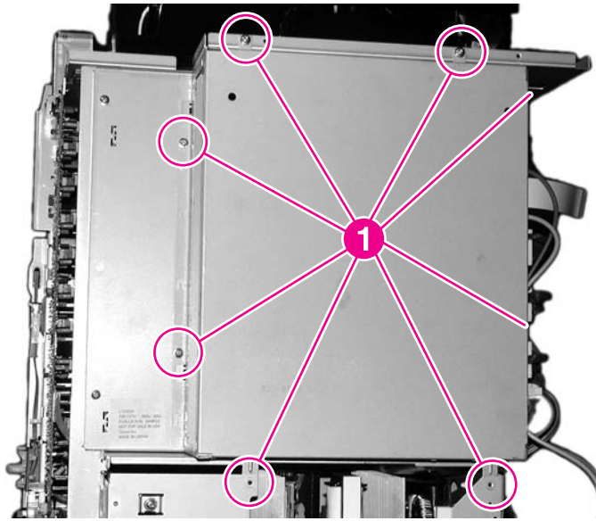
Figure 6-49 Remove the formatter case (1 of 2)
