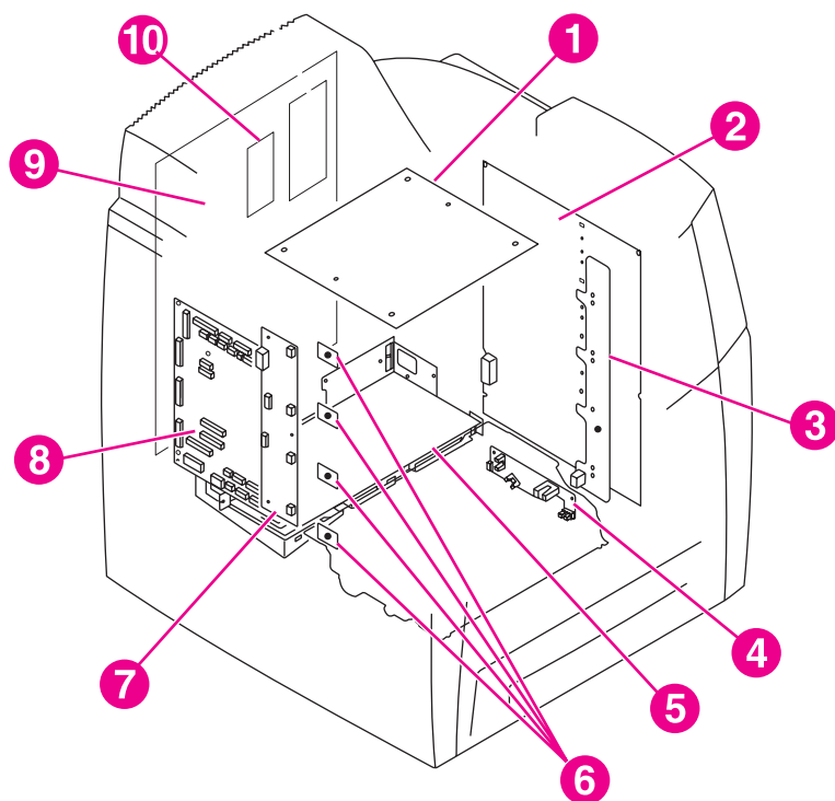
Figure 7-43 PCA locations
