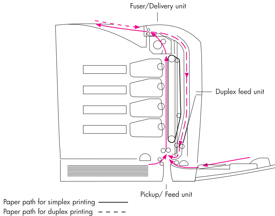
Figure 5-34 Pickup/feed system
