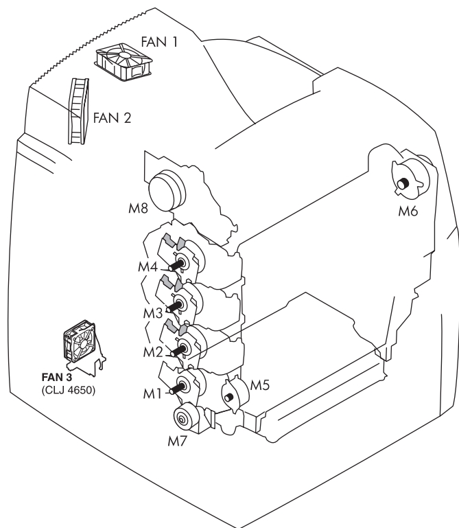
Figure 7-41 Location of motors and fans
