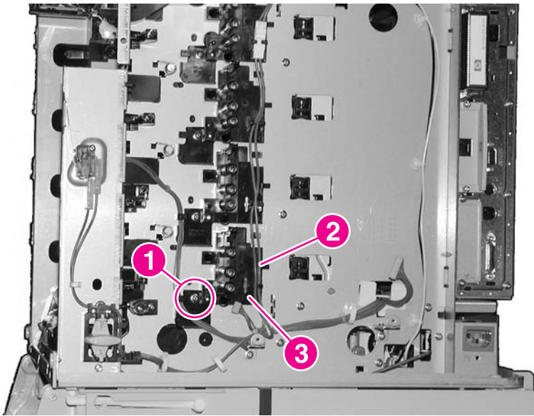
Figure 6-62 Remove the high-voltage contact blocks (cyan is shown)
