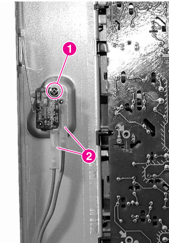
Figure 6-63 Remove the door switch
