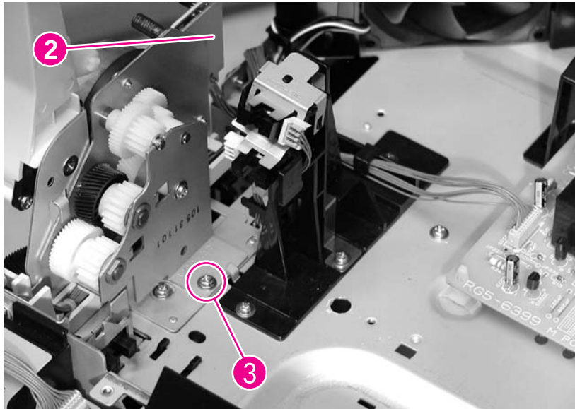
Figure 6-67 Remove the fuser drive unit (2 of 2)
