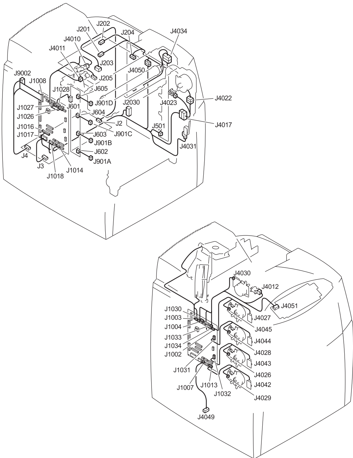
Figure 7-47 Location of connectors (HP Color LaserJet 4600 models)
