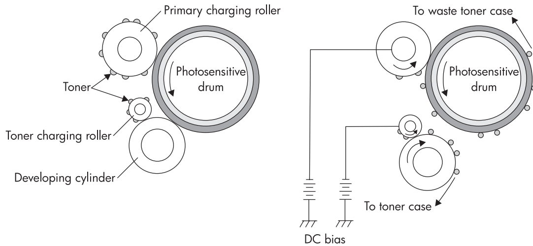
Figure 5-30 Primary charging roller and toner charging roller cleaning
