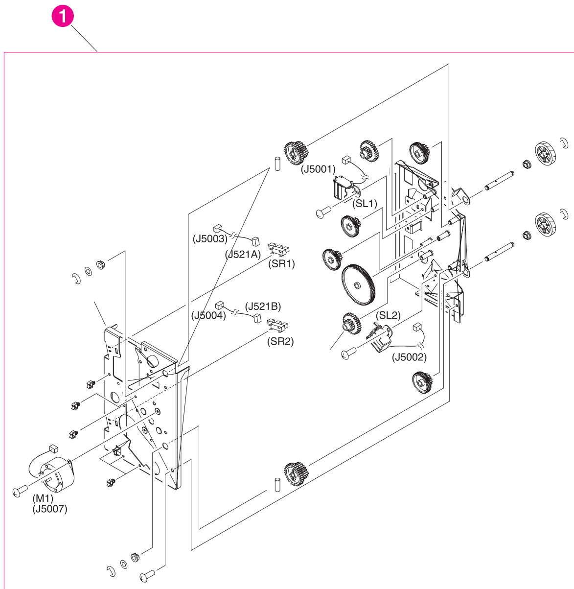
Figure 8-22 2 x 500-sheet feeder paper pickup drive assembly (HP CLJ 4650 models only)
