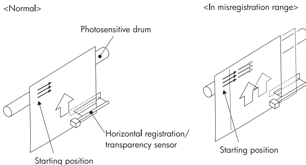
Figure 5-40. Horizontal registration adjustment
