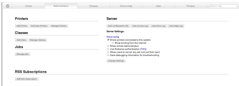
Figure 17-3 The CUPS administration screen
