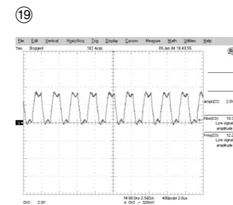
CN401 PIN20:AIN_MCLKOUT
