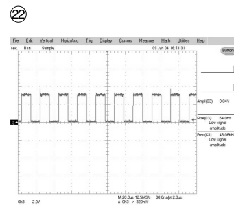
CN400 PIN5:AIN_FSYNC
