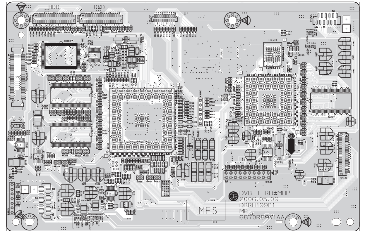
( BOTTOM VIEW )
