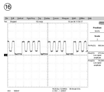
CN400 PIN6:VOUT_B/Pb
