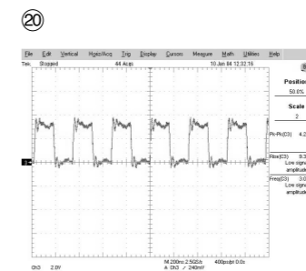
CN401 PIN7:AIN_SCLK
