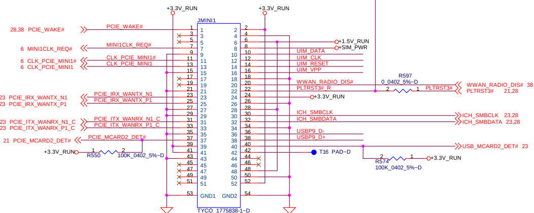
Mini-Card Latch
