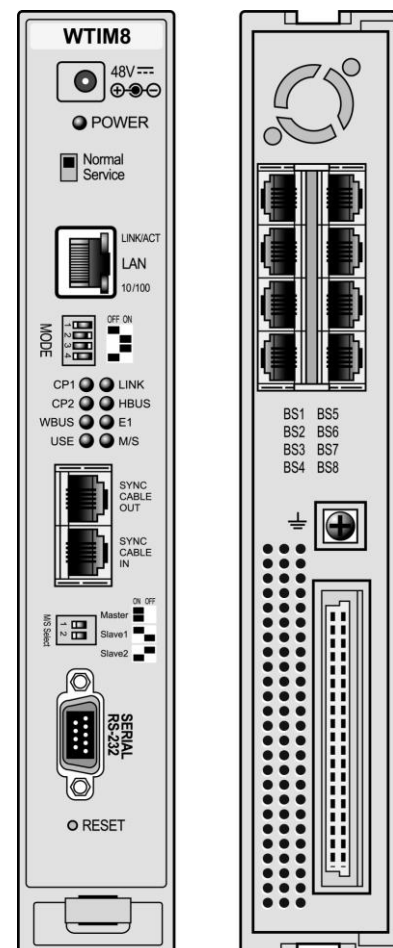
Figure 2.1.13.2-1 WTIM8 Front & Rear Panels
