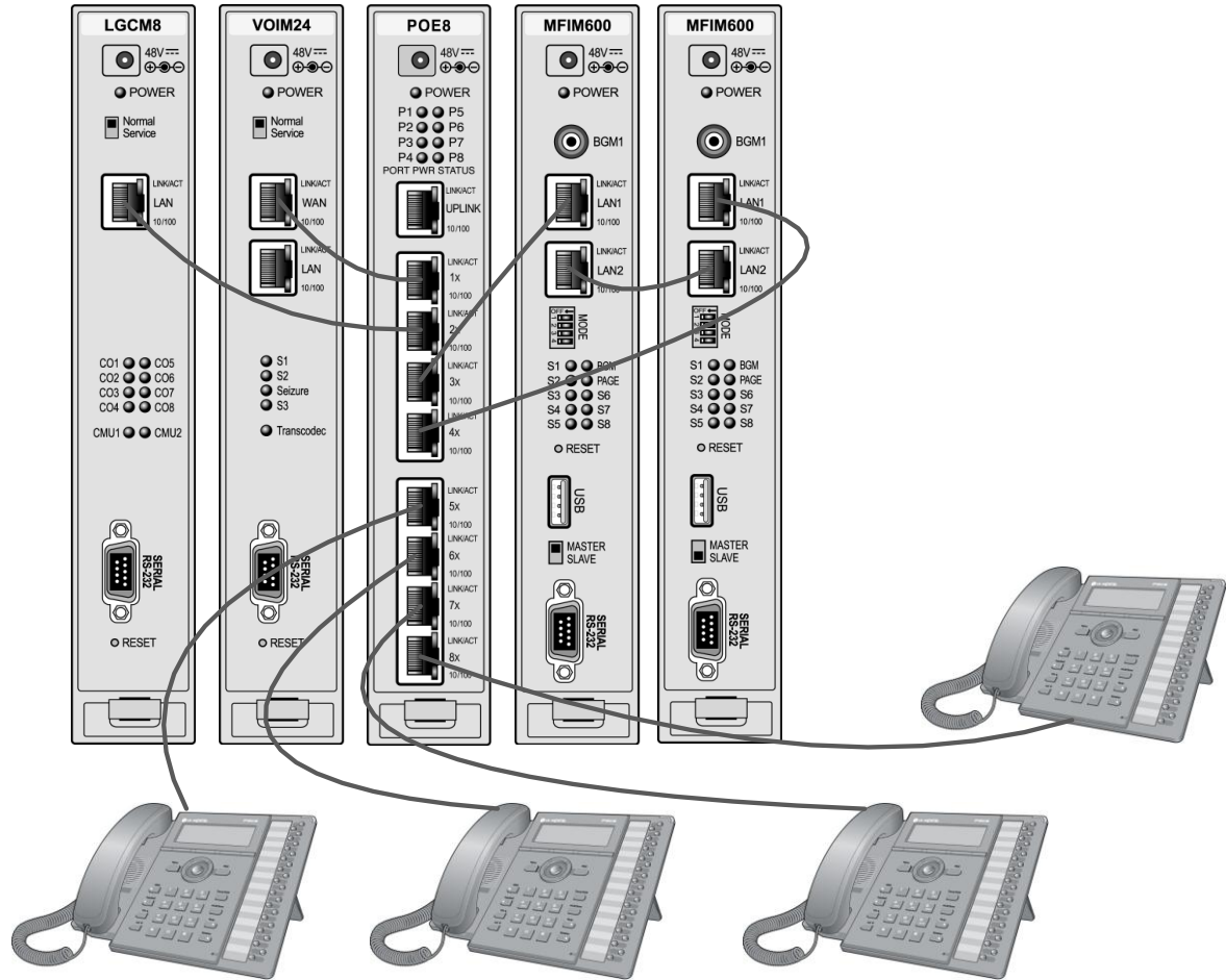
Figure 4.5.18-1 POE8 Installation with MFIM600 Redundancy
