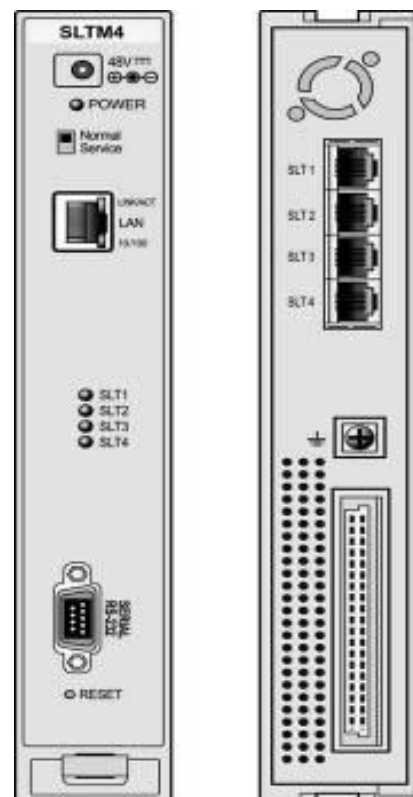
Figure 2.1.6.1-1 SLTM4 Front & Rear Panels
