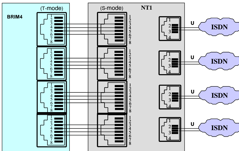
Figure 4.5.13-1 BRIM4 BRI Line Connector Configuration
