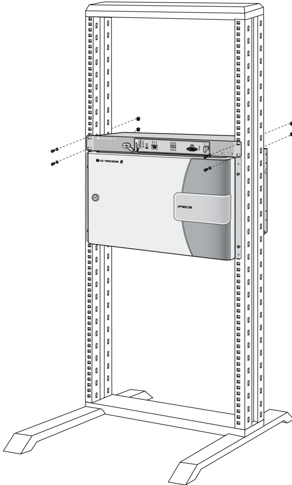
Figure 4.3.5-3 1U-RMB Rack-mount Installation
