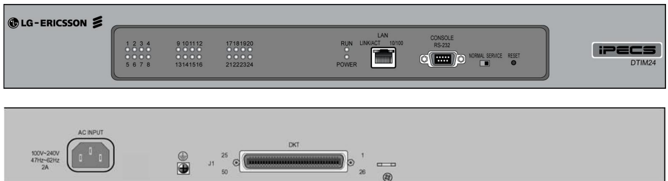
Figure 2.1.5.2-1 DTIM24 Front & Rear Panels
