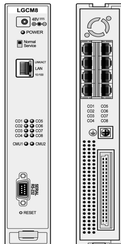
Figure 2.1.3.2-1 LGCM8 Front & Rear Panels
