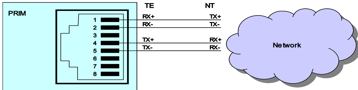
Figure 4.5.14-1 PRI Line Connector Configuration
