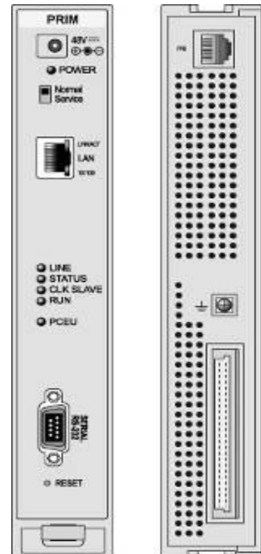
Figure 2.1.8-1 PRIM Front & Rear Panels
