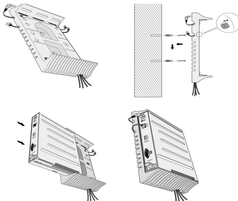
Figure 4.3.4-1 Module Wall Mount Holder Kit
