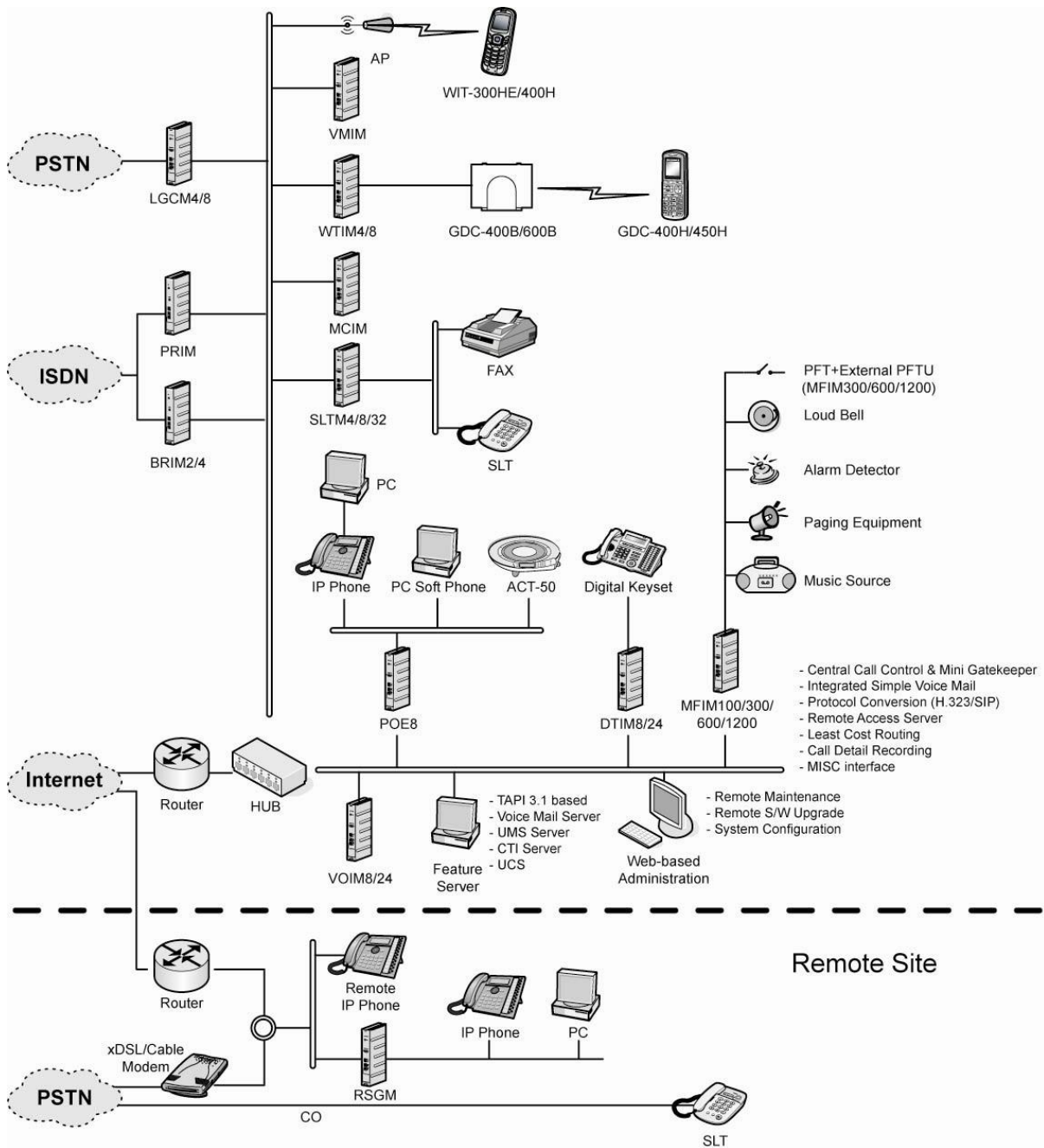
Figure 1.1-1 iPECS Structure
