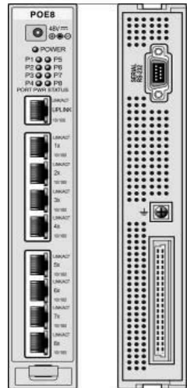
Figure 2.1.12-1 POE8 Front & Rear Panels
