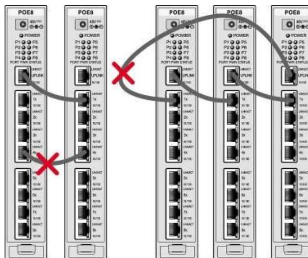
Figure 4.5.1.7-2 Erroneous Loop Wiring
