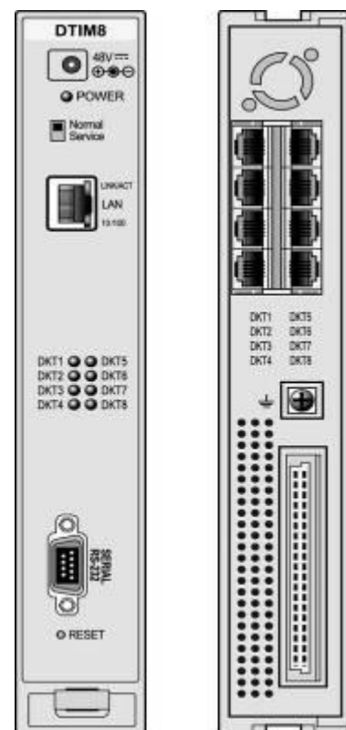
Figure 2.1.5-1 DTIM8 Front & Rear Panels
