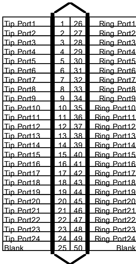
Figure 4.5.8-2 DTIM24 RJ-21X Connector Configuration
