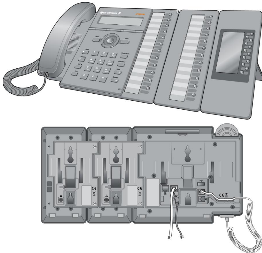
Figure 4.7-4 LIP-8000 DSS Installation (12DSS + 12LS)
