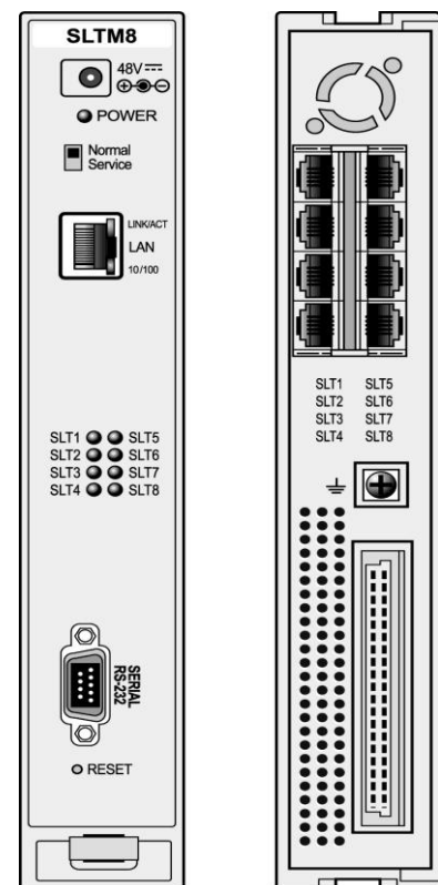
Figure 2.1.6.2-1 SLTM8 Front & Rear Panels
