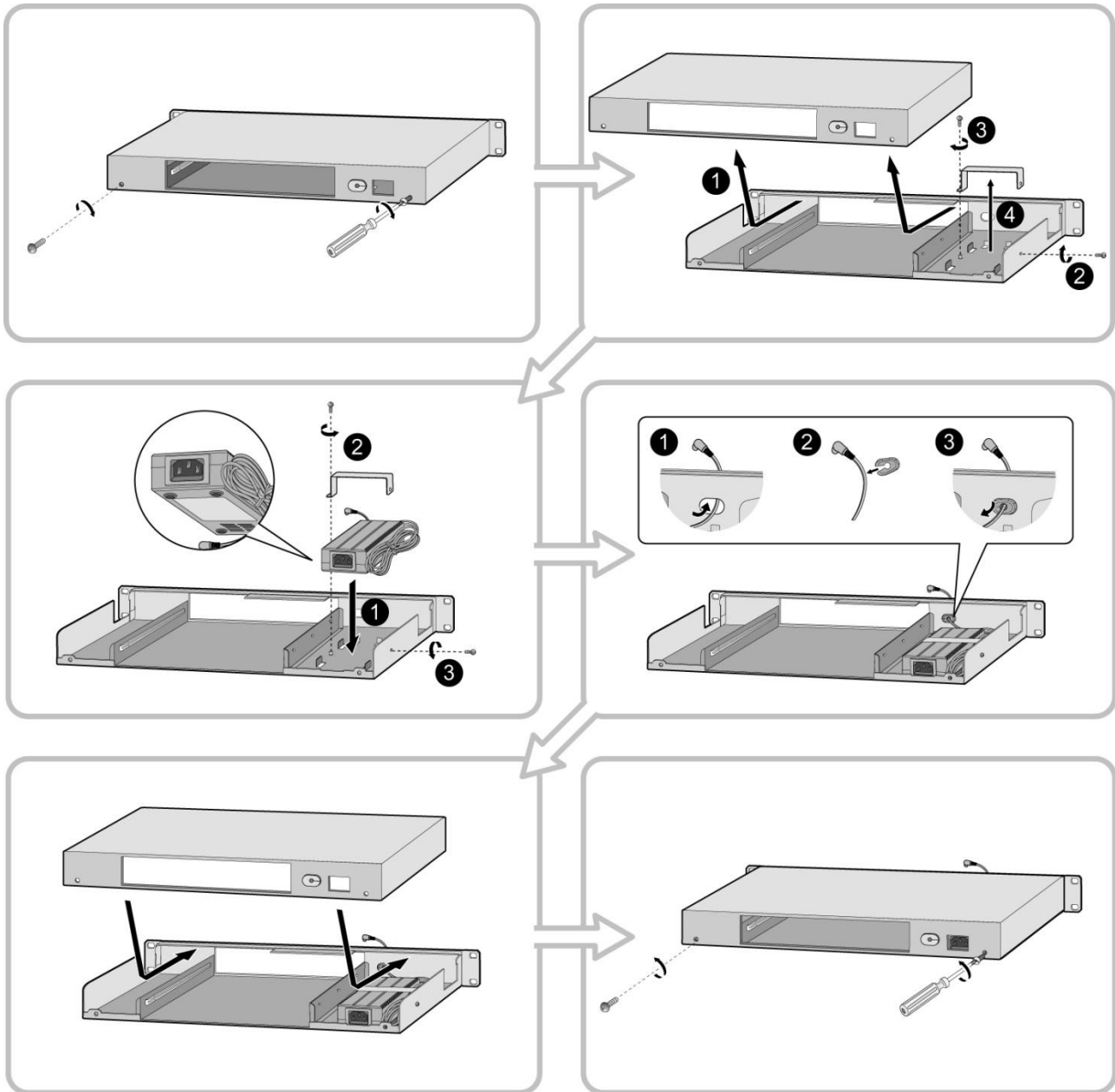
Figure 4.3.5-1 1U RMB Adapter Installation
