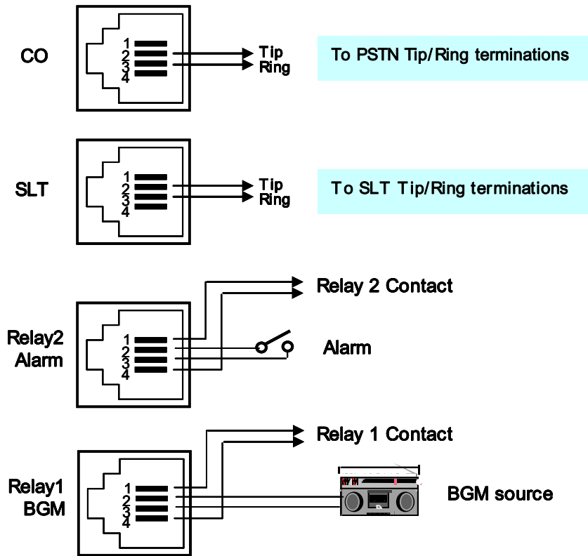
Figure 4.5.17-3 RSGM Connections
