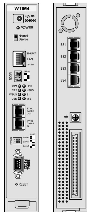
Figure 2.1.13.1-1 WTIM4 Front & Rear Panels
