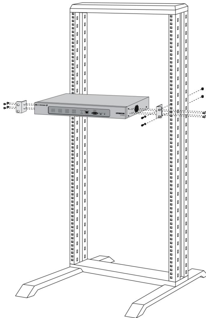
Figure 4.5.11-1 SLTM32 Rack Mounting Installation
