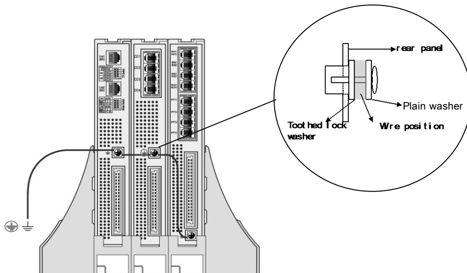
Figure 4.5.1.4-1 Module Grounding
