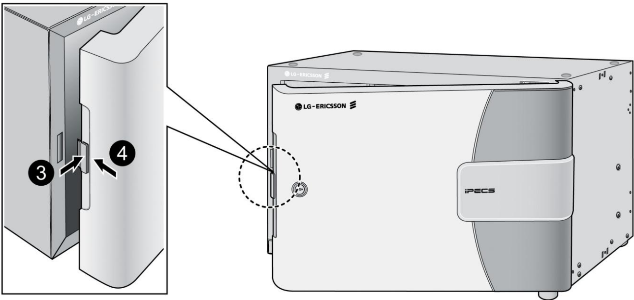
Figure 4.3.1.1-1 Cover installation
