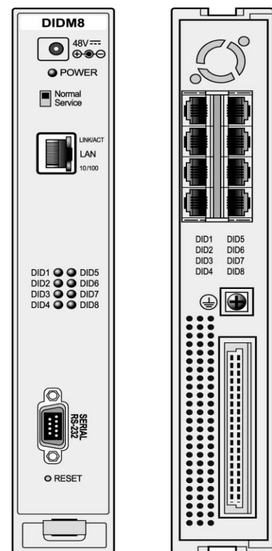
Figure 2.1.4-1 DIDM8 Front & Rear Panels
