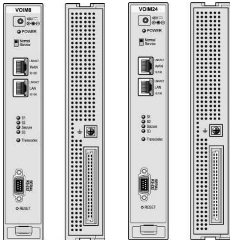
Figure 2.1.2-1 VOIM8 & 24 Front & Rear Panels
