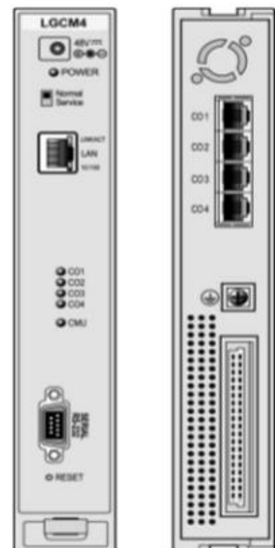
Figure 2.1.3.1-1 LGCM4 Front & Rear Panels
