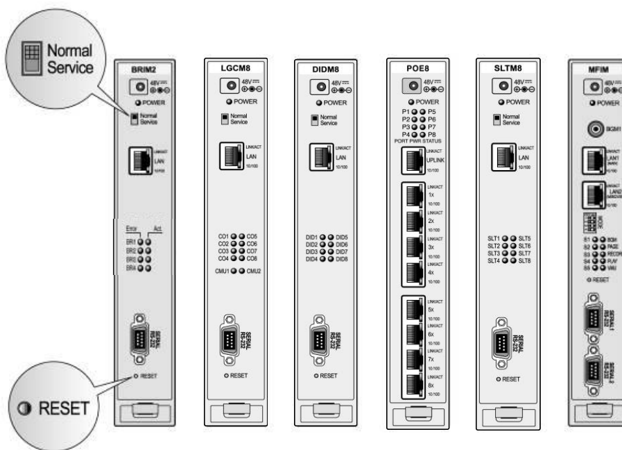
Figure 4.5.1.3-1 Common Module Switches
