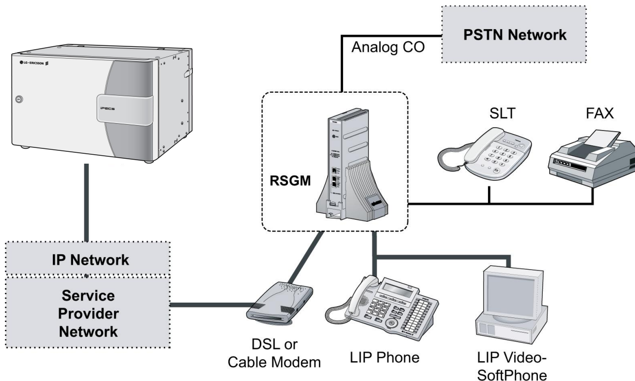
Figure 2.1.11-1 RSGM Connection
