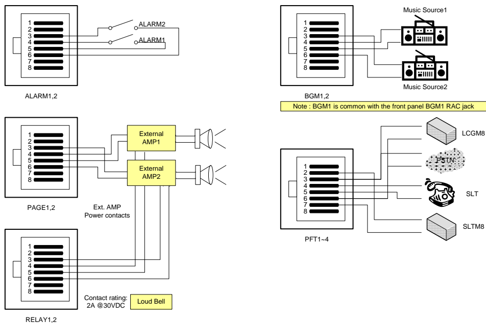
Figure 4.5.2-1 MFIM100 Miscellaneous Function Connections
