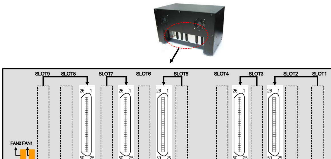
Figure 4.6-1 RJ-21x Connector Backplane Wiring Diagram
