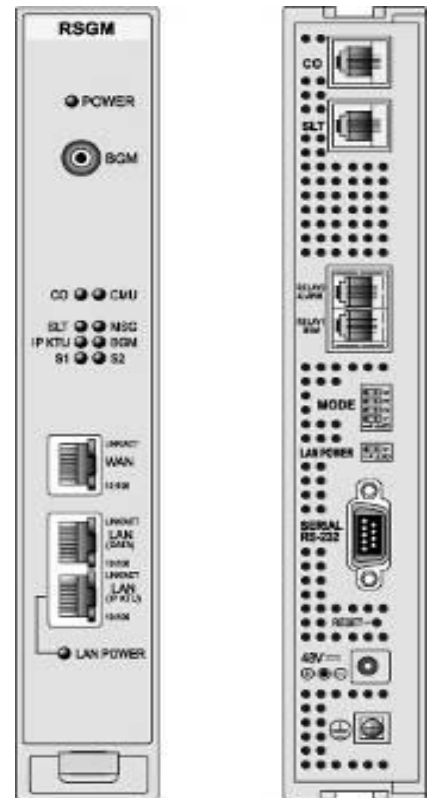
Figure 2.1.11-2 RSGM Front & Rear Panels
