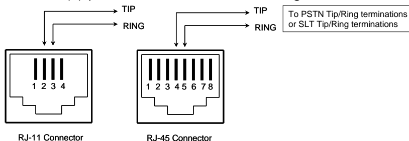
Figure 4.5.1.5-1 Telephony (RJ-11 or RJ-45) Connector Pin Assignment
