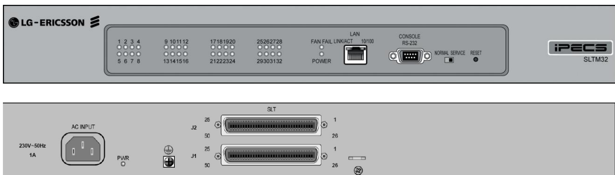
Figure 2.1.6.3-1 SLTM32 Front & Rear Panels
