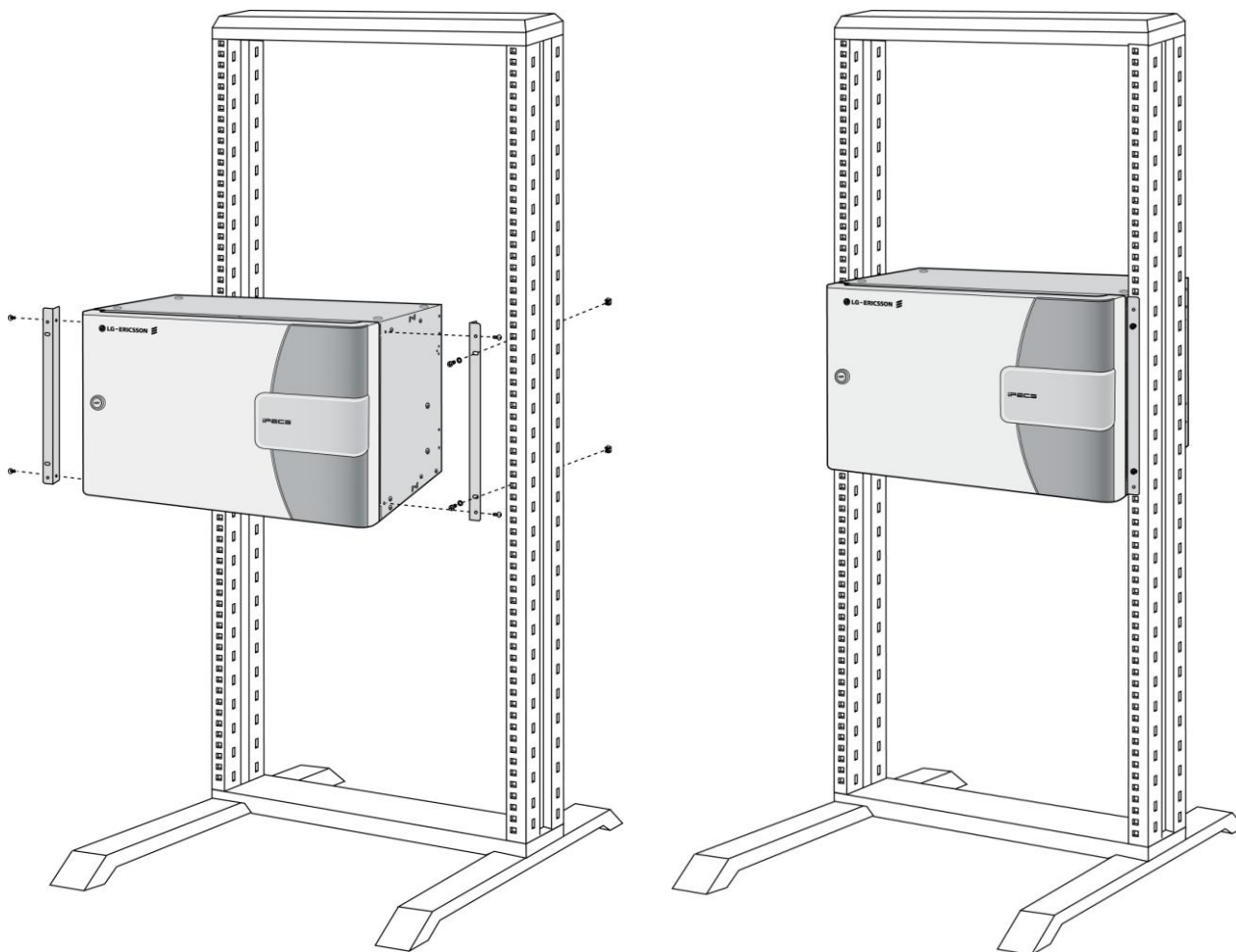
Figure 4.3.1.2-1 Rack (19”) Installation
