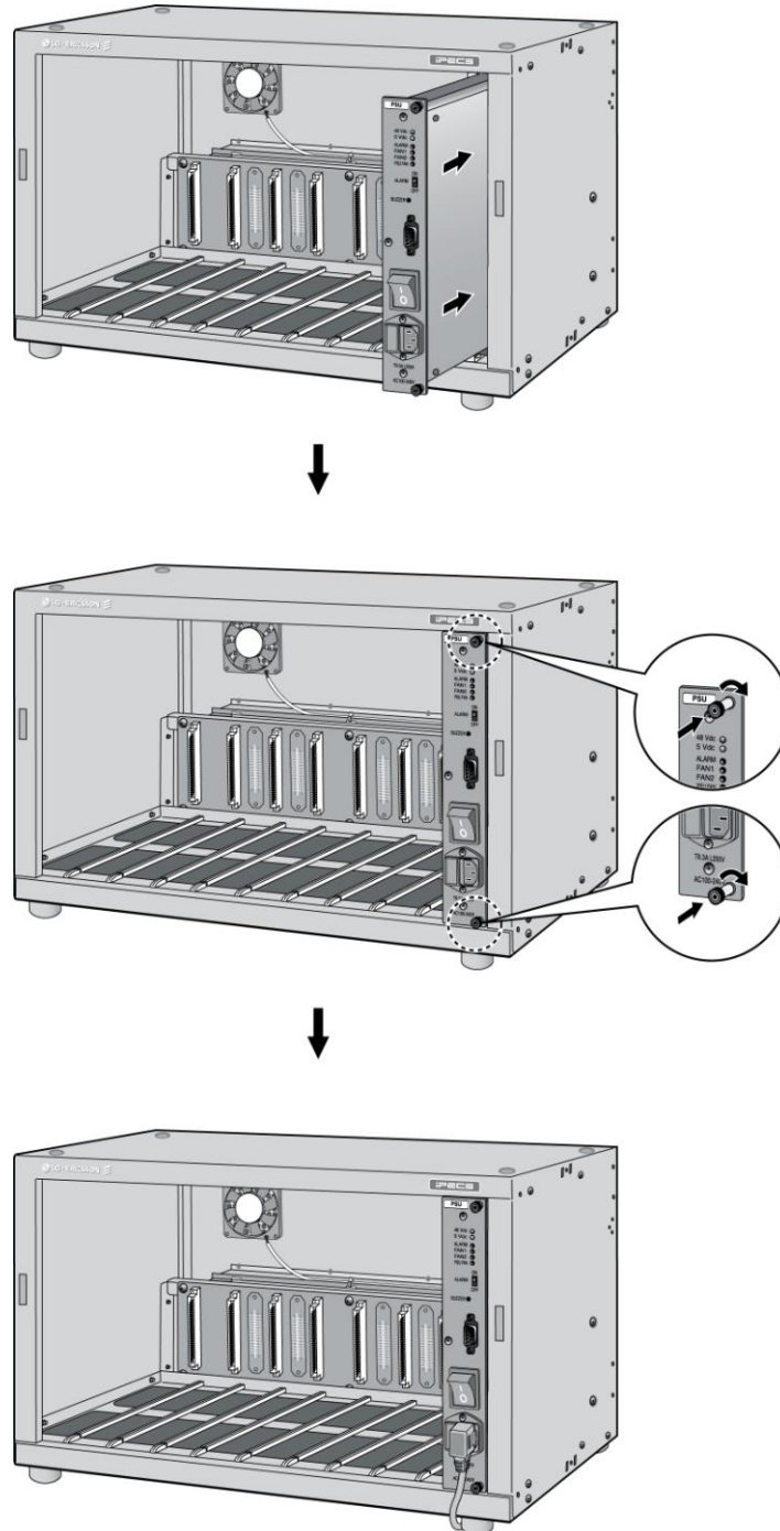
Figure 4.4-1 Main PSU Installation
