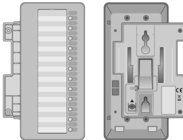
Figure 2.2.1-6 LIP-8012DSS
