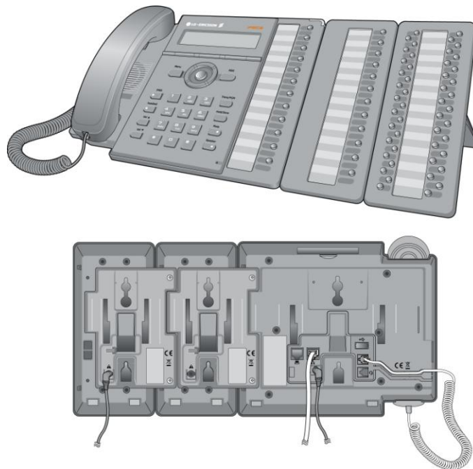
Figure 4.7-3 LIP-8000 DSS Installation (12DSS + 48DSS)
