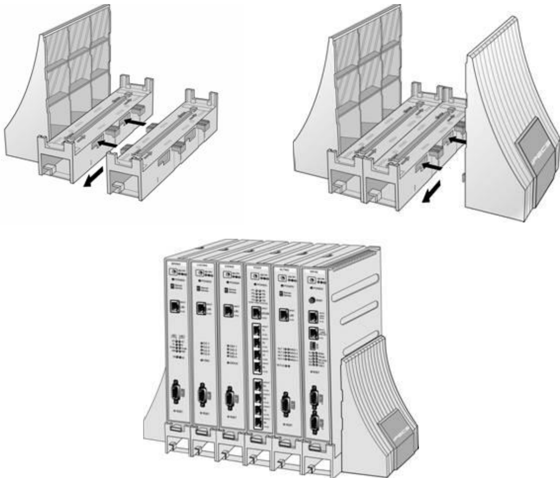
Figure 4.3.3-1 Module Desk Mount Holder Kit
