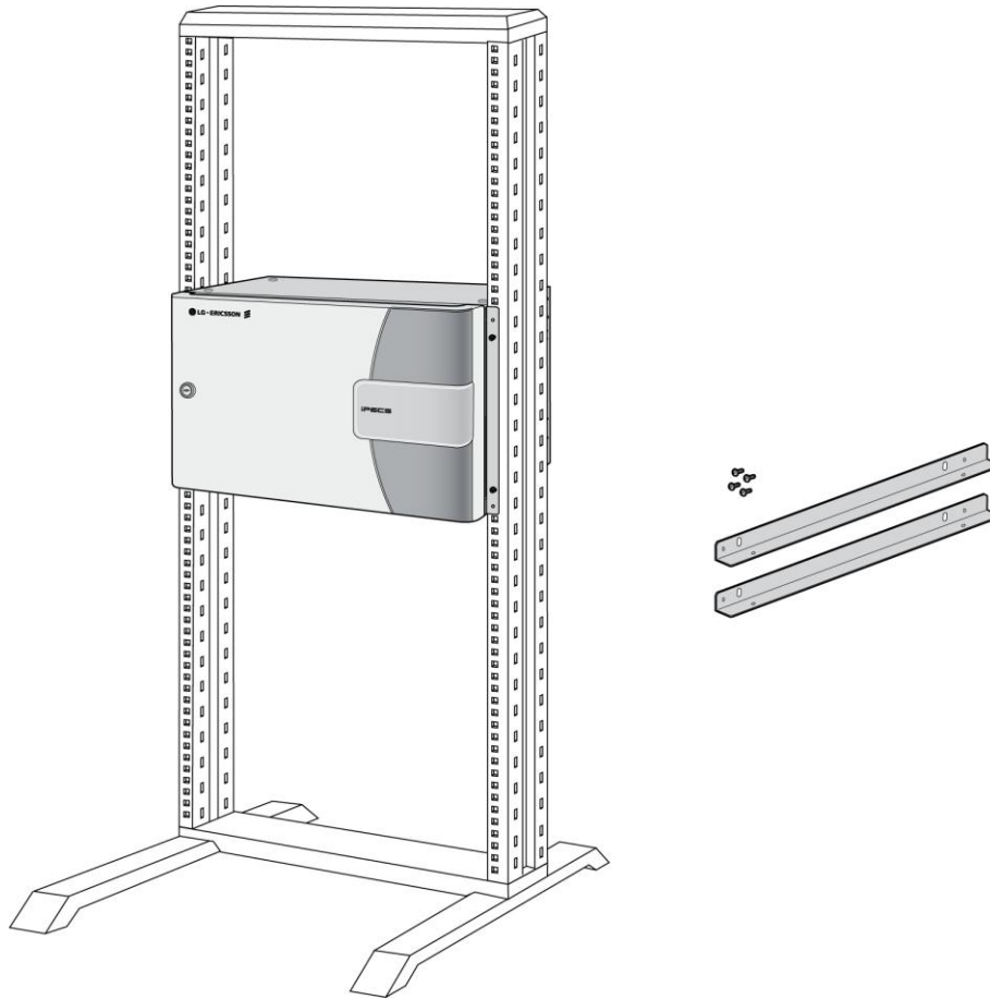
Figure 2.3.4-2 19" Rack Mount Installation
