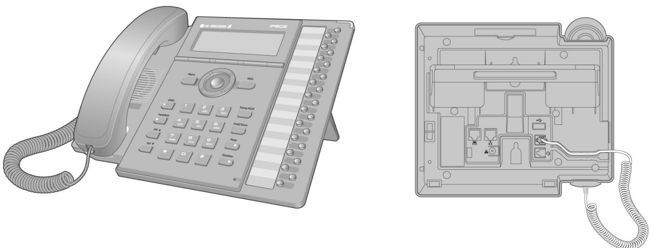
Figure 2.2.1-4 LIP-8024D
