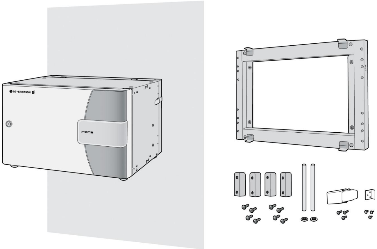
Figure 2.3.4-4 Wall Mount Installation
