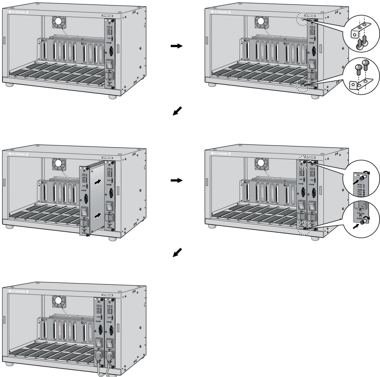
Figure 4.4-2 Back-up PSUs Installation
