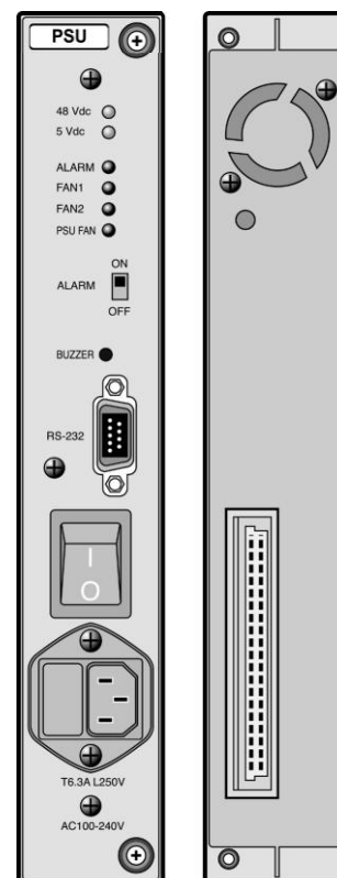
Figure 2.1.14-1 PSU Front & Rear Panels
