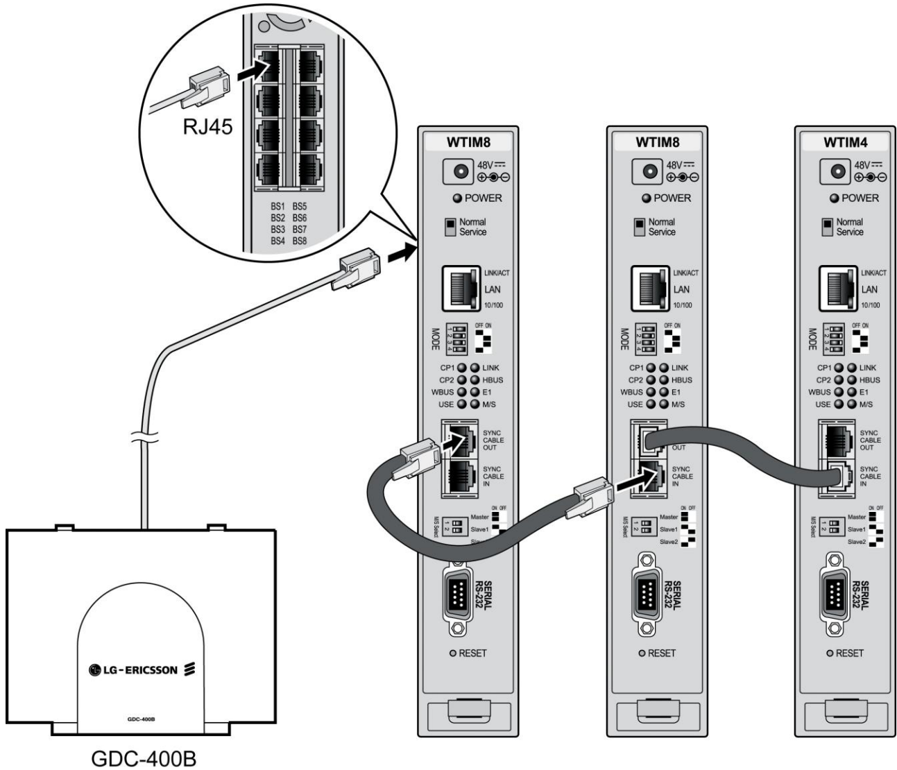
Figure 4.5.19-1 Cascading connections of WTIM4/8
