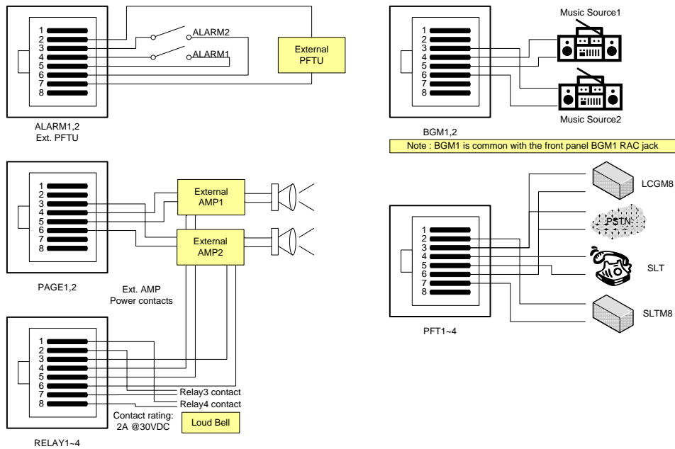
Figure 4.5.2-2 MFIM300/MFIM600/MFIM1200 Miscellaneous Function Connections
