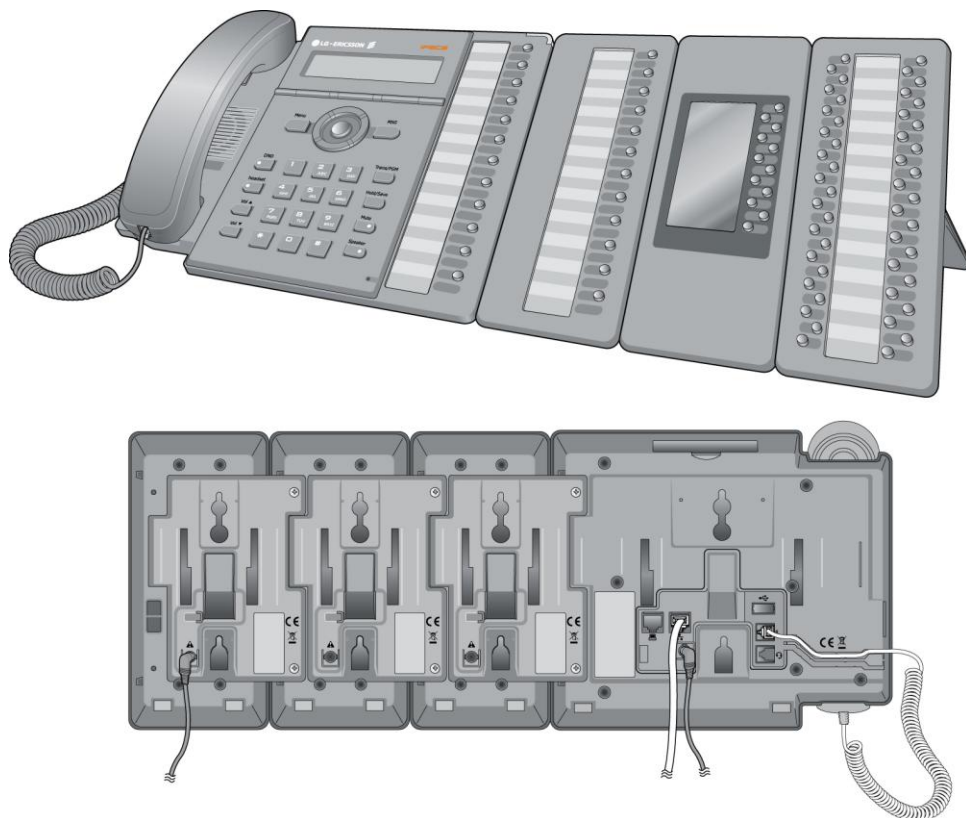
Figure 4.7-5 LIP-8000 DSS Installation (12DSS + 12LSS+48DSS)
