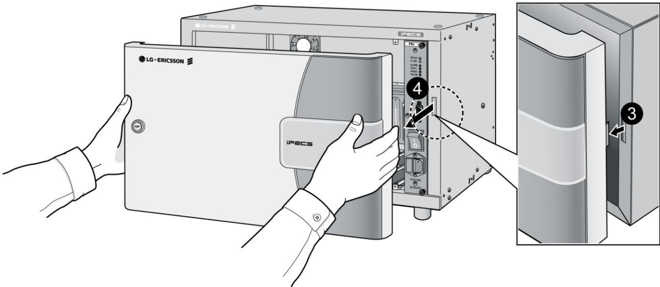
Figure 4.3.1.1-2 Cover removal
