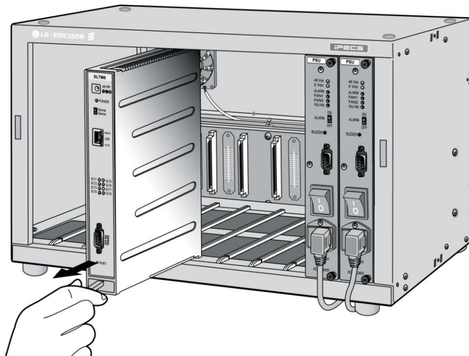
Figure 4.5.1.2-1 Module Insertion/Removal
