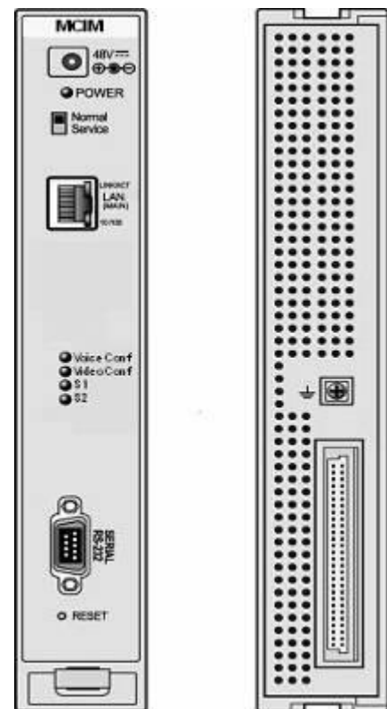
Figure 2.1.10-1 MCIM Front & Rear Panels
