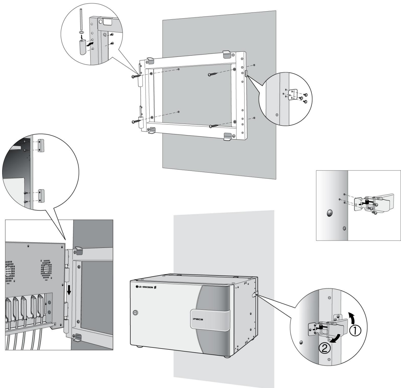
Figure 4.3.1.3-1 Cabinet Wall Mount Kit Installation
