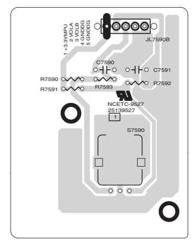
U22 VOLUME PC BOARD (NAETC-9527) Soldering side
