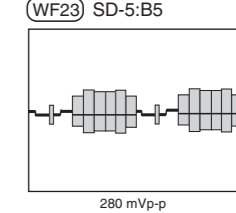
S-Video C waveform (WF23) SD-5:B5
