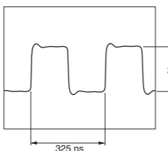
(WF08) CX_SLCK (SD-7:E4)
