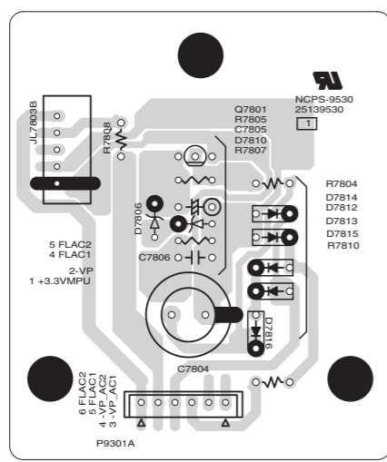
U25 POWER SUPPLY PC BOARD (NAPS-9530) Soldering side
