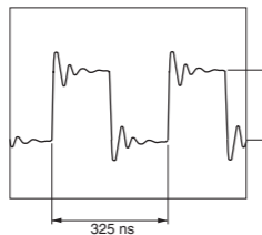
(WF05) SAI_SLCK (SD-7:D5)
