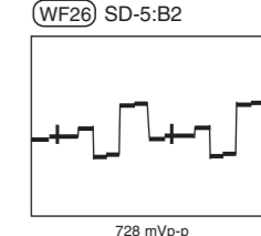
Component PR waveform (WF26) SD-5:B2
