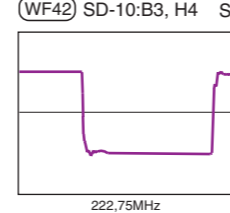
HDMI CK waveform (WF42) SD-10:B3, H4 SD-11:B5
