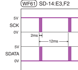
SCK/SDATA waveform (WF61) SD-14:E3,F2
