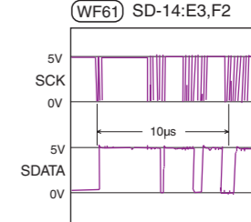
SDATA waveform varies according to the data content
