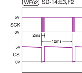
SCK/RESET waveform (WF63) SD-14:E3,F2
