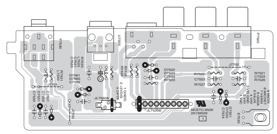
U24 TERMINAL PC BOARD (NAETC-9529) Soldering side
