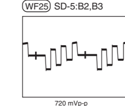
Component PB waveform (WF25) SD-5:B2,B3
