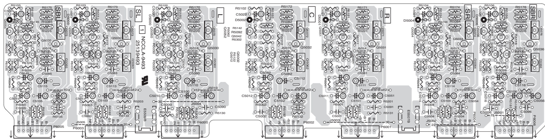
U13 AMPLIFIER PC BOARD (NACLA-9493)
