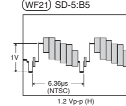
Composite waveform (WF21) SD-5:B5
