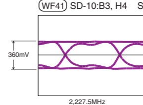
HDMI D0,D1,D2 waveform (WF41) SD-10:B3, H4 SD-11:B5
