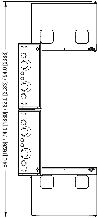
TOP VIEW (2 DWR's fully opened)
