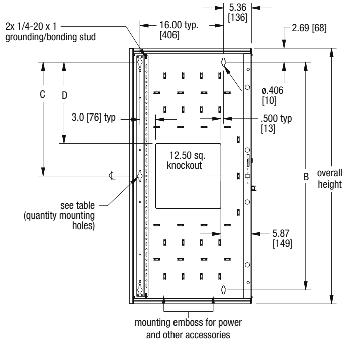
FRONT VIEW (BACK PAN)
