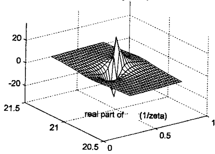
1/zeta near .5 + i21.022
