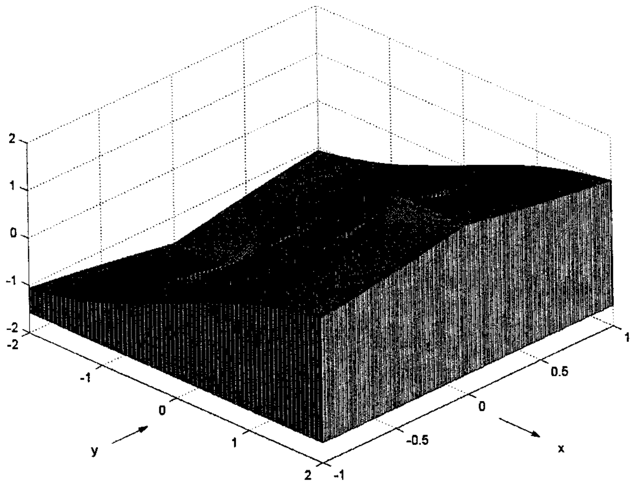
problem 20(c) sec. 3.7 real part
