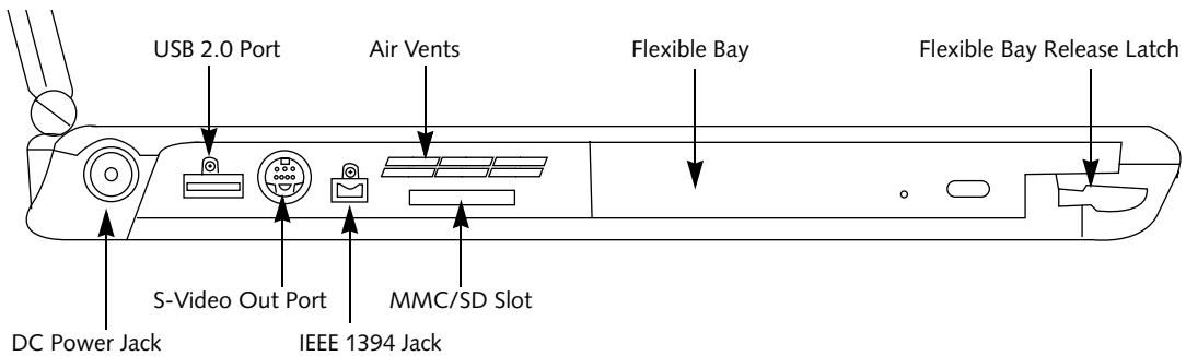
Figure 2-5. LifeBook notebook left-side panel
