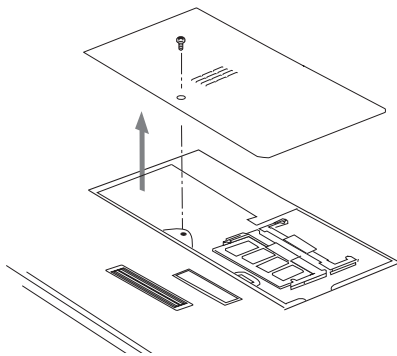
Figure 4-7. Opening the Memory Upgrade Compartment
