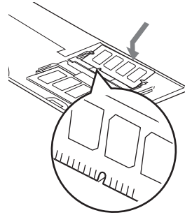
Figure 4-8. Installing a Second Memory Module
