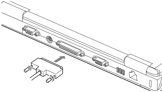
Figure 4-17. Connecting a Parallel Device
