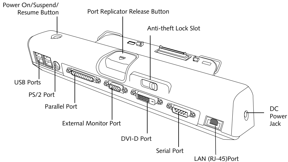
Figure 4-10. Port Replicator back panel
