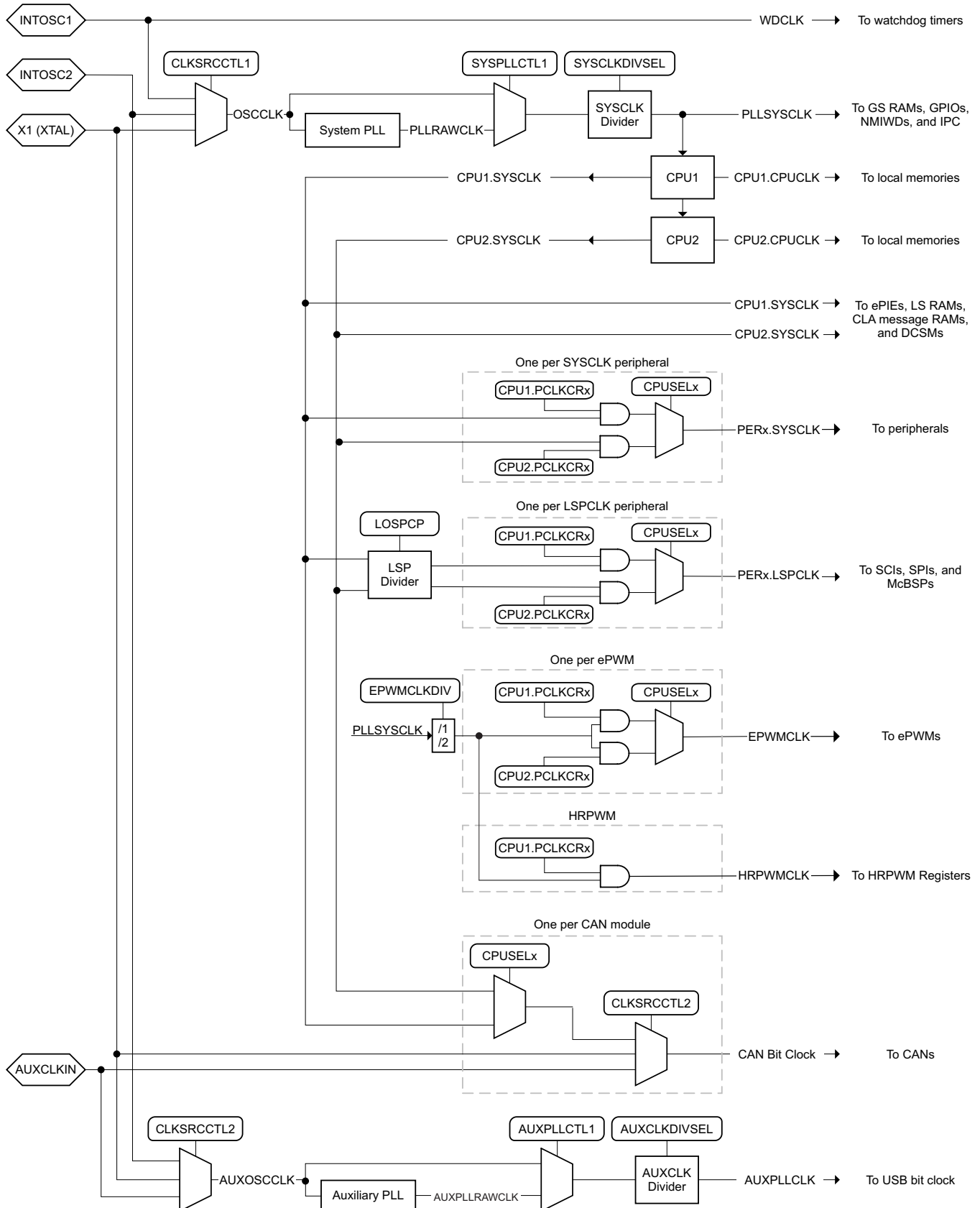
Figure 2-5. Clocking System
