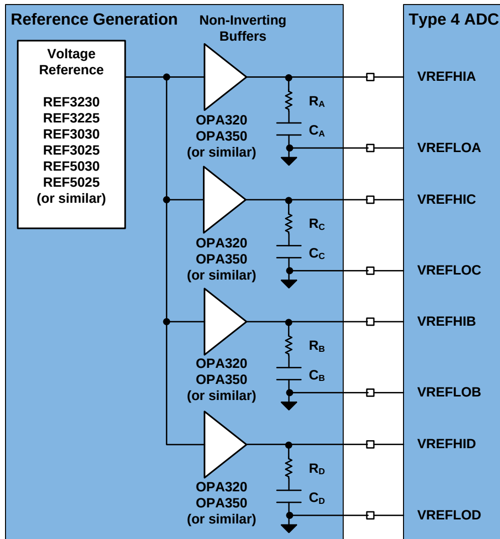
Figure 10-23. ADC Reference System
