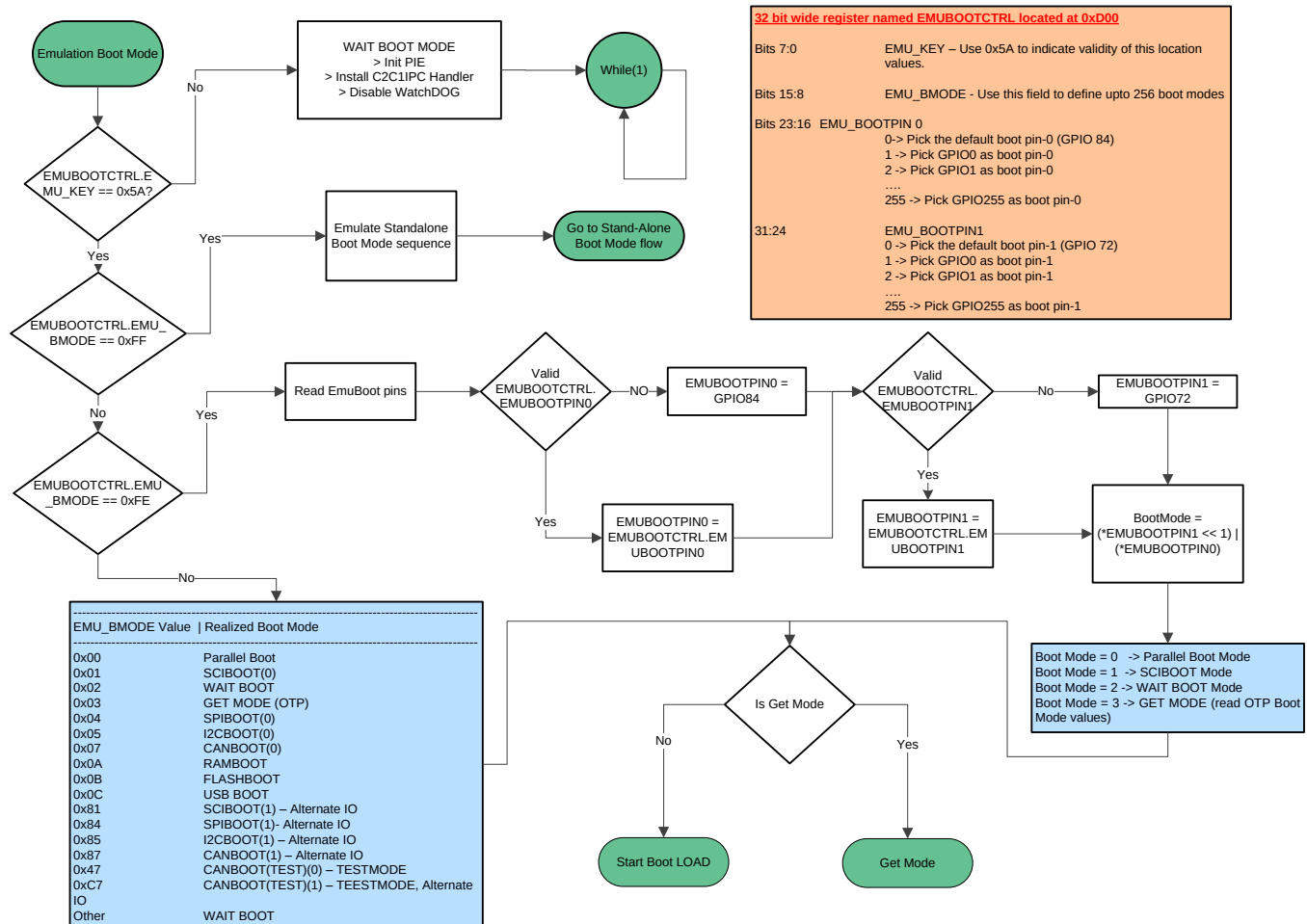
Figure 3-4. CPU1 Emulation Boot Flow
