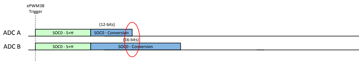
Figure 10-20. Example: Asynchronous Operation with Different Resolutions
