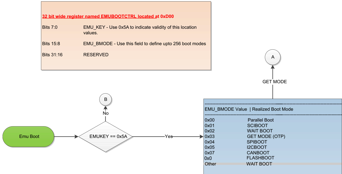
Figure 3-7. CPU2 Standalone and Hibernate Boot Flow
