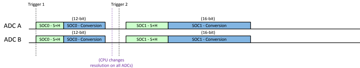
Figure 10-21. Example: Synchronous Operation with Different Resolutions
