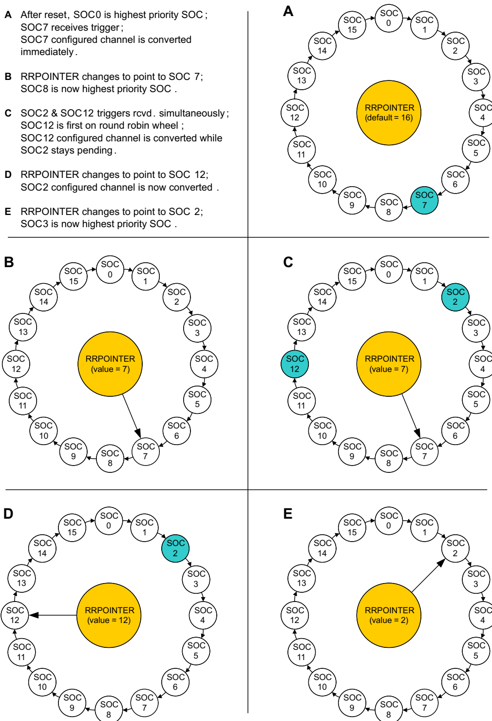
Figure 10-5. Round Robin Priority Example
