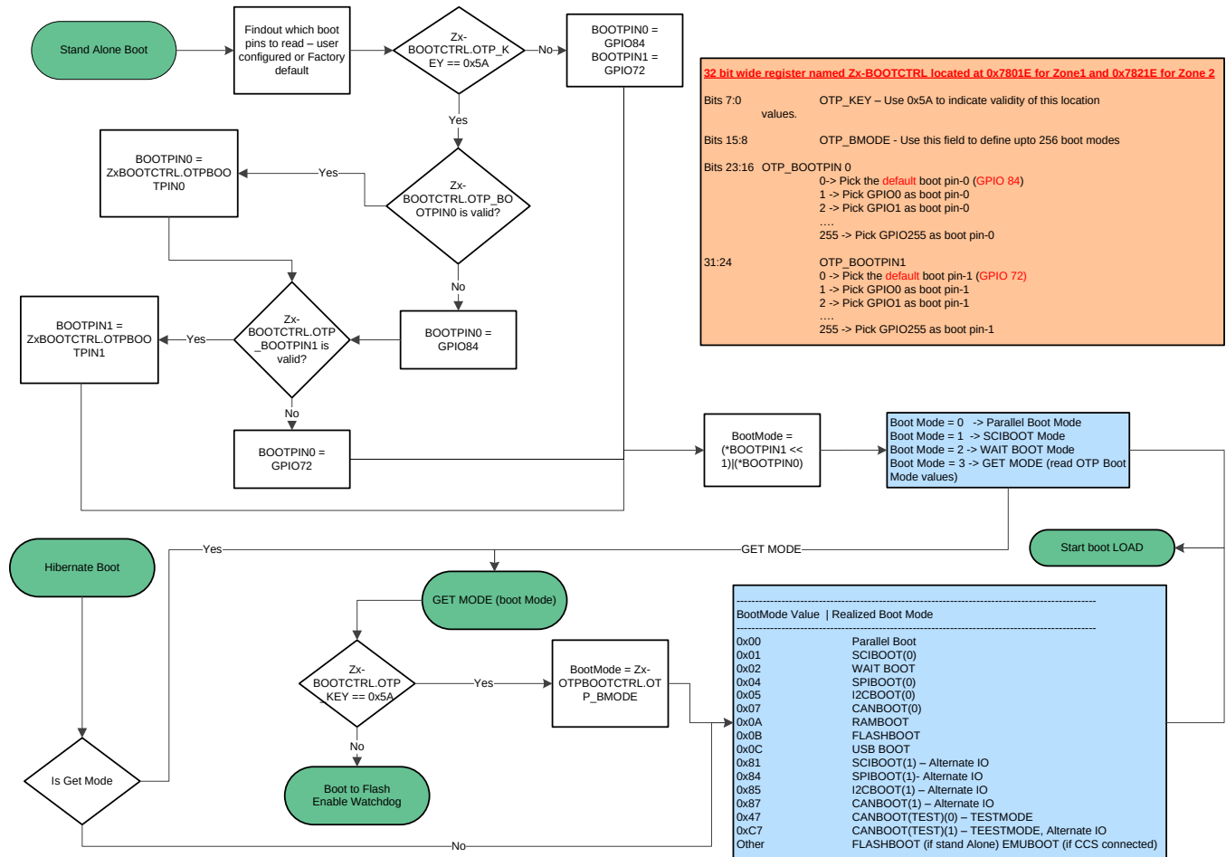
Figure 3-6. CPU1 Standalone and Hibernate Boot Flow
