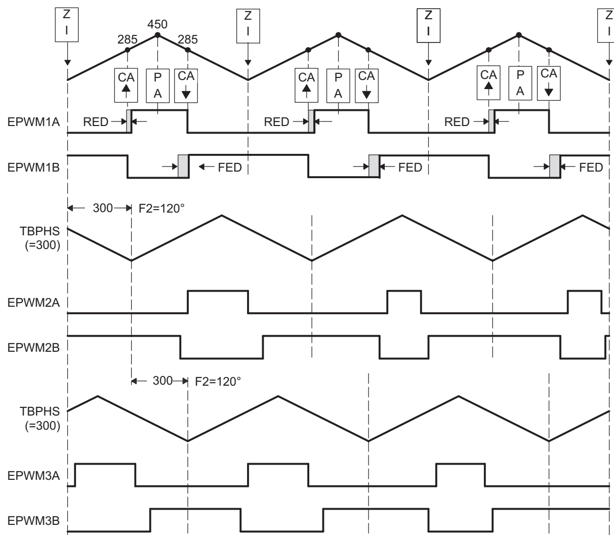
Figure 14-70. 3-Phase Interleaved DC/DC Converter Waveforms for Figure 14-69
