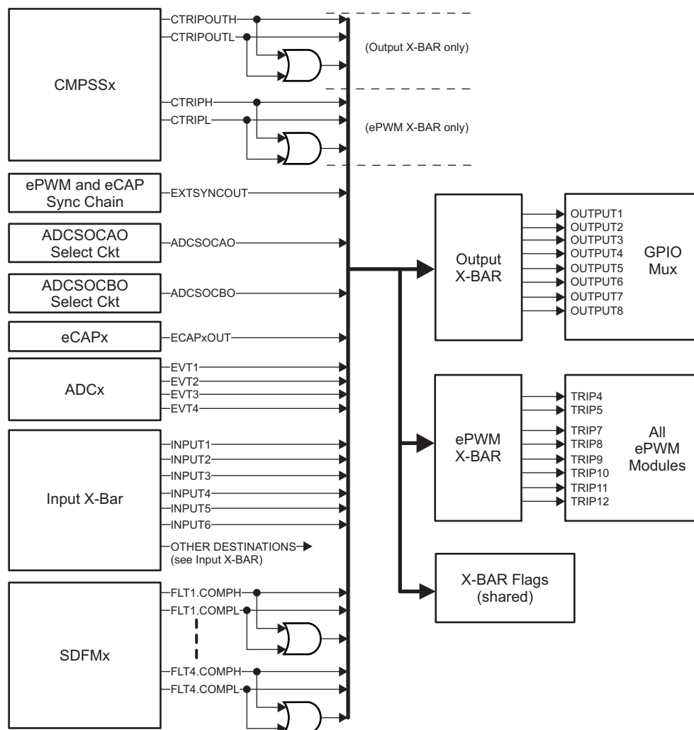
Figure 14-57. EPWM X-BAR
