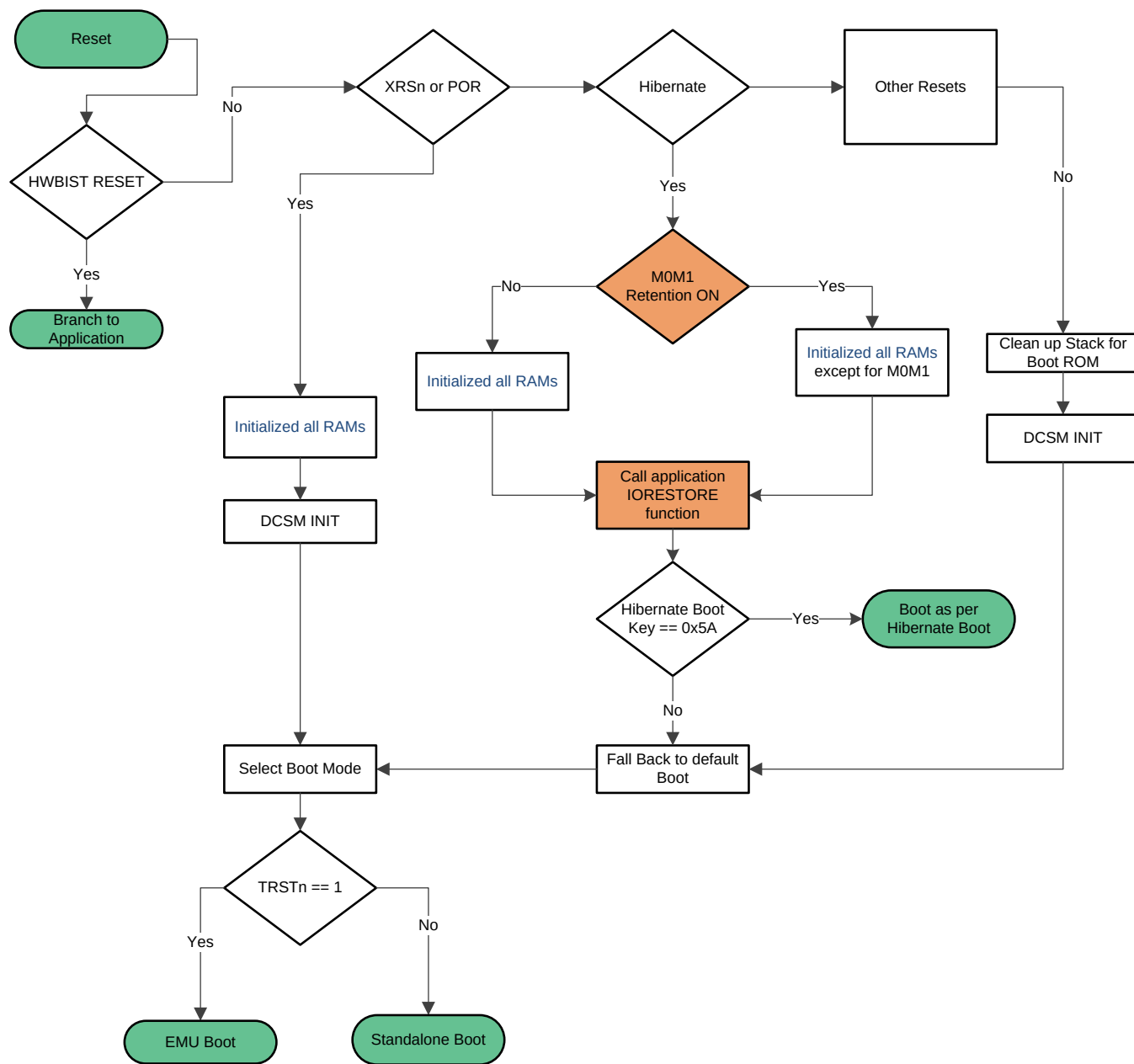
Figure 3-3. CPU2 Device Boot Flow
