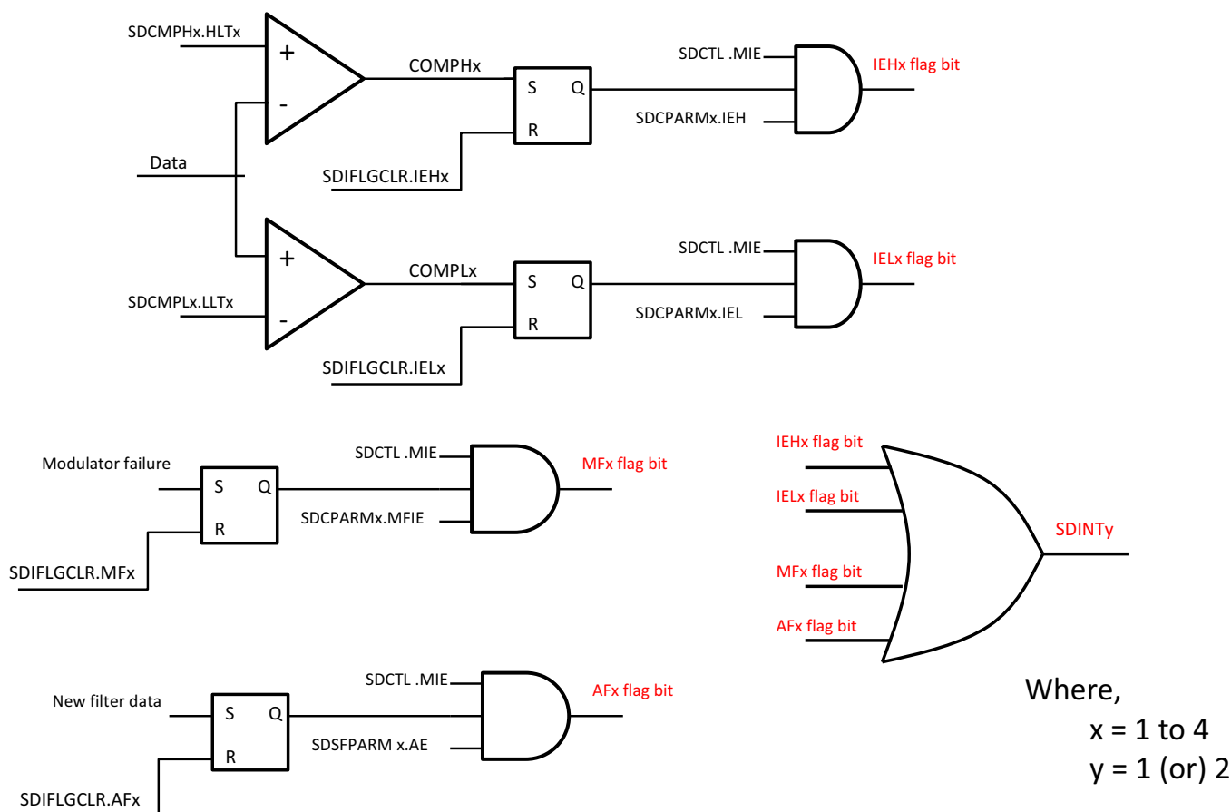
Figure 13-9. SDFM Interrupt Unit
