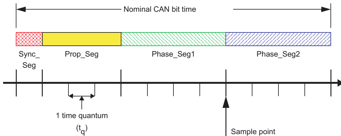
Figure 22-10. Bit Timing
