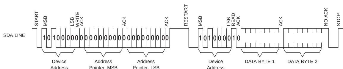
Figure 3-14. Random Read
