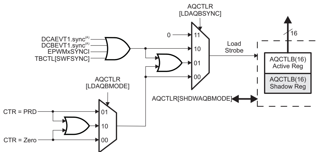
Figure 14-23. AQCTLR[SHDWAQBMODE]
