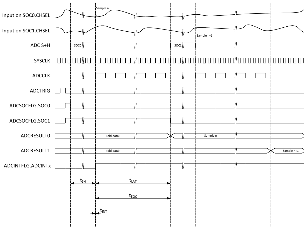
Figure 10-14. ADC Timings for 16-bit Mode in Early Interrupt Mode
