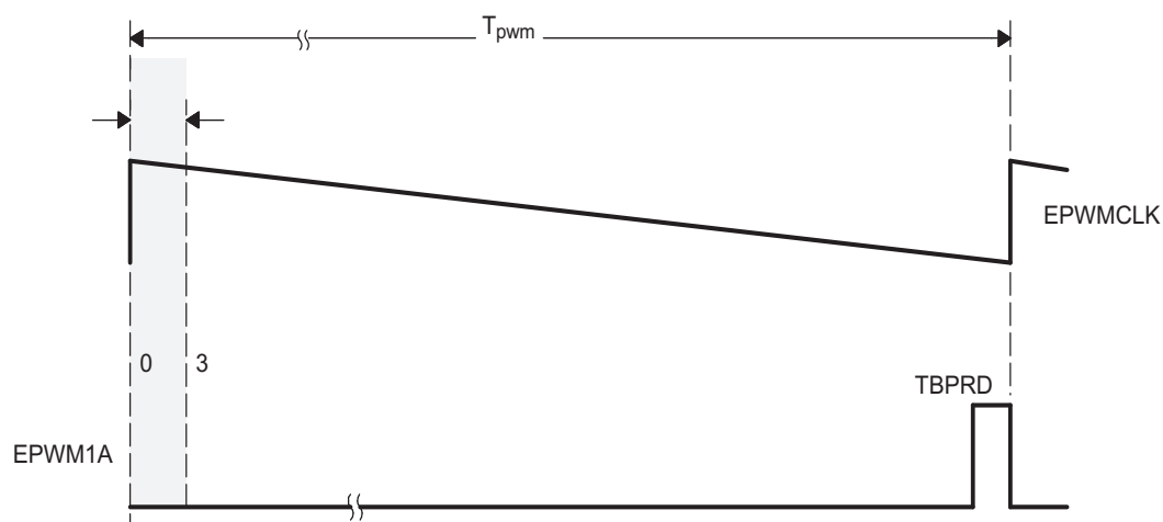
Figure 15-8. High % Duty Cycle Range Limitation Example (HRPCTL[HRPE] = 0)
