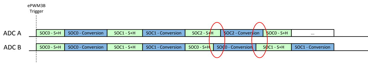
Figure 10-19. Example: Asynchronous Operation with Uneven SOC Numbers – Trigger Overflow
