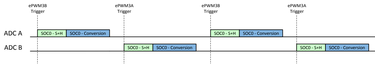
Figure 10-22. Example: Synchronous Equivalent Operation with Non-Overlapping Conversions
