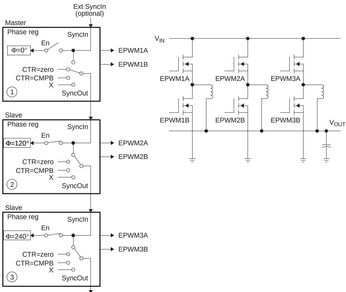
Figure 14-69. Control of a 3-Phase Interleaved DC/DC Converter
