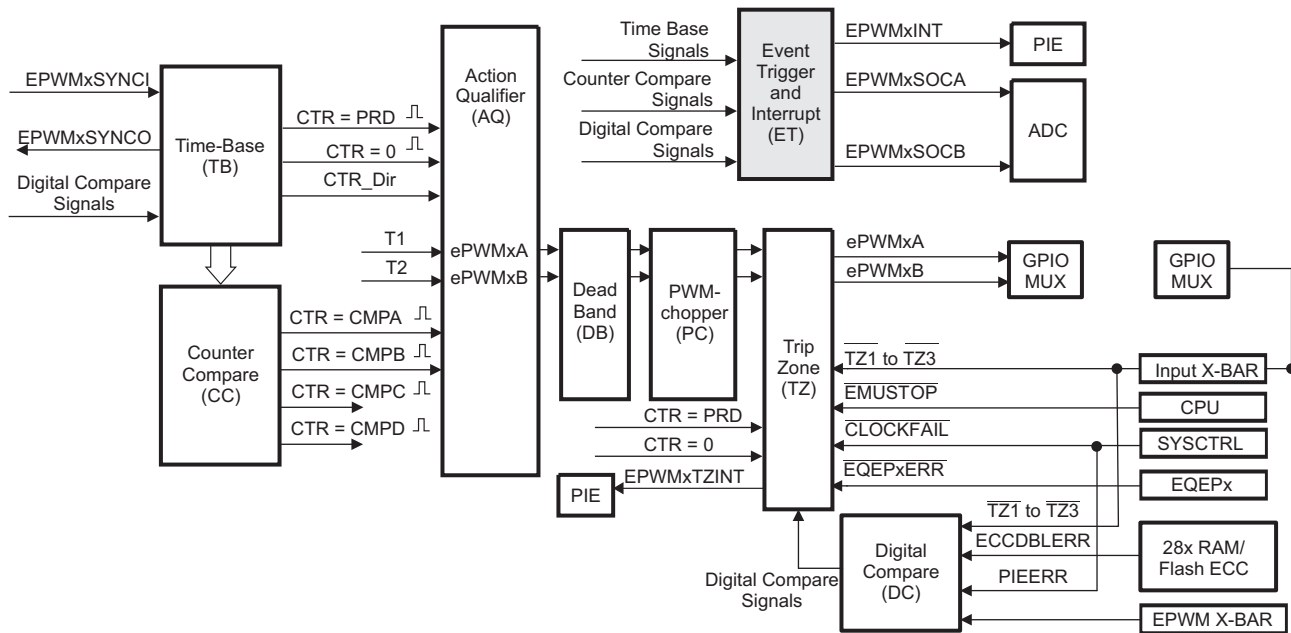
Figure 14-43. Event-Trigger Submodule
