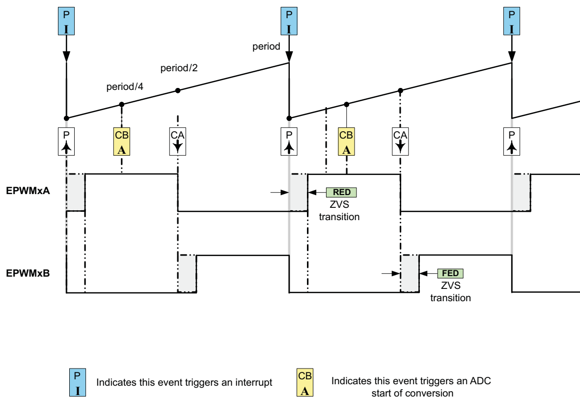
Figure 14-76. H-Bridge LLC Resonant Converter PWM Waveforms
