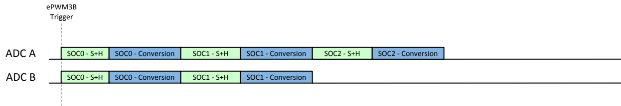
Figure 10-18. Example: Synchronous Operation with Uneven SOC Numbers
