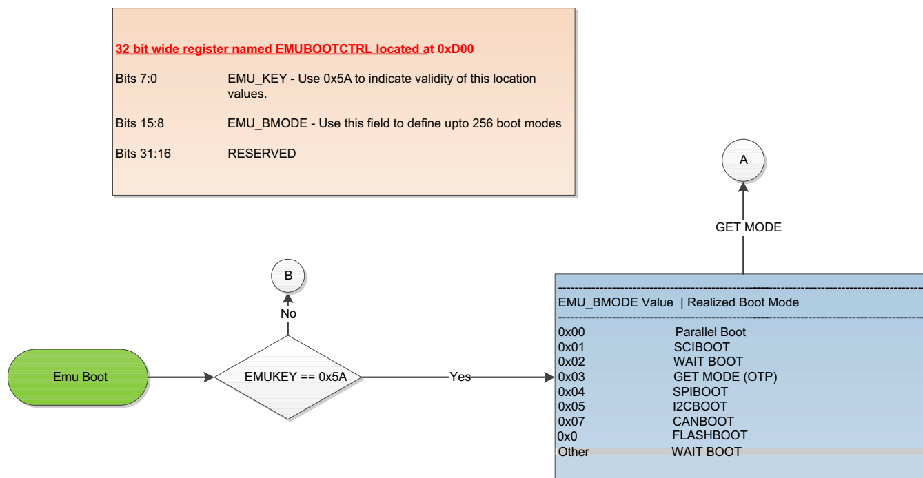
Figure 3-5. CPU2 Emulation Boot Flow
