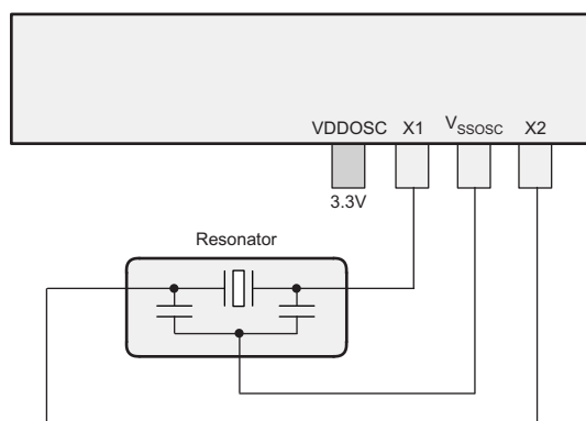
Figure 2-8. External Resonator
