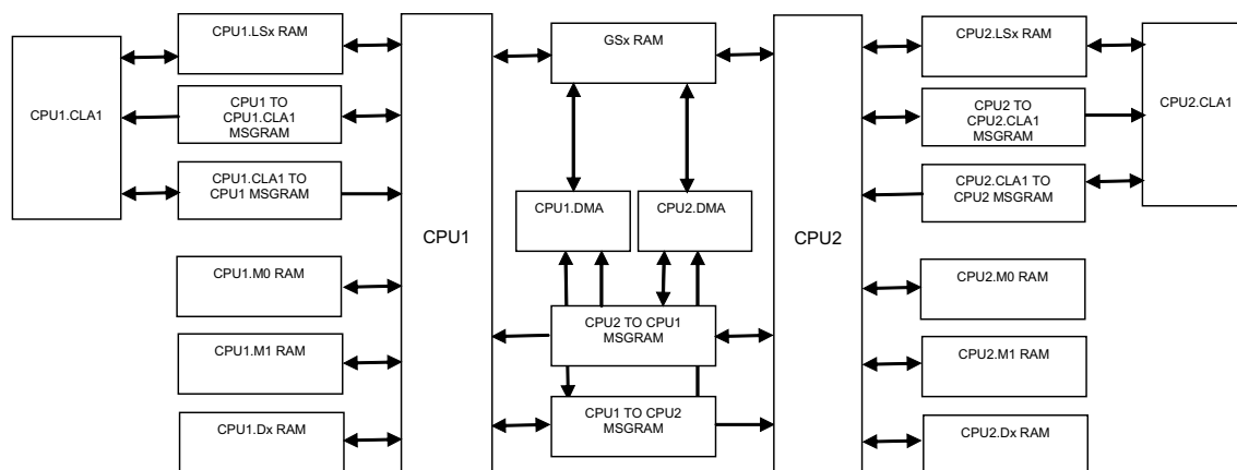
Figure 2-13. Memory Architecture
