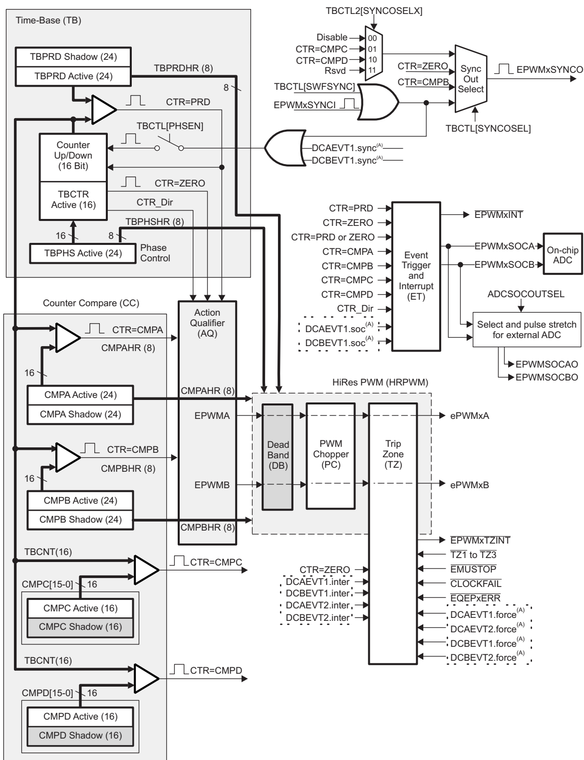
Figure 14-3. ePWM Submodules and Critical Internal Signal Interconnects
