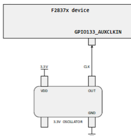
Figure 2-9. AUXCLKIN
