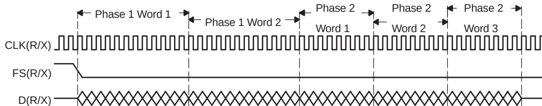
Figure 21-10. Dual-Phase Frame for a McBSP Data Transfer
