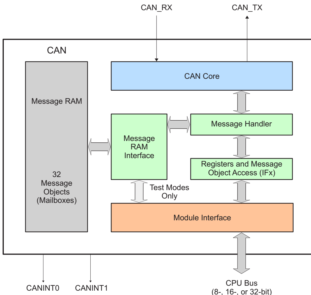
Figure 22-1. CAN Block Diagram
