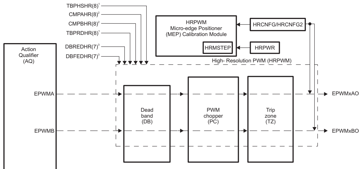
Figure 15-5. HRPWM Block Diagram
