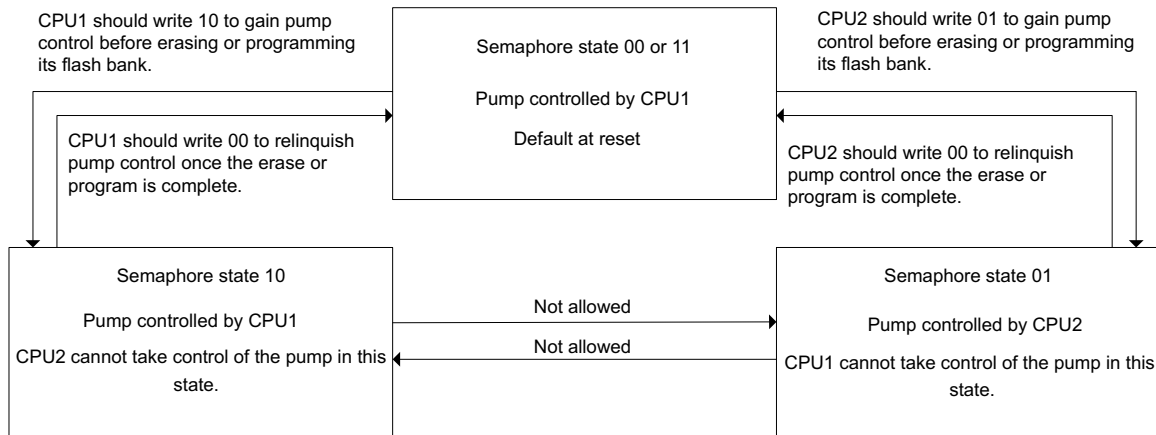
Figure 2-19. Flash Pump Semaphore (PUMPREQUEST) States and State Transitions
