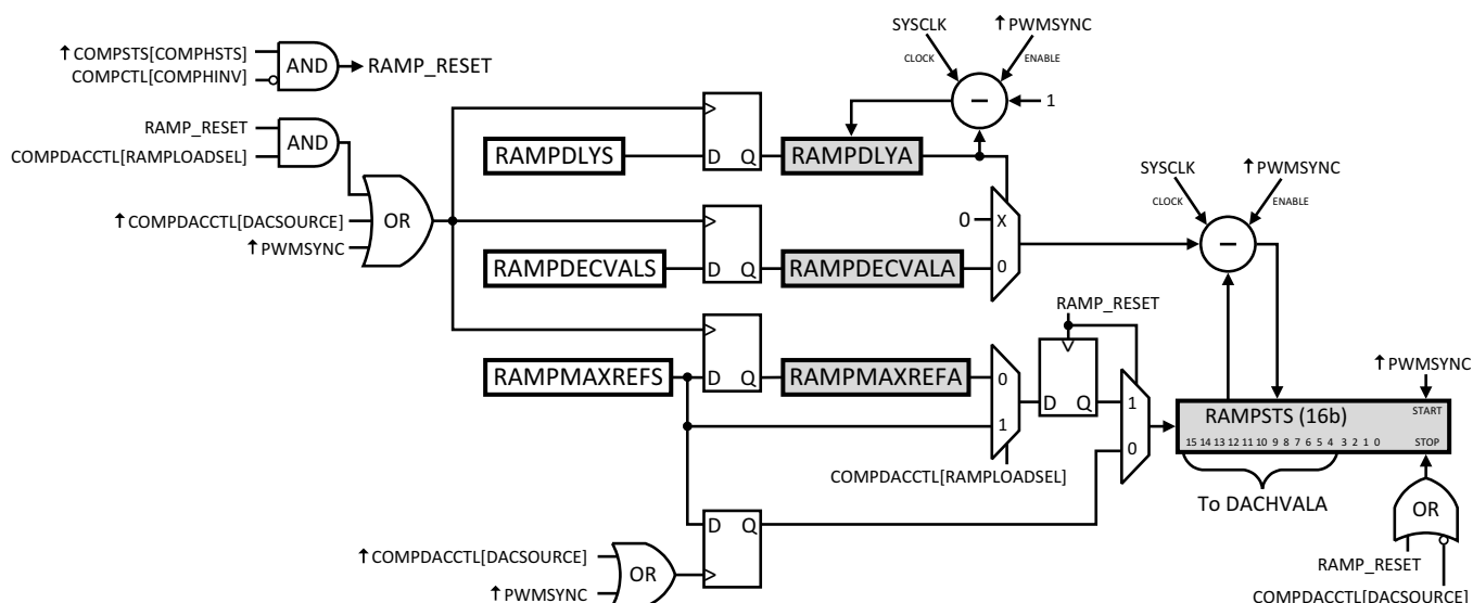
Figure 12-5. Ramp Generator
