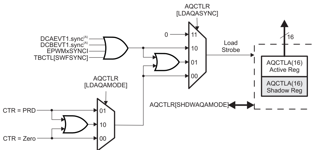
Figure 14-22. AQCTLR[SHDWAQAMODE]
