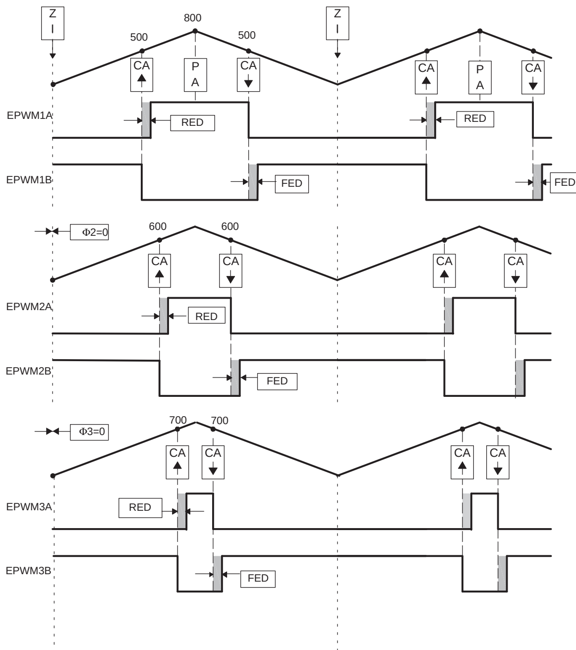
Figure 14-66. 3-Phase Inverter Waveforms (Only One Inverter Shown)
