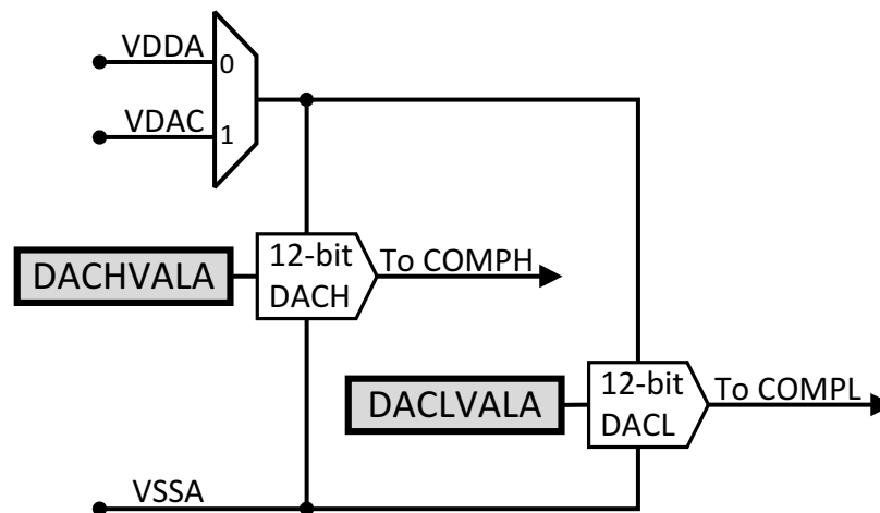
Figure 12-3. DAC Reference Select
