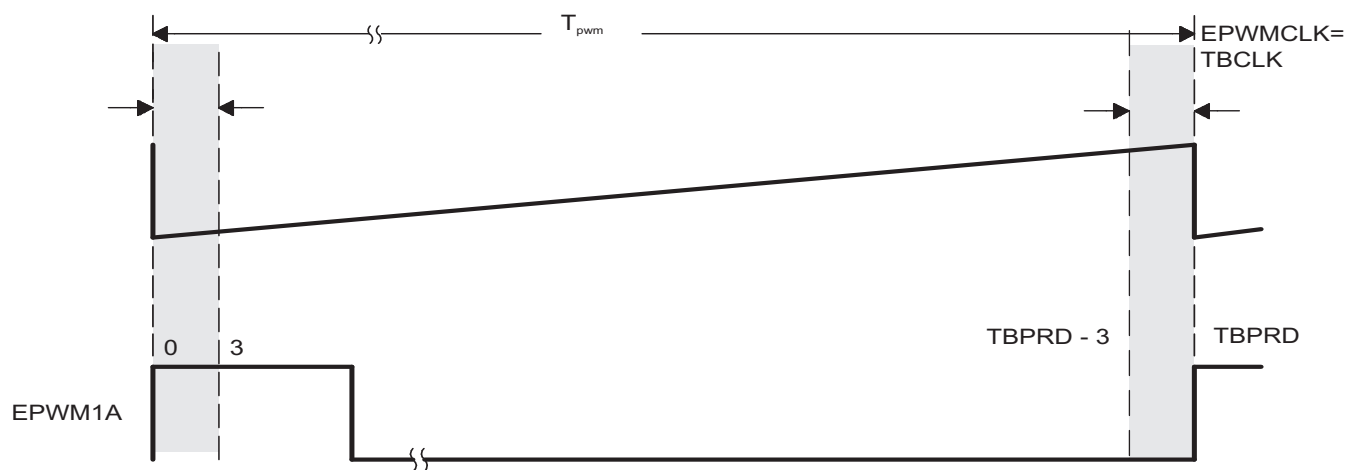
Figure 15-9. Up-Count Duty Cycle Range Limitation Example (HRPCTL[HRPE]=1)
