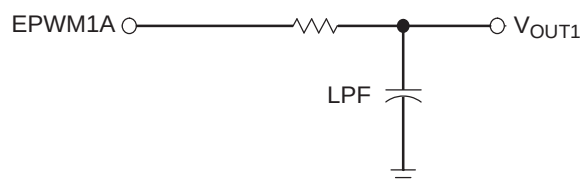
Figure 15-13. Simple Reconstruction Filter for a PWM-based DAC
