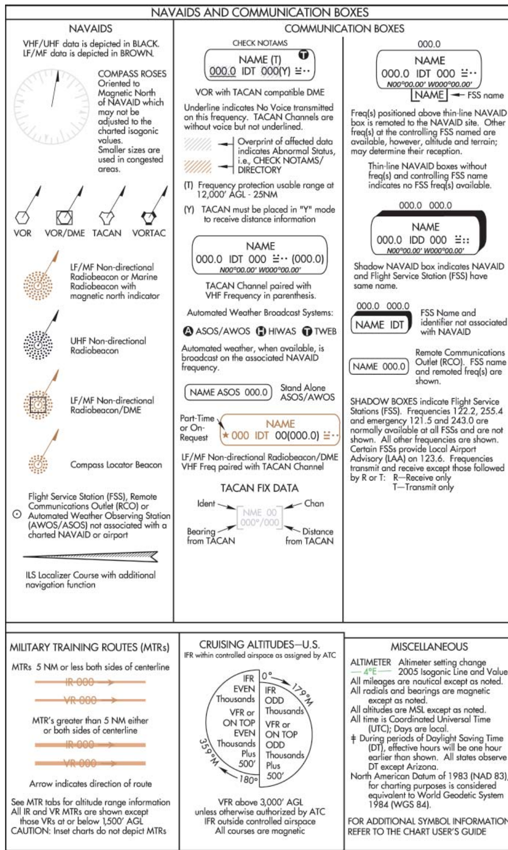
Figure 8-5. Legend From En Route Low Attitude Chart.
