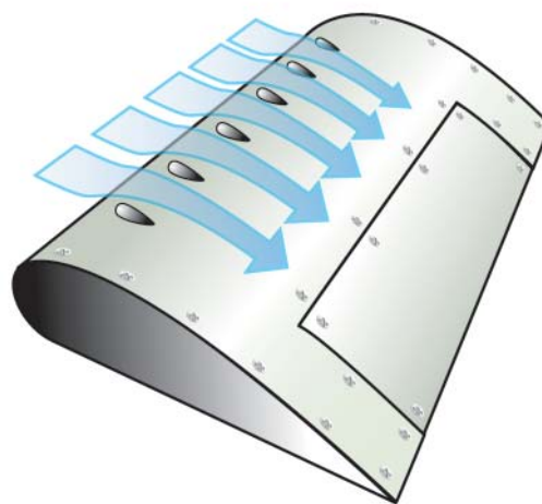
Controlled Vortices
