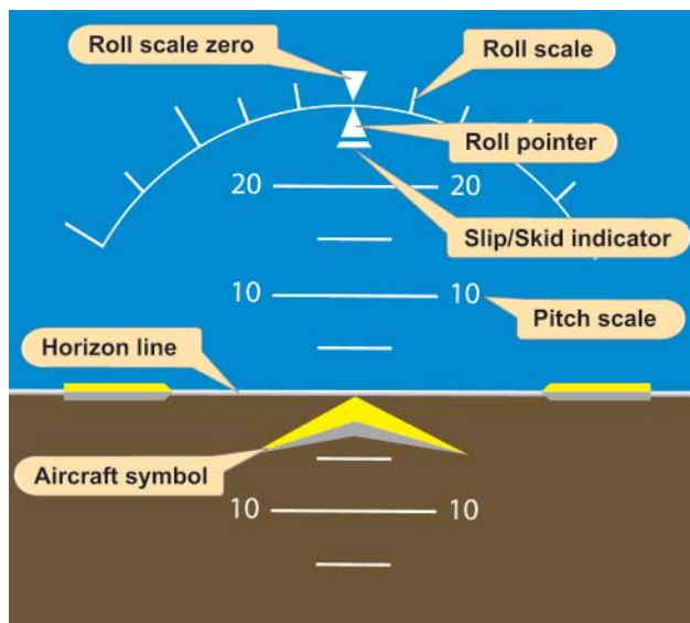
Figure 5-52. Attitude Indicator.
