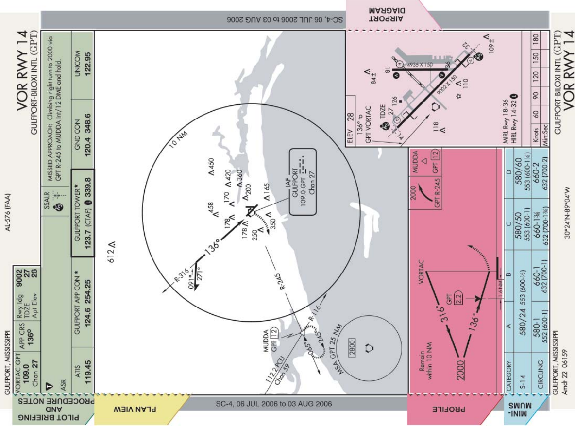
Figure 8-16. More IAP Profile View Features.
