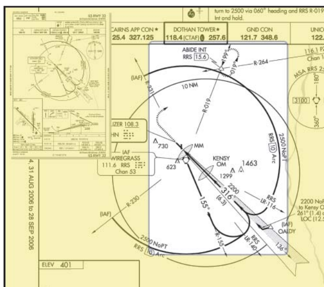
Figure 8-15. Teardrop Procedure.
