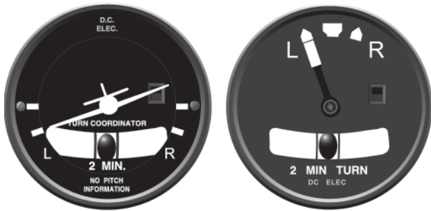
Figure 4-12. Turn Coordinator and Turn-and-Slip Indicator.
