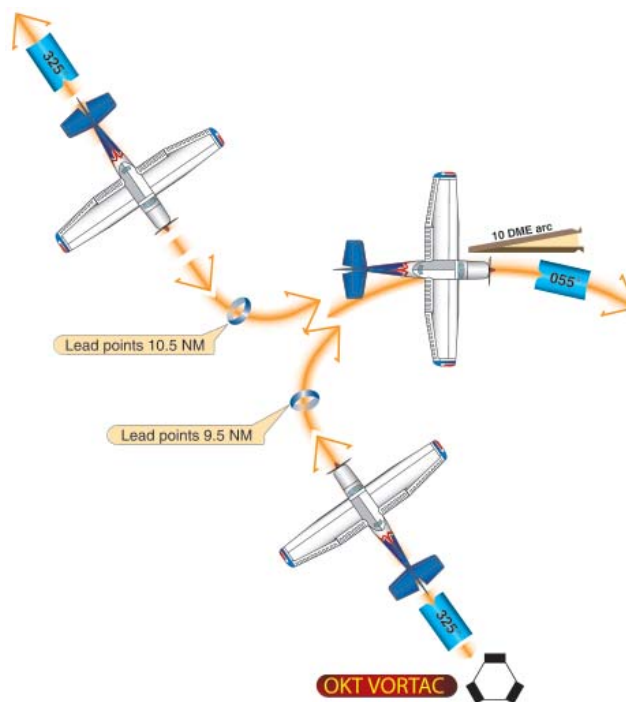
Figure 7-17. DME Arc Interception.
