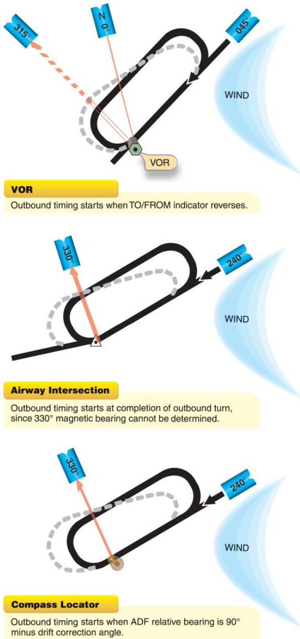
Figure 10-7. Holding—Outbound Timing.
