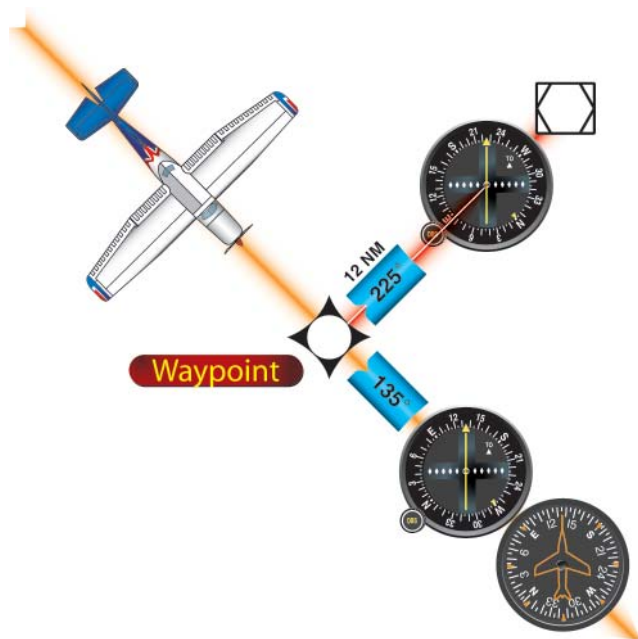
Figure 7-25. Aircraft/DME/Waypoint Relationship.
