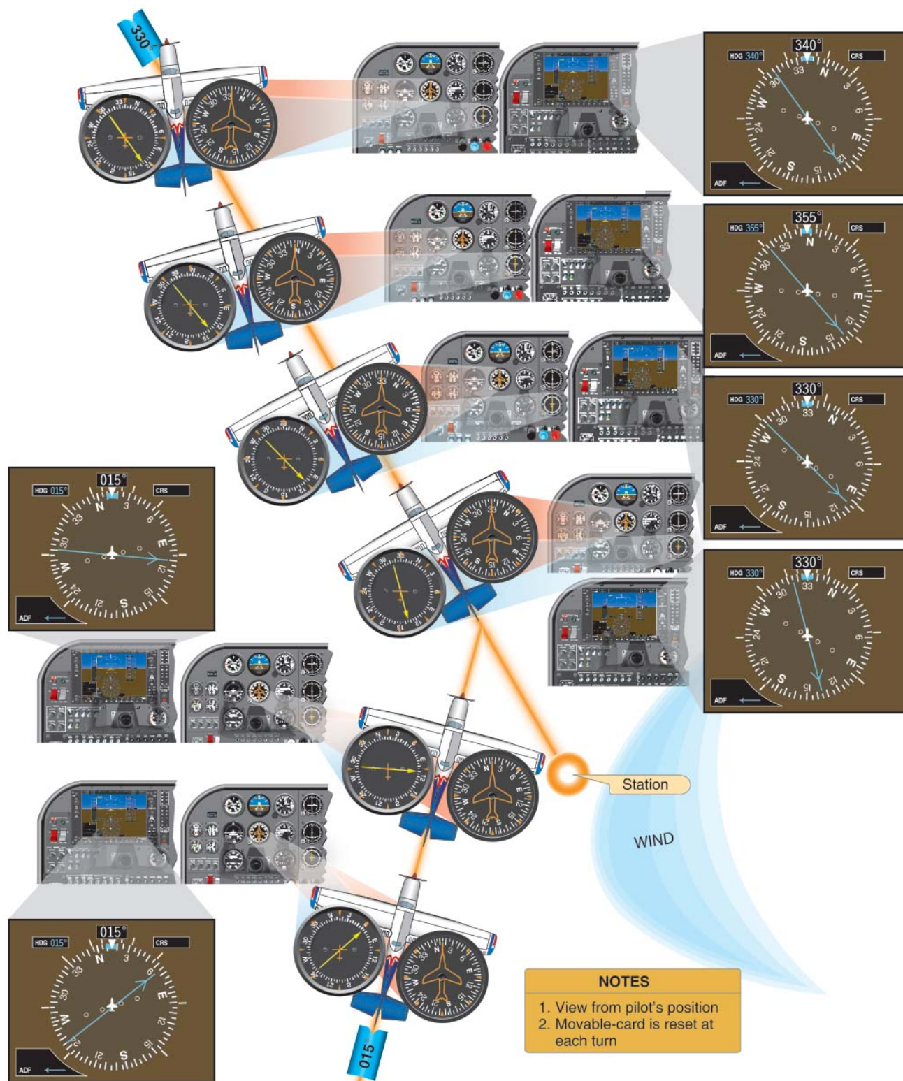
Figure 7-8. ADF Interception and Tracking Outbound.
