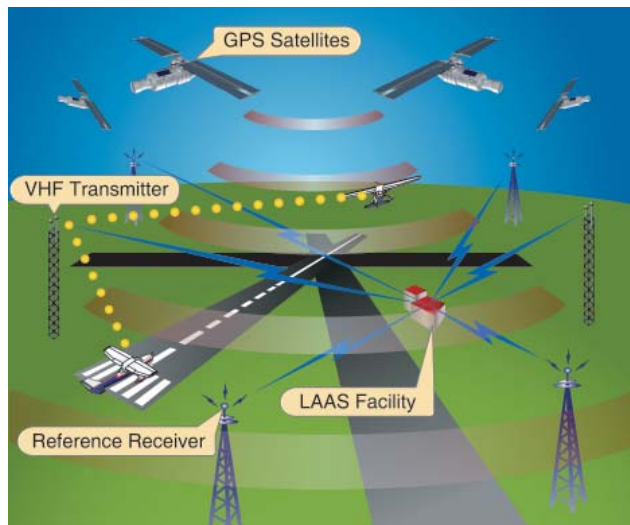
Figure 7-33. LAAS Representation.
