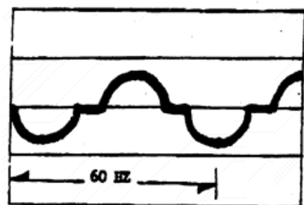
Figure 5-6 Harmonic Imbalance
