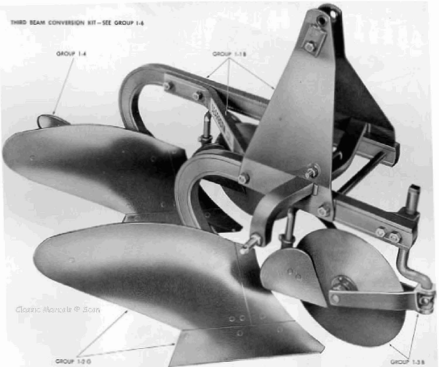
Figure 2 - Dearborn Economy Plow, Double Bottom
