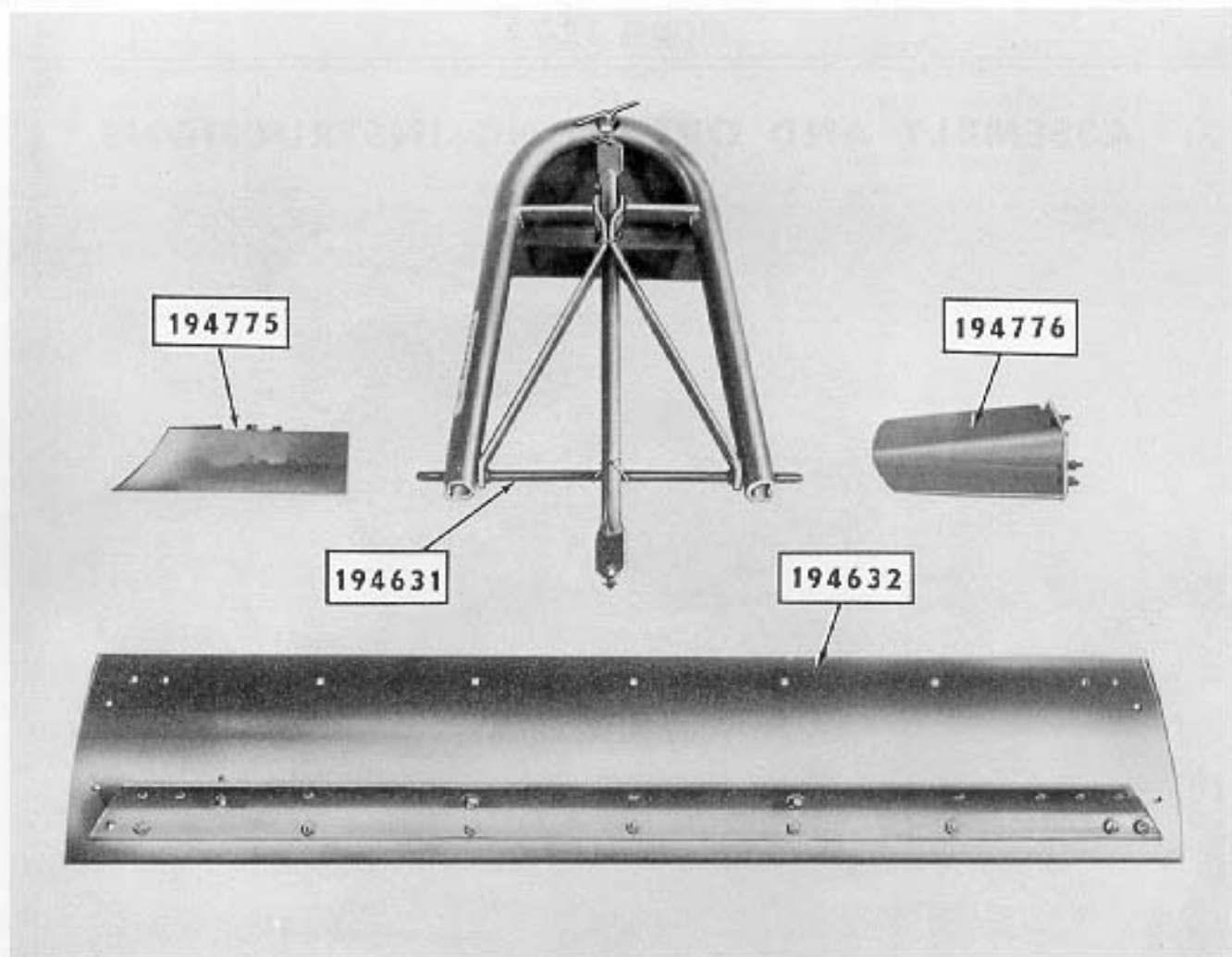
Figure 1 Dearborn Economy Blade Bundled for Shipment
