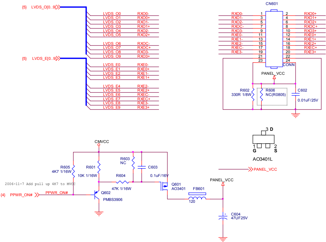
LVDS Panel ( Normal Type )
