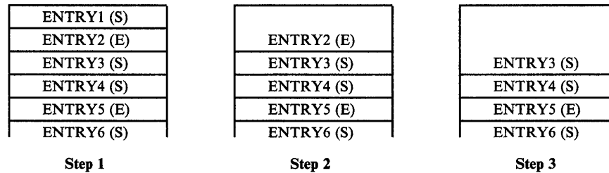
Figure 28. ENQ Macro Instruction Processing
