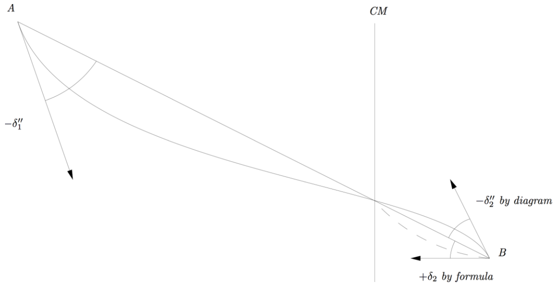
Figure C.1 Arc-to-chord correction
