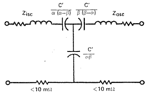
Figure 4-4. Actual equivalent circuit.
