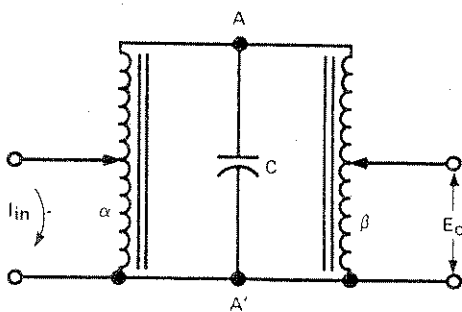
Figure 4-1. Basic circuit diagram.
