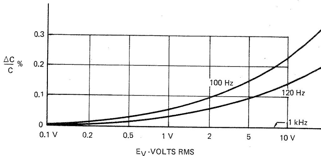
Figure 2-2. Changes in capacitance vs voltage at VOLTMETER terminals.
