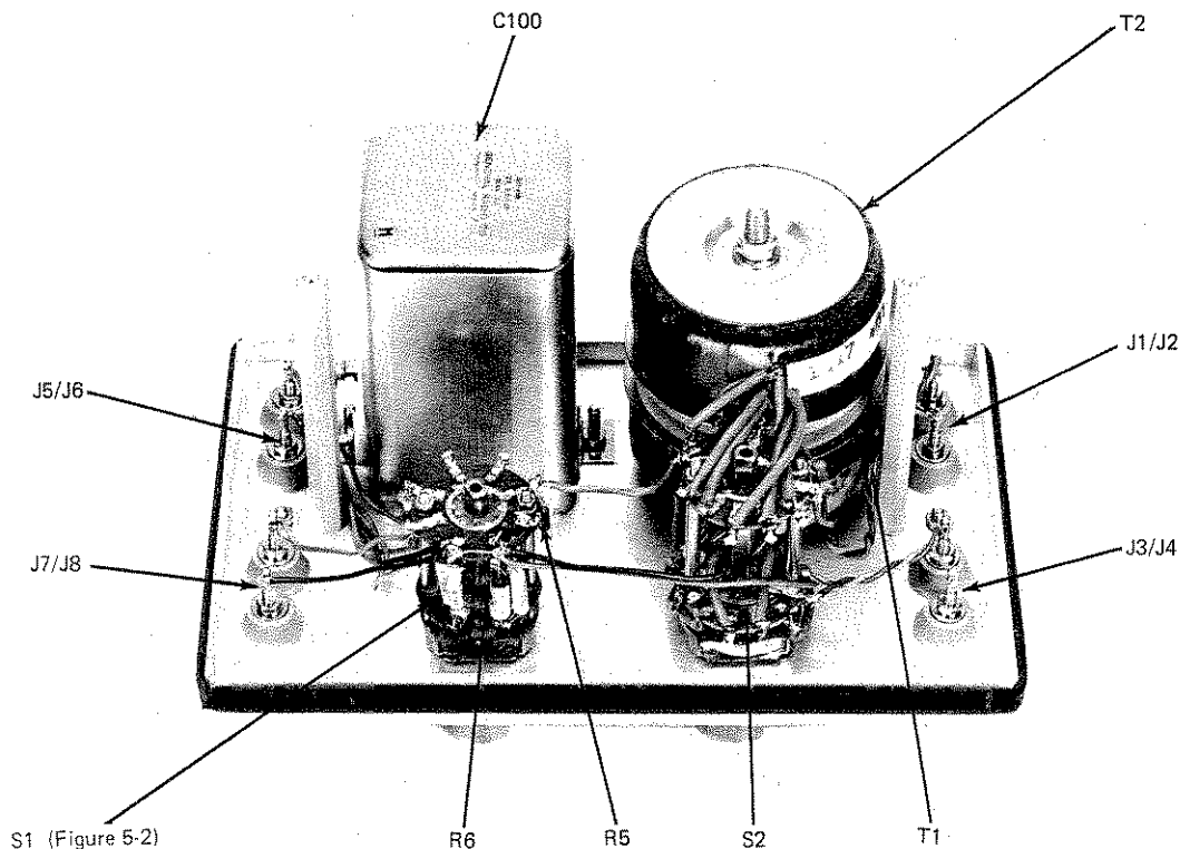
Figure 5-1. Internal view (transformer shields removed).
