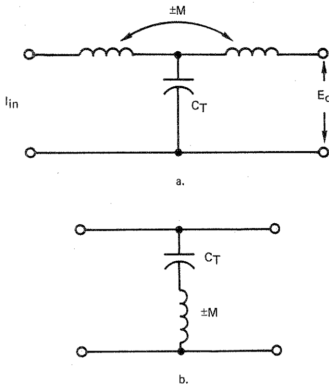
Figure 4-3. Equivalent circuits for mutual inductance errors.
