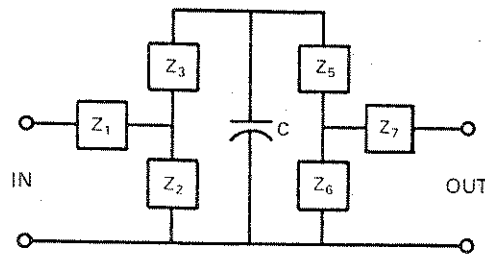
Figure 4-2. General equivalent circuit.
