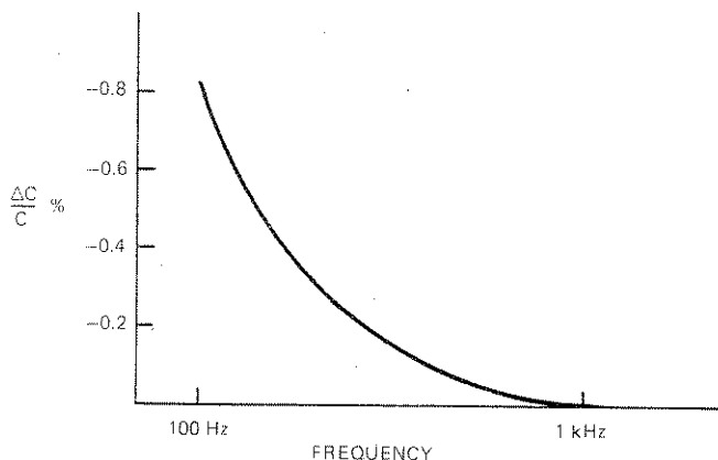
Figure 2-4. Typical capacitance change with frequency. Note corrections are made at 100 Hz and 120 Hz.
