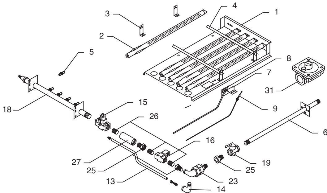
STANDING PILOT
