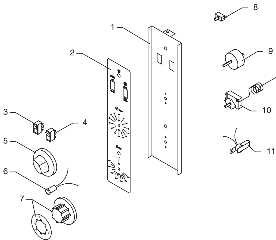
MANUAL CONTROL
