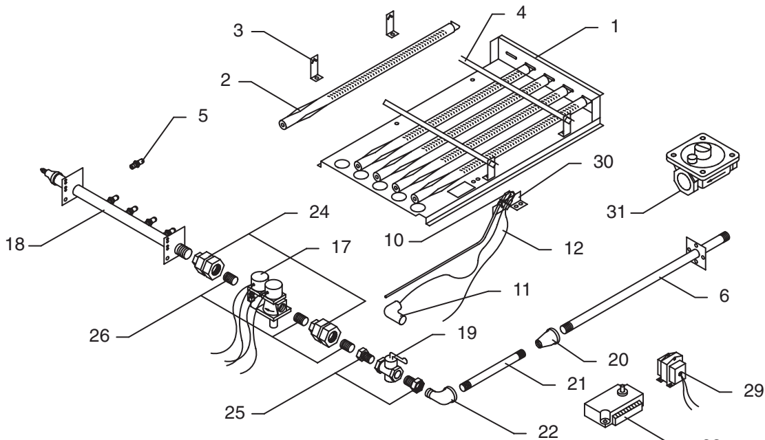
SPARK IGNITION
