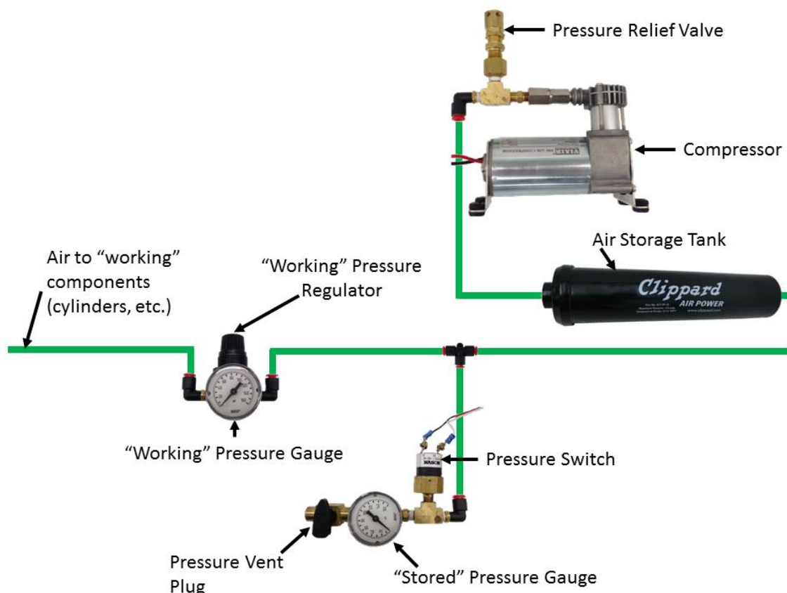
Figure 8-14: Pneumatic circuitry
