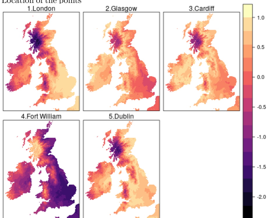
Figure 3.9: Maps of the similarity in terms of precipitation time-series
