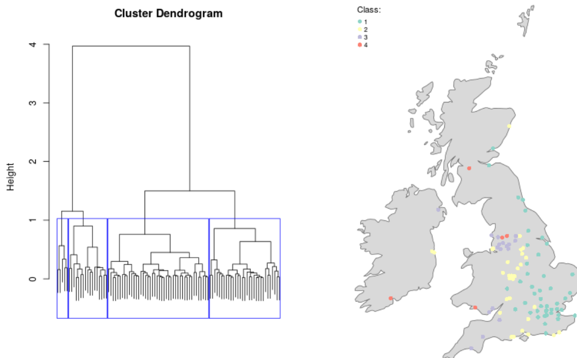
Figure 3.24: Example of a clustering of time series motifs
