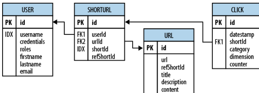
Figure 1-2. The Hush schema expressed as an ERD
