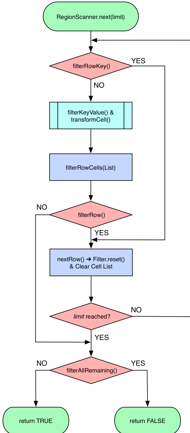
Figure 4-2. The logical flow through the filter methods for a scanner 263
