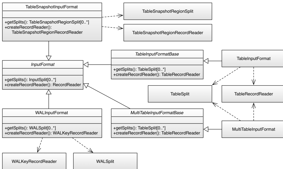
Figure 7-2. The InputFormat hierarchy
