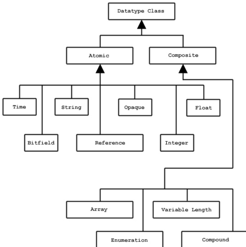
Figure 6-4. Datatype classes
