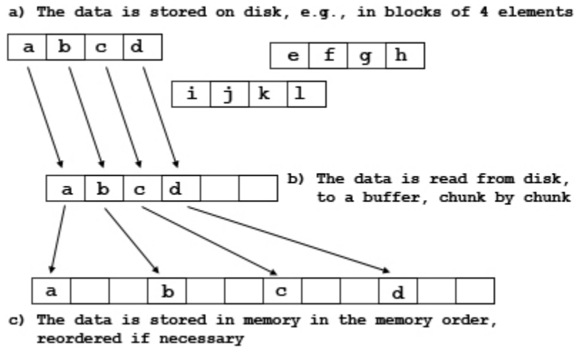
Figure 7-4. Moving data from disk to memory
