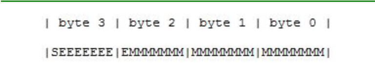
Figure 5-15. H5T_NATIVE_FLOAT in memory
