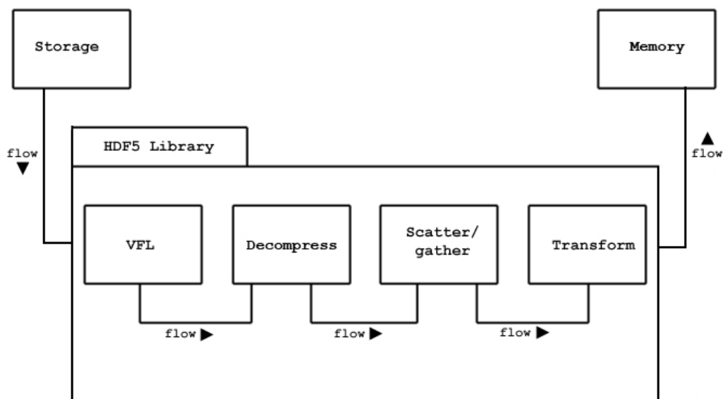
Figure 2-4. A data transfer from storage to memory
