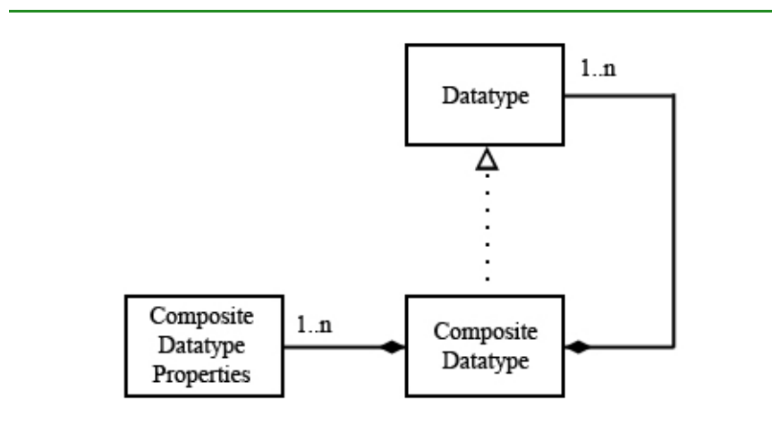
Figure 6-3. Composite datatypes
