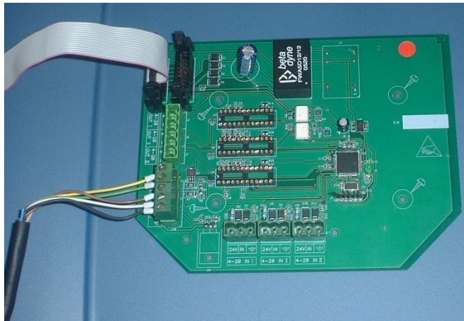
Figure 13: Connecting Turbidity Sensor to Turbidity Module
