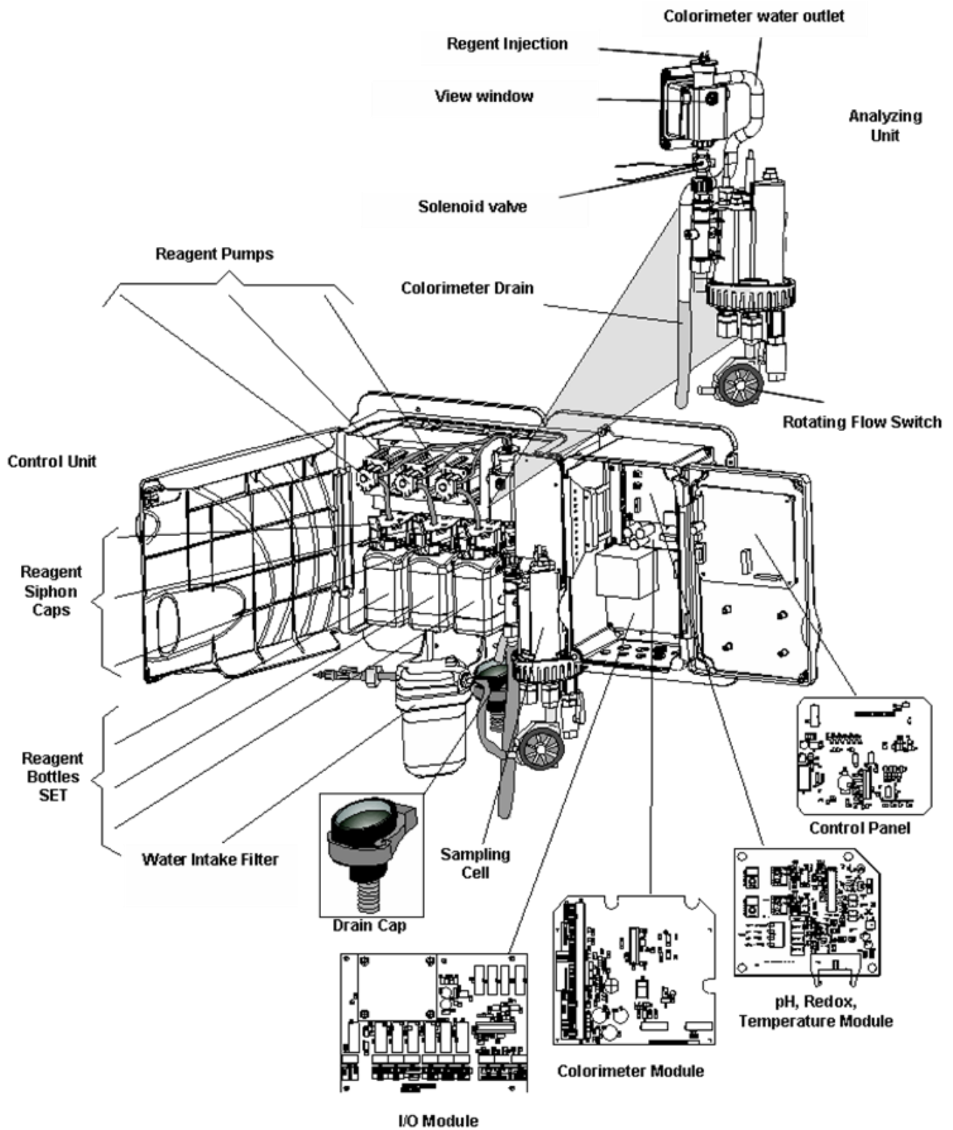
Figure 1: HYDROGUARD HG-702 Main Components
