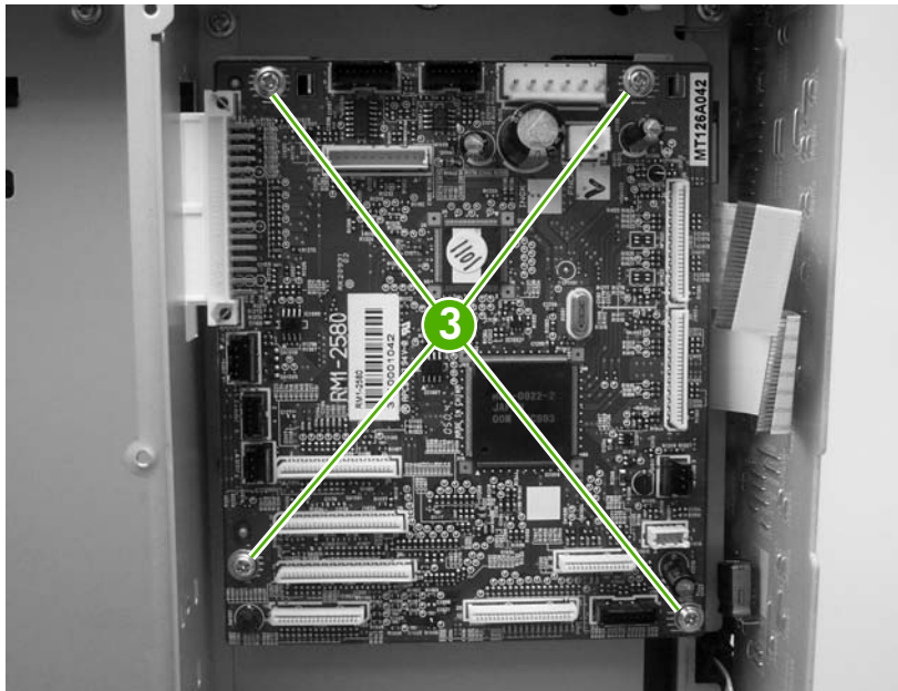
Figure 5-87 Remove the DC controller PCA (3 of 3)
