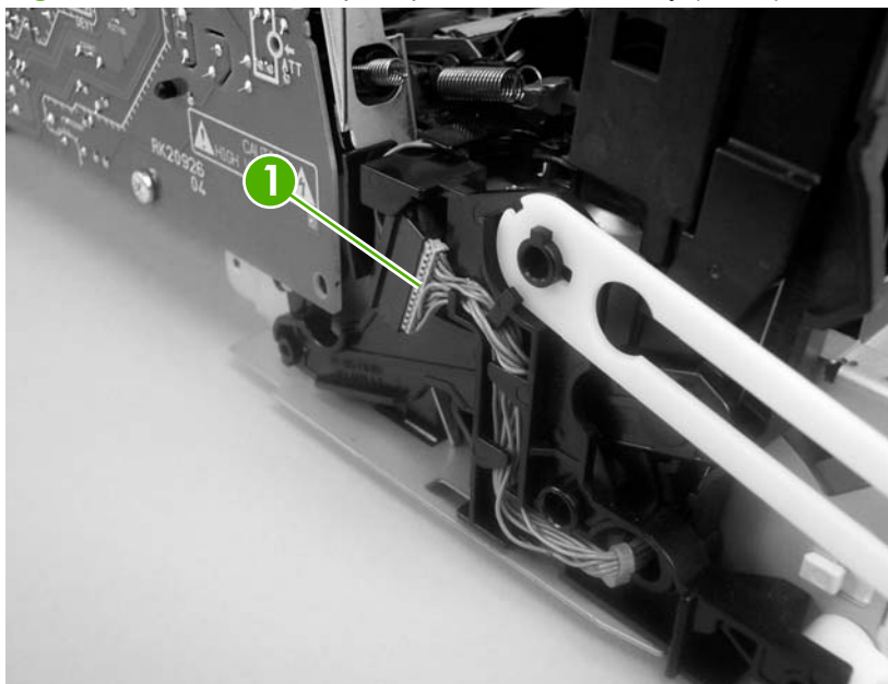
Figure 5-50 Remove the pickup-and-feed assembly (1 of 8)
