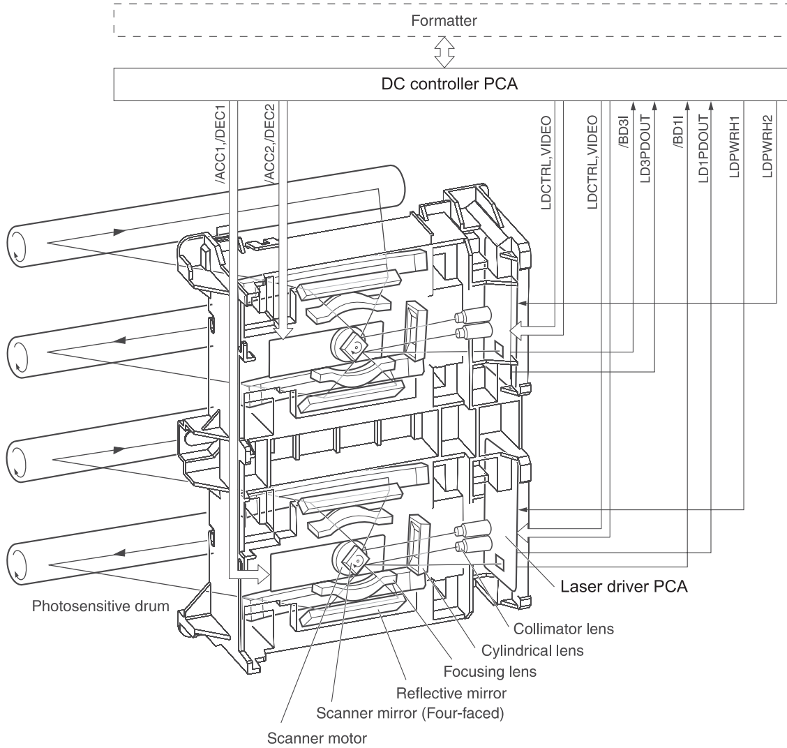
Figure 4-4 Laser/scanner system
