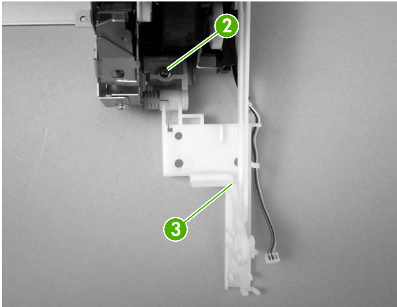
Figure 5-59 Remove the pickup-drive assembly (2 of 13)
