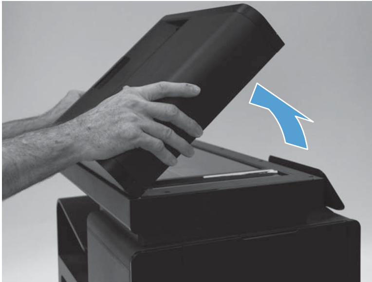
Figure 1-70 Remove the document feeder (1 of 5)
