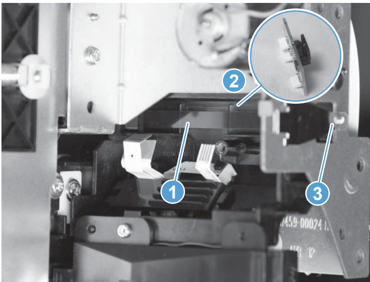
Figure 1-177 Remove the sensor carriage PCA and encoder strip (4 of 8)
