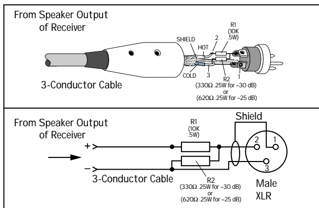
Figure 3. Speaker-level to Line-level XLR Pad
