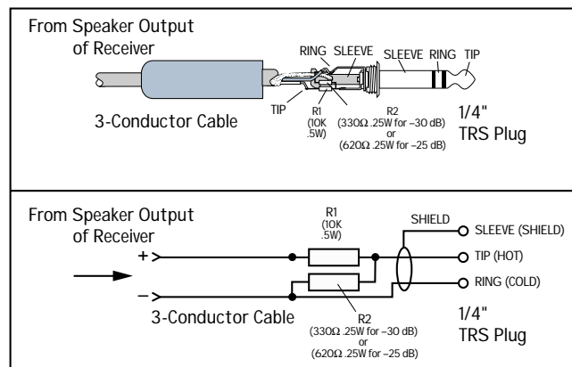
Figure 4. Speaker-level to Line-level TRS Pad
