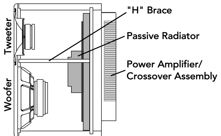
Figure 1. HR824 Cutaway side view
