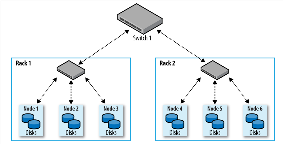
Figure 10-1. Typical two-level network architecture for a Hadoop cluster
