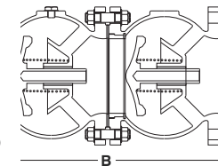
Double Check Valve configuration Fig. 2761
