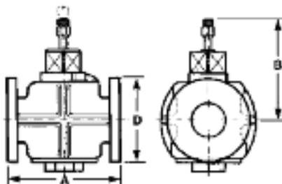
201R - Sizes 1 1/4" to 4" 4" size has bolted bottom cover
