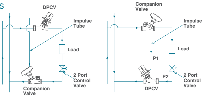
Example Flow Configuration (F300)
