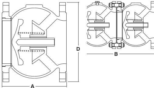
Single Check Valve Fig. 761
