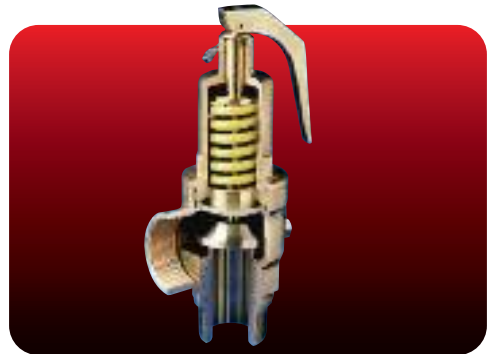
Fig. 500ST High Lift Safety Valve
