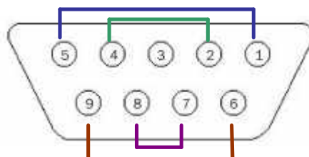
Figure 43 - RS-422/485 DB-9 connector
