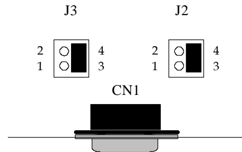
Figure 41 - RS-422/485 jumper settings
