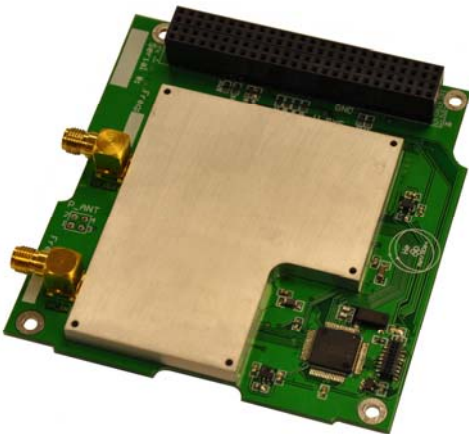
Figure 1-- He-100 radio
