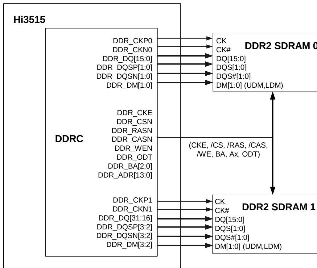
Figure 4-1 Interconnection between the DDRC and two DDR2 SDRAMs
