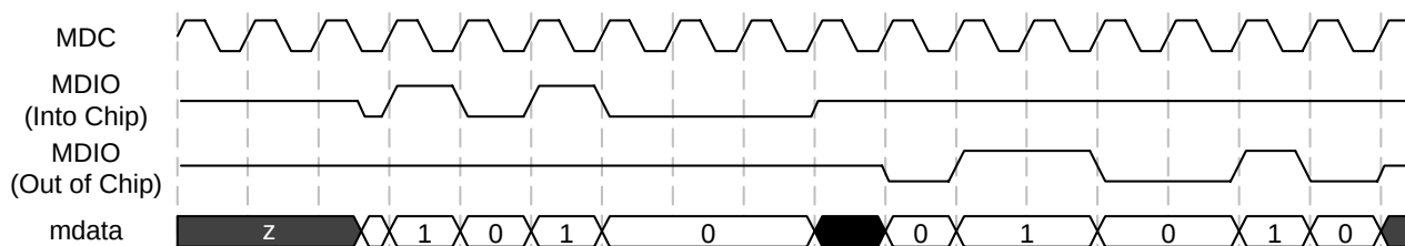
Figure 2-12 Read timing of the MDIO interface
