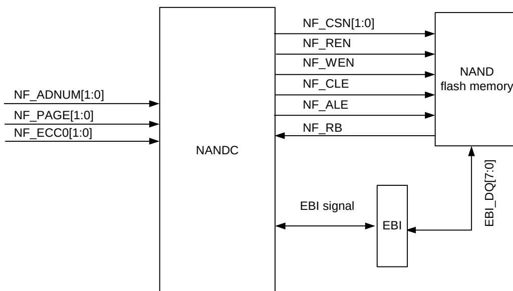
Figure 4-7 Block diagram of NANDC interfaces
