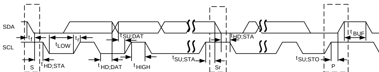
Figure 2-17 Transfer timings of the I 2 C interface
