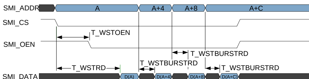
Figure 4-5 Timing diagram (page read) of the SMI controller in timing parameter mode
