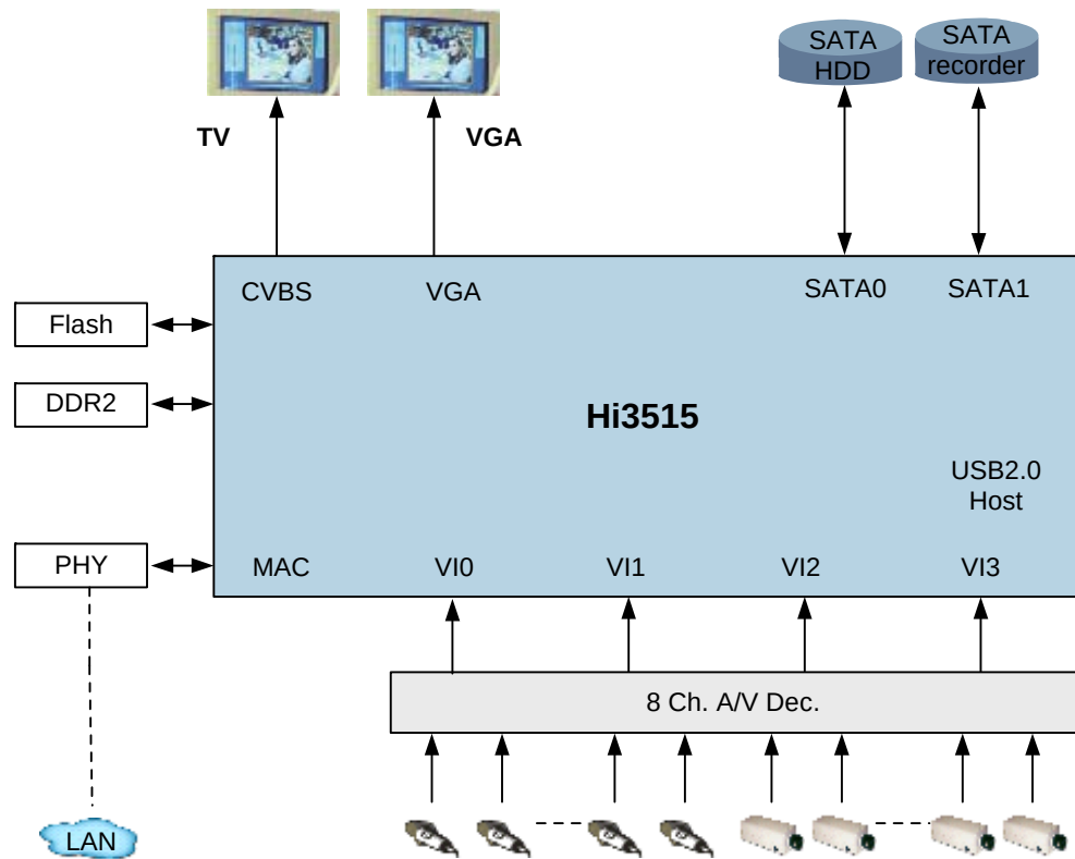
Figure 1-3 Block diagram of the Hi3515 in an 8-channel CIF DVR
