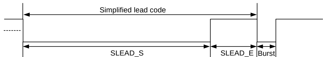
Figure 11-28 Code format for transmitting continuous NEC with simple repeat codes by holding the key down
