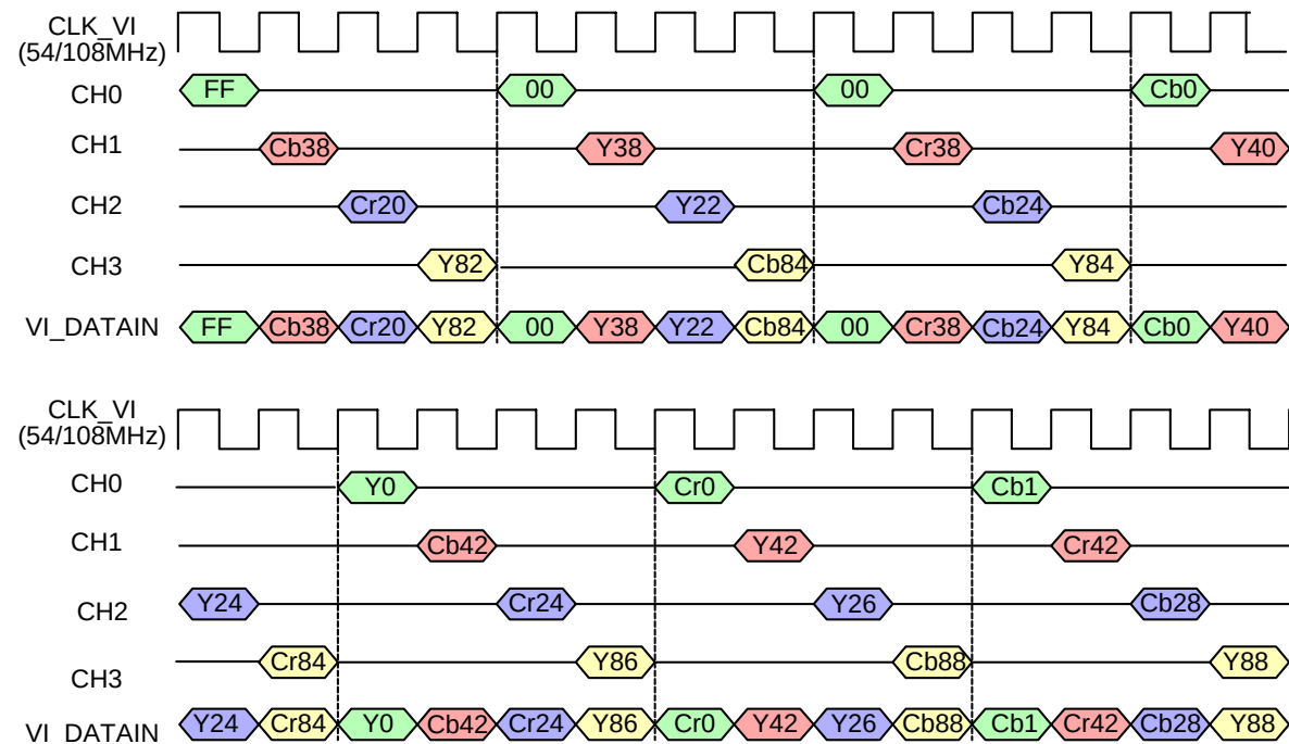
Figure 6-6 4-Path BT.656 TDM timing
