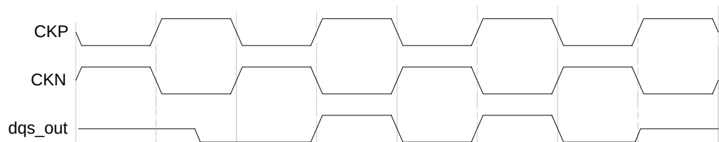
Figure 2-3 Write timing of dqs_out relative to CK
