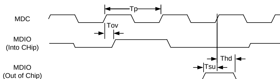
Figure 2-14 Timing parameter diagram of the MDIO interface
