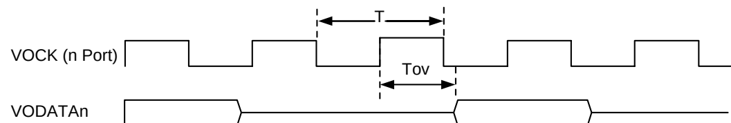
Figure 2-16 Timings of the VO interface
