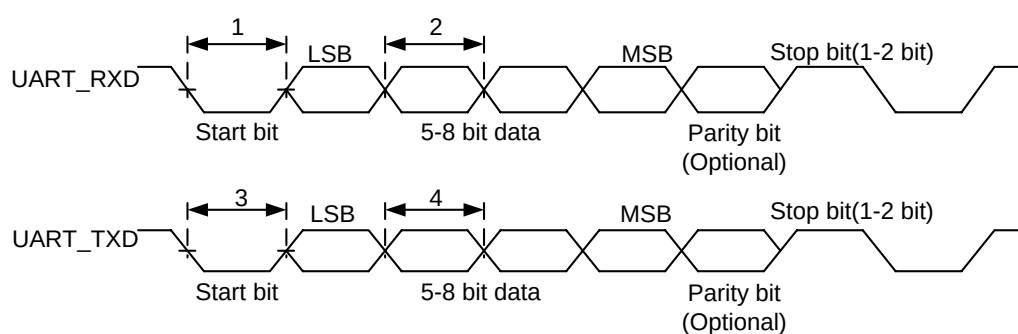
Figure 2-22 Timings of the UART interface
