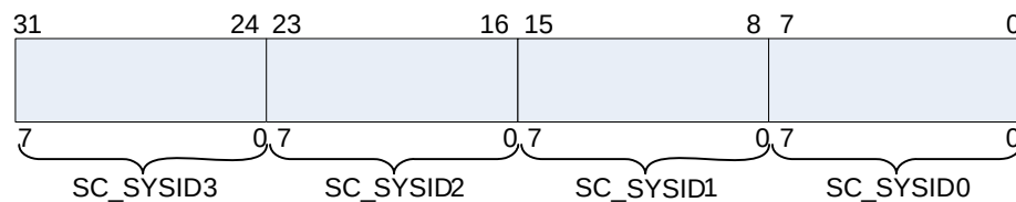
Figure 3-25 Bit allocation of chip ID registers
