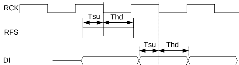
Figure 2-25 Receive timing of the PCM interface
