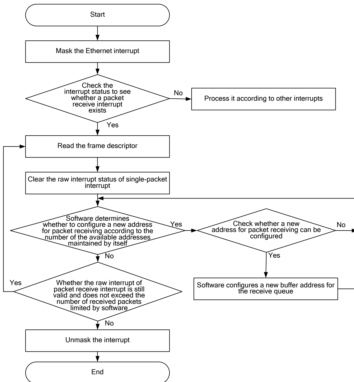
Figure 5-11 Process of receiving a frame in interrupt mode
