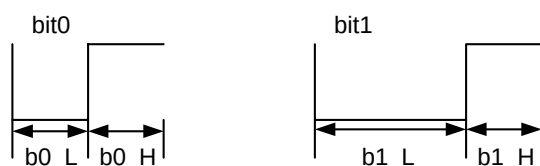
Figure 11-41 Definitions of bit0 and bit1
