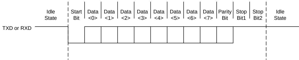
Figure 11-7 Frame format of the UART
