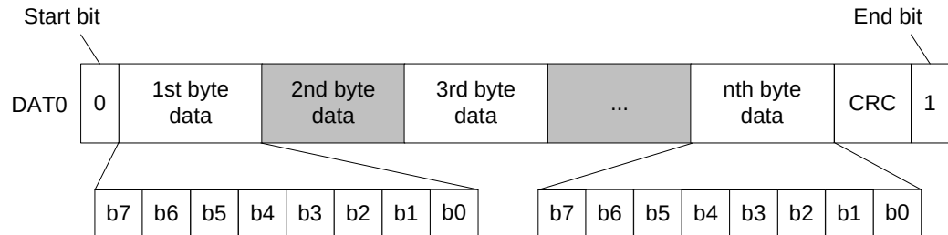
Figure 8-8 Block data format in 1-bit transfer mode
