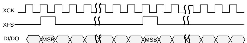
Figure 7-7 Timing diagram of the PCM interface in customized mode
