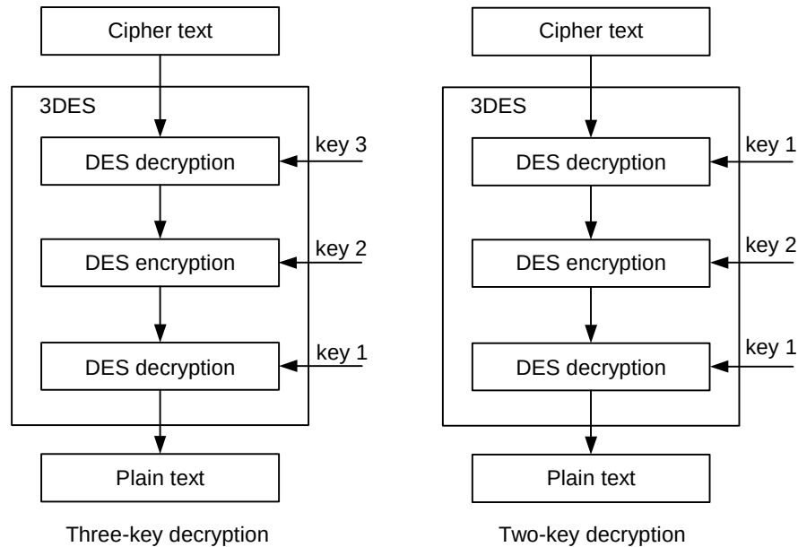
Figure 3-12 3DES decryption of the 3-key operation and 2-key operation
