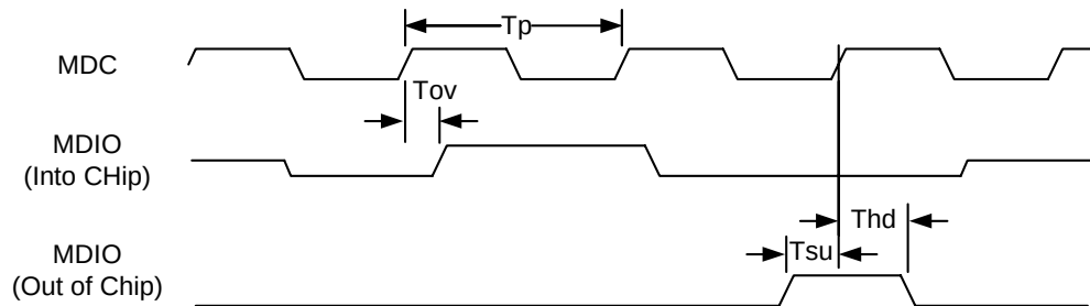
Figure 5-10 Receive timing parameters of the MDIO interface
