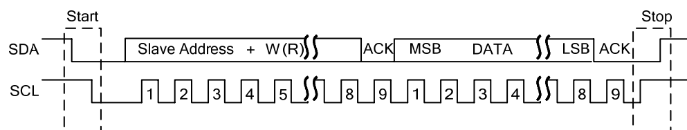
Figure 11-2 Timing for I 2 C data transfer
