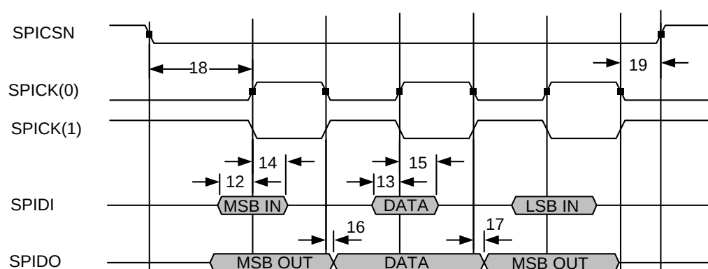
Figure 2-21 Timing of the SPI interface in master mode (sph = 1)
