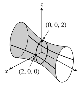
Hyperboloid of one sheet
