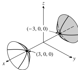
Hyperboloid of two sheets
