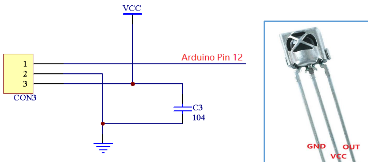
Figure .3.2.35 Circuit Diagram and Physical Map of Infrared Receiving Head
