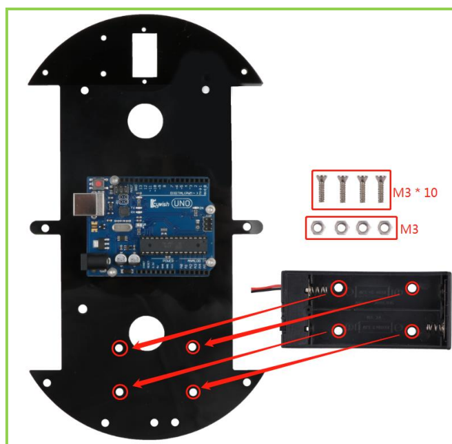
Figure 3.1.25 Schematic diagram of battery box installation
