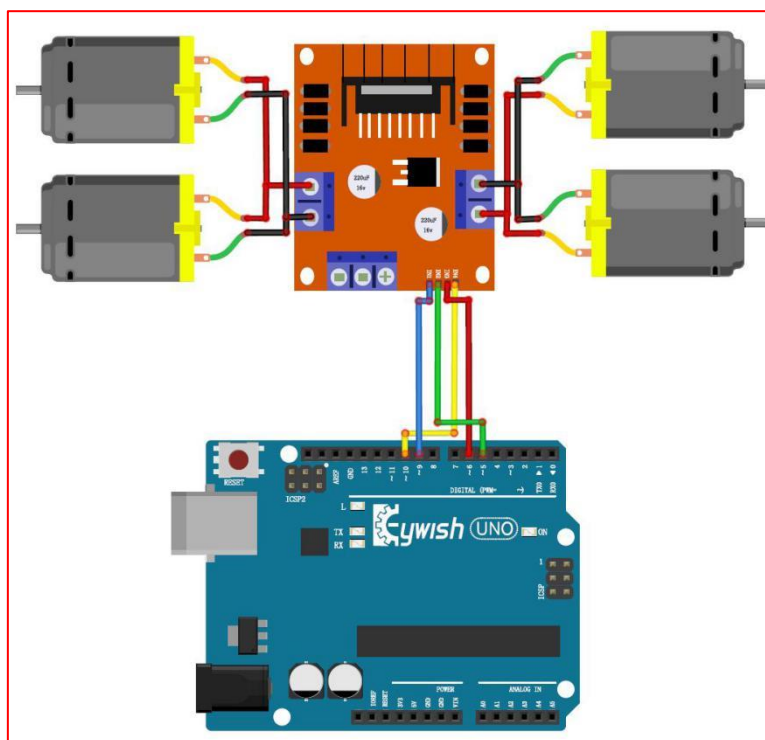
Figure .2.4.7 Arduino and L298N driver board connection diagram and connection table
