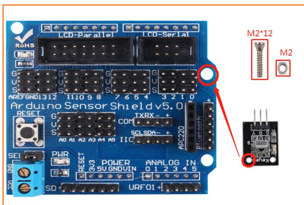
Figure 3.1.37 Schematic diagram of infrared remote control receiver installation
