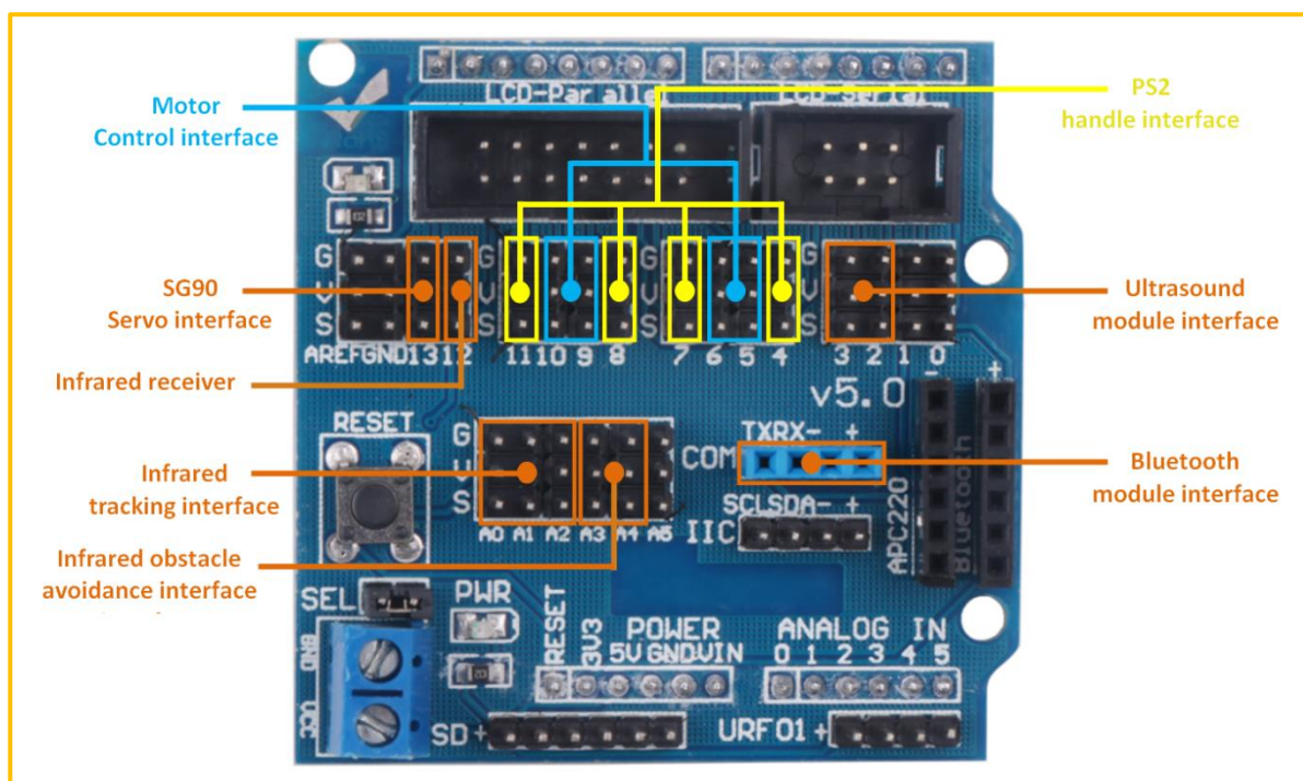
Figure 3.1.41 Expansion Board Connection Diagram
