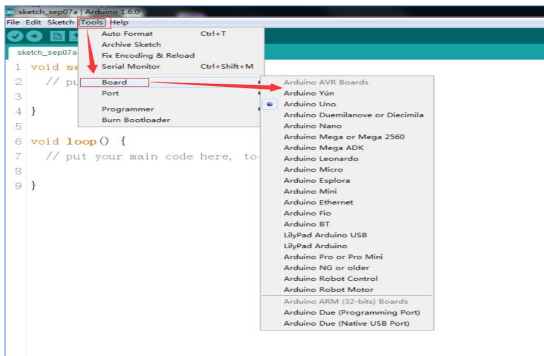
Figure 2.1.14 Tools interface
