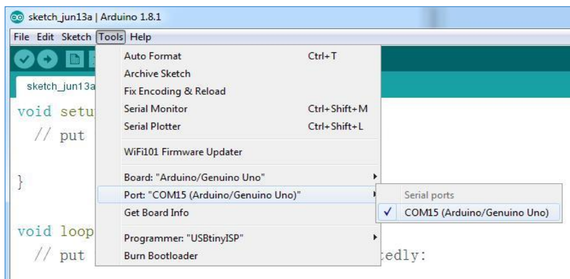
Figure 2.1.14 Tools interface
