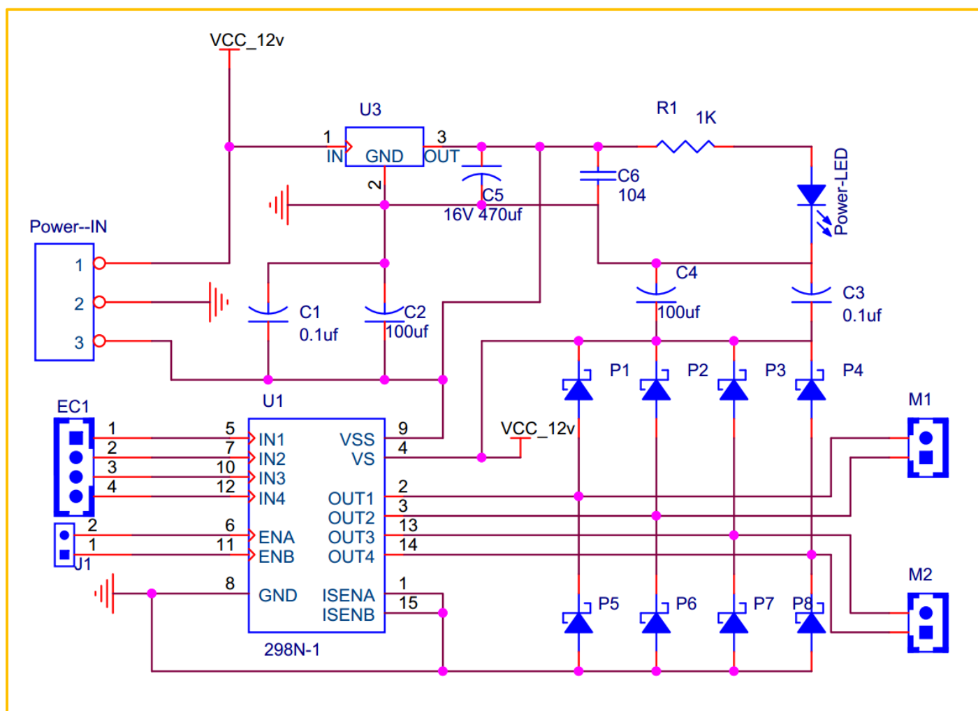
Figure .3.2.4 Schematic Diagram of Motor Drive
