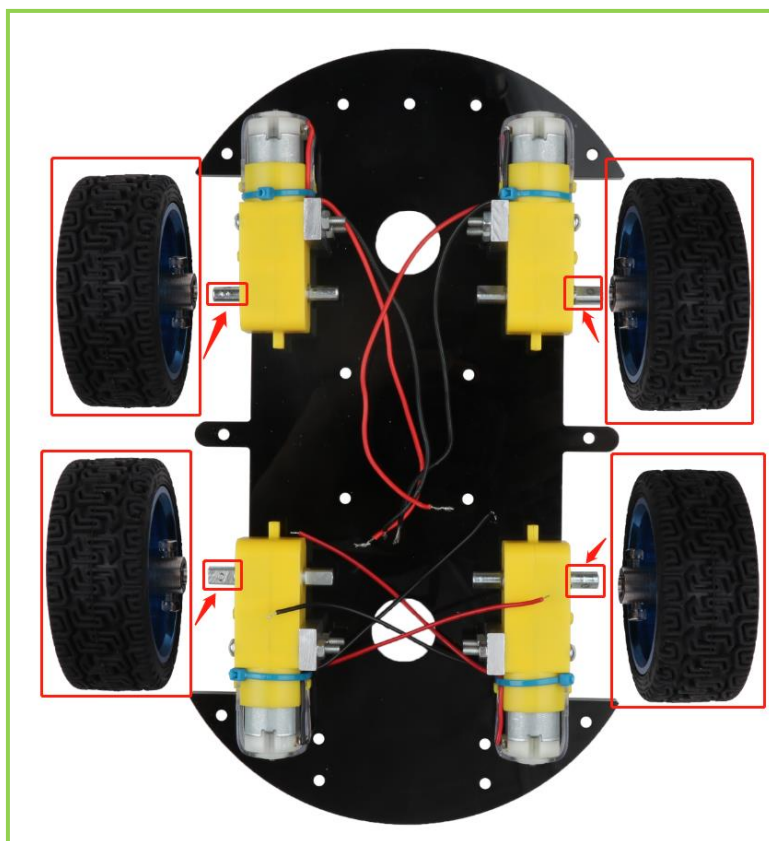
Figure 3.1.9 Schematic diagram of wheel installation
