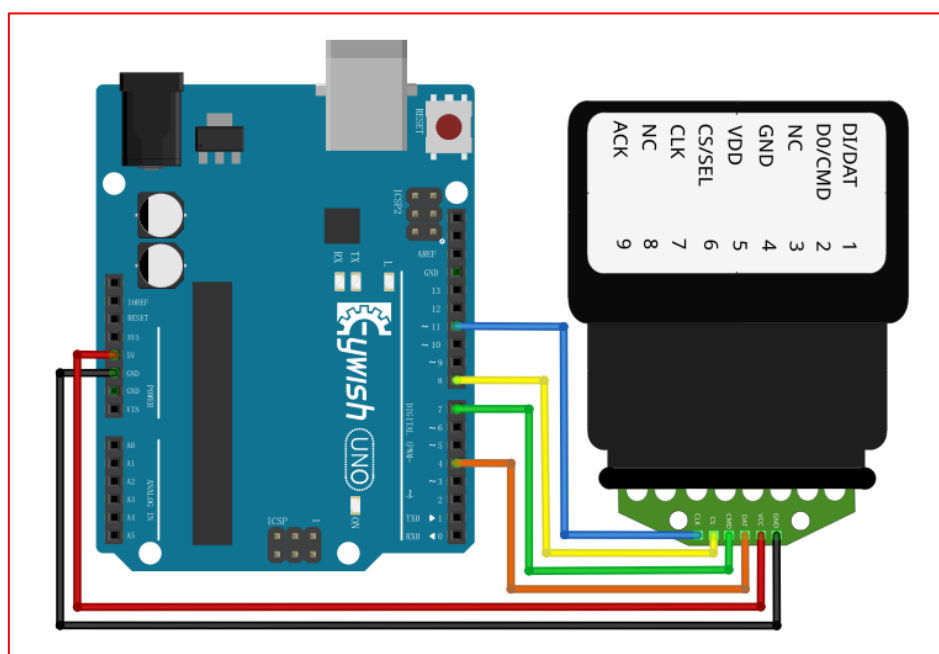
Figure 3.2.58 Connection of Arduino and Receiving Head Wires
