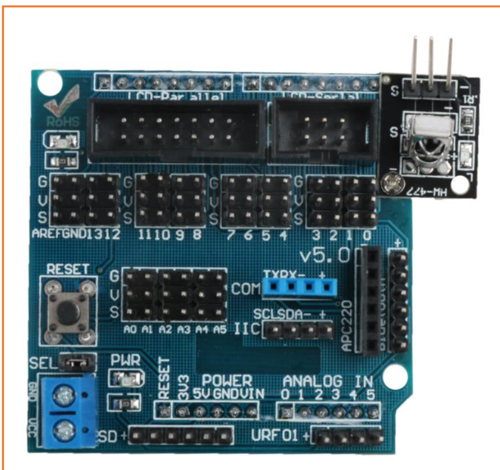
Figure 3.1.38 Effect diagram of infrared remote control receiver installation
