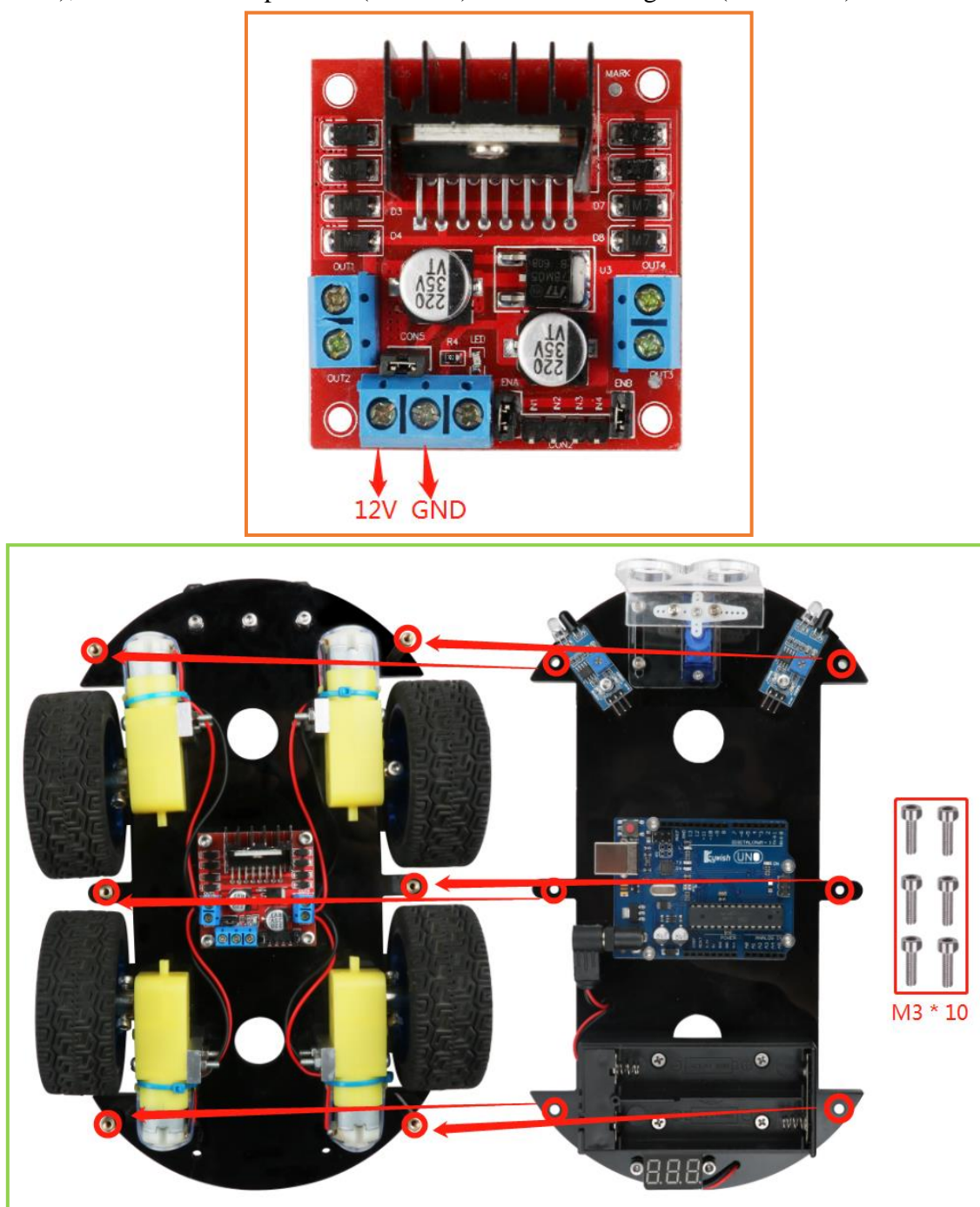
Figure 3.1.39 Schematic diagram of Overall assembly
