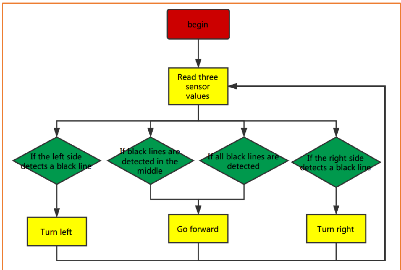
Figure .3.2.23 the Tracing Flow Chart
