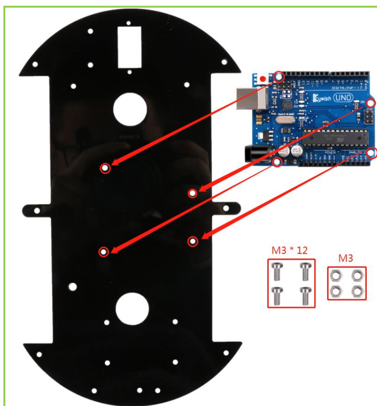
Figure 3.1.23 Schematic diagram of Keywish Uno R3 board installation
