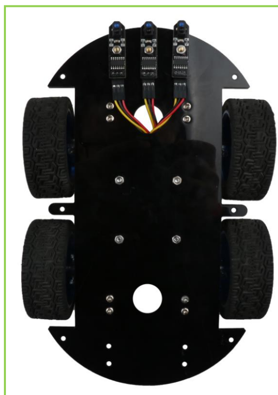
Figure 3.1.18 Effect diagram of copper column of tracking module installation
