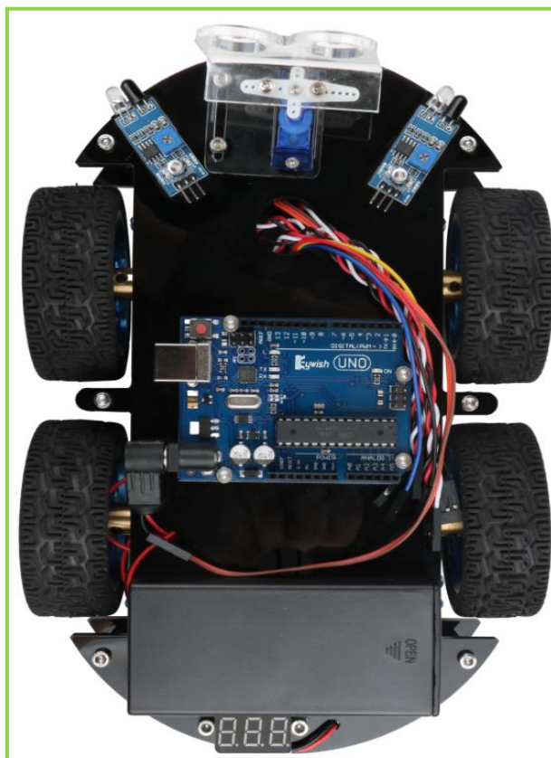
Figure 3.1.40 Effect diagram of Overall assembly
