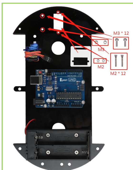
Figure 3.1.27 Schematic diagram of servo installation
