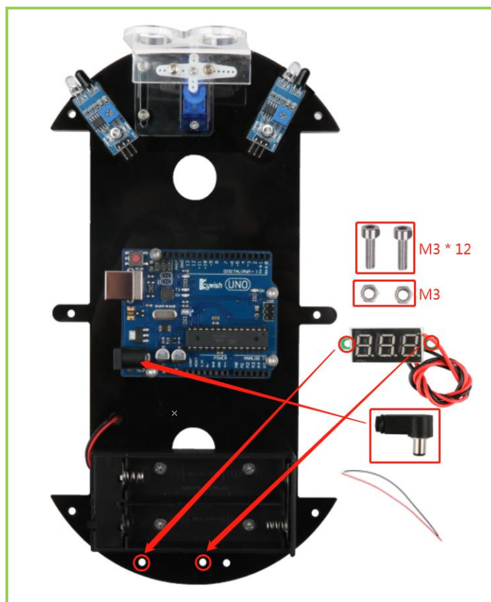
Figure 3.1.33 Schematic diagram of voltage display module and DC head installation
