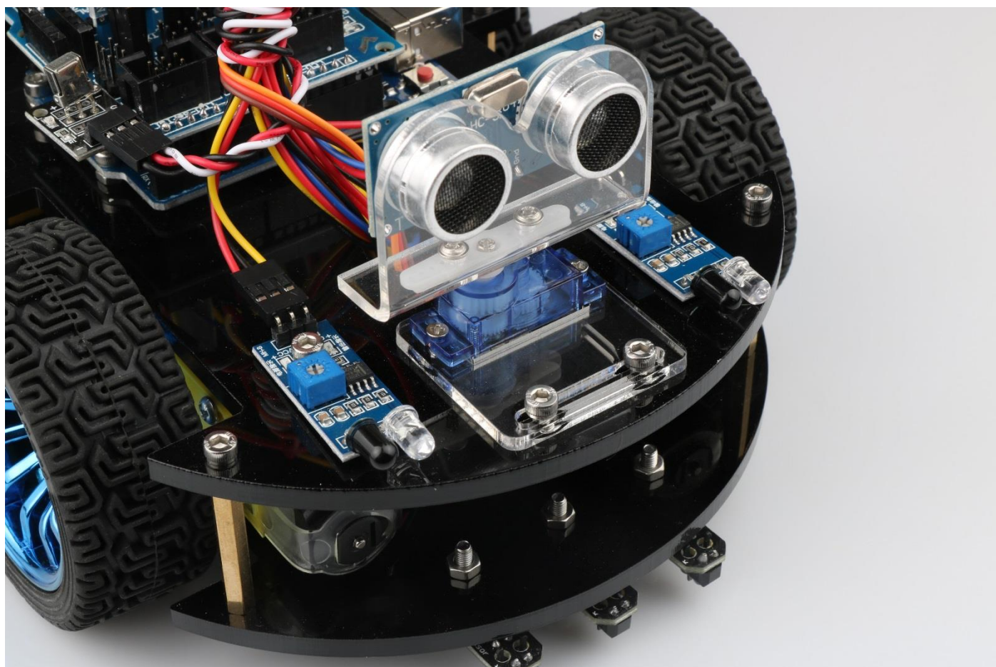
Figure .3.2.31 Installation Diagram of the Steering Gear and Ultrasonic Module
