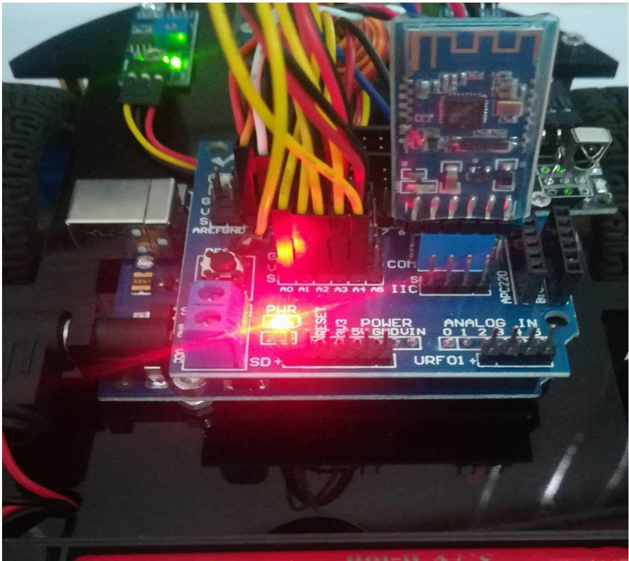
Figure .3.2.52 Installation of Bluetooth Module
