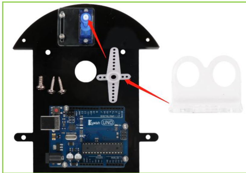
Figure 3.1.29 Schematic diagram of rudder wing and ultrasonic bracket installation
