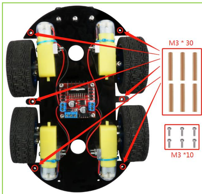
Figure 3.1.21 Schematic diagram of copper column installstion
