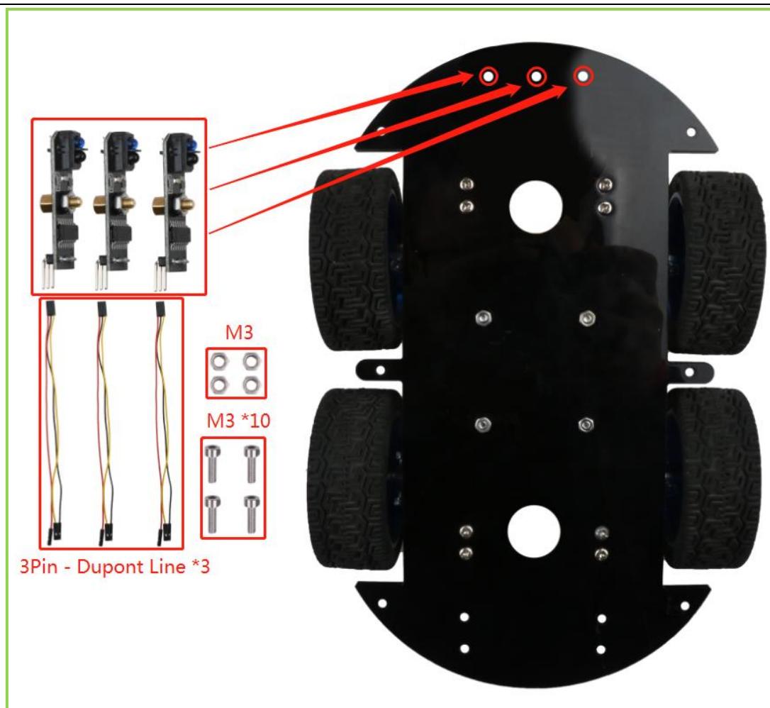
Figure 3.1.17 Schematic diagram of tracking module installation
