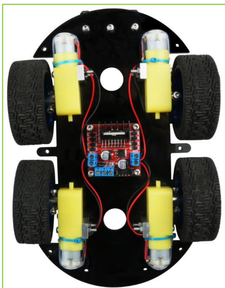
Figure 3.1.20 Effect diagram of motor wiring
