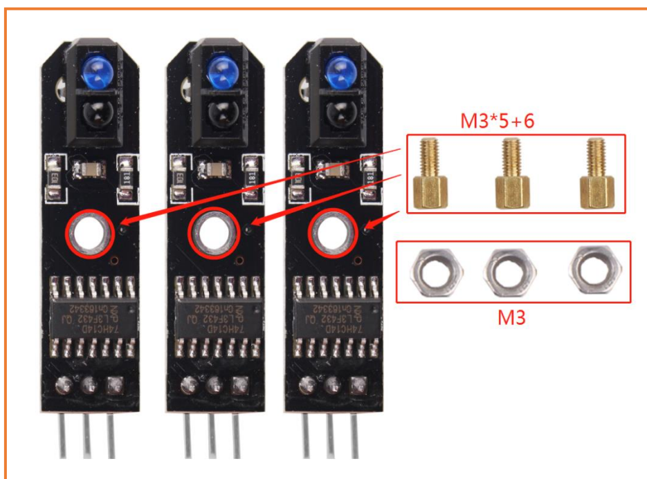
Figure 3.1.15 Shematic diagram of copper column of tracking moduble installation
