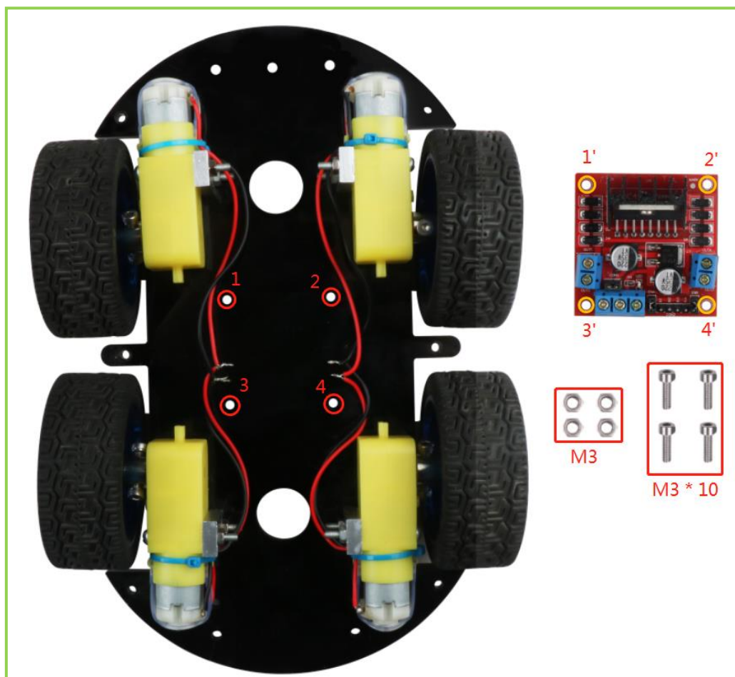
Figure 3.1.11 Shematic diagram of fixing motor driver board
