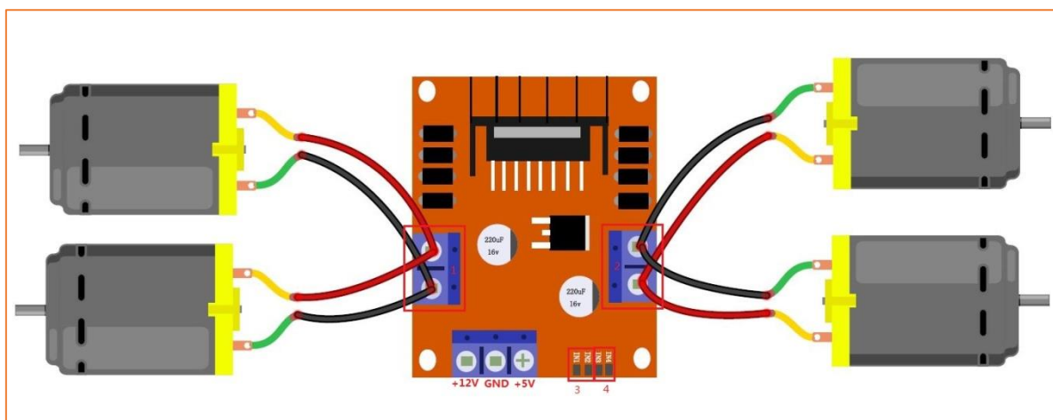
Figure 3.1.19 Schematic diagram of motor wiring
