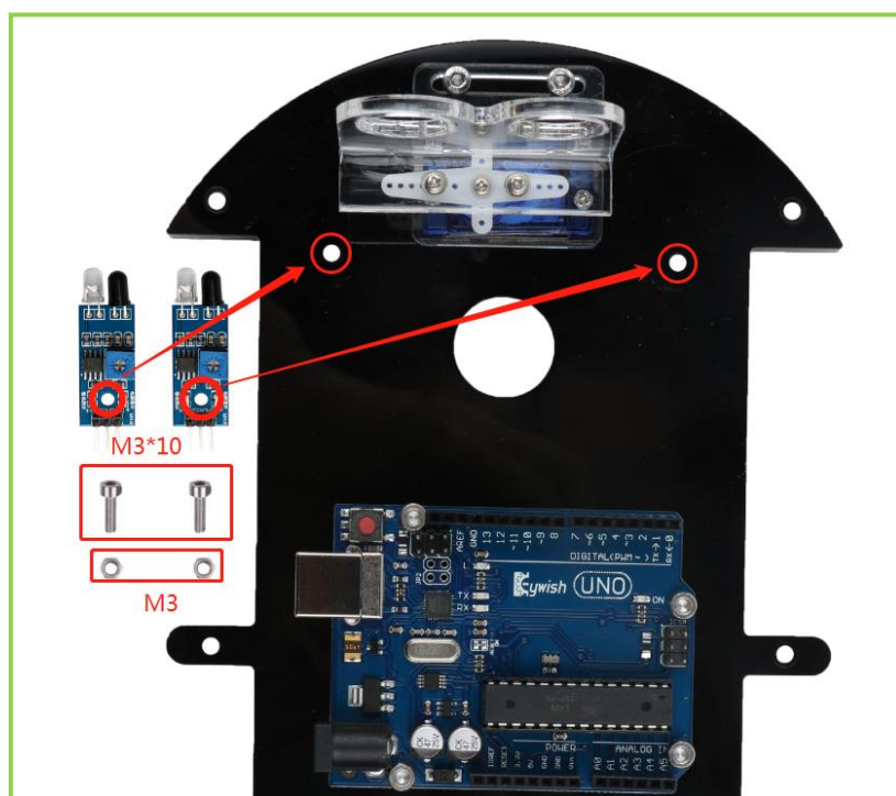
Figure 3.1.27 Schematic diagram of infrared obstacle module installation
