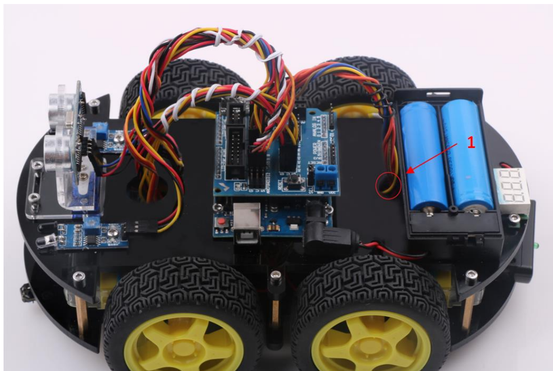
Figure 3.2.57 Wire Connection Diagram
