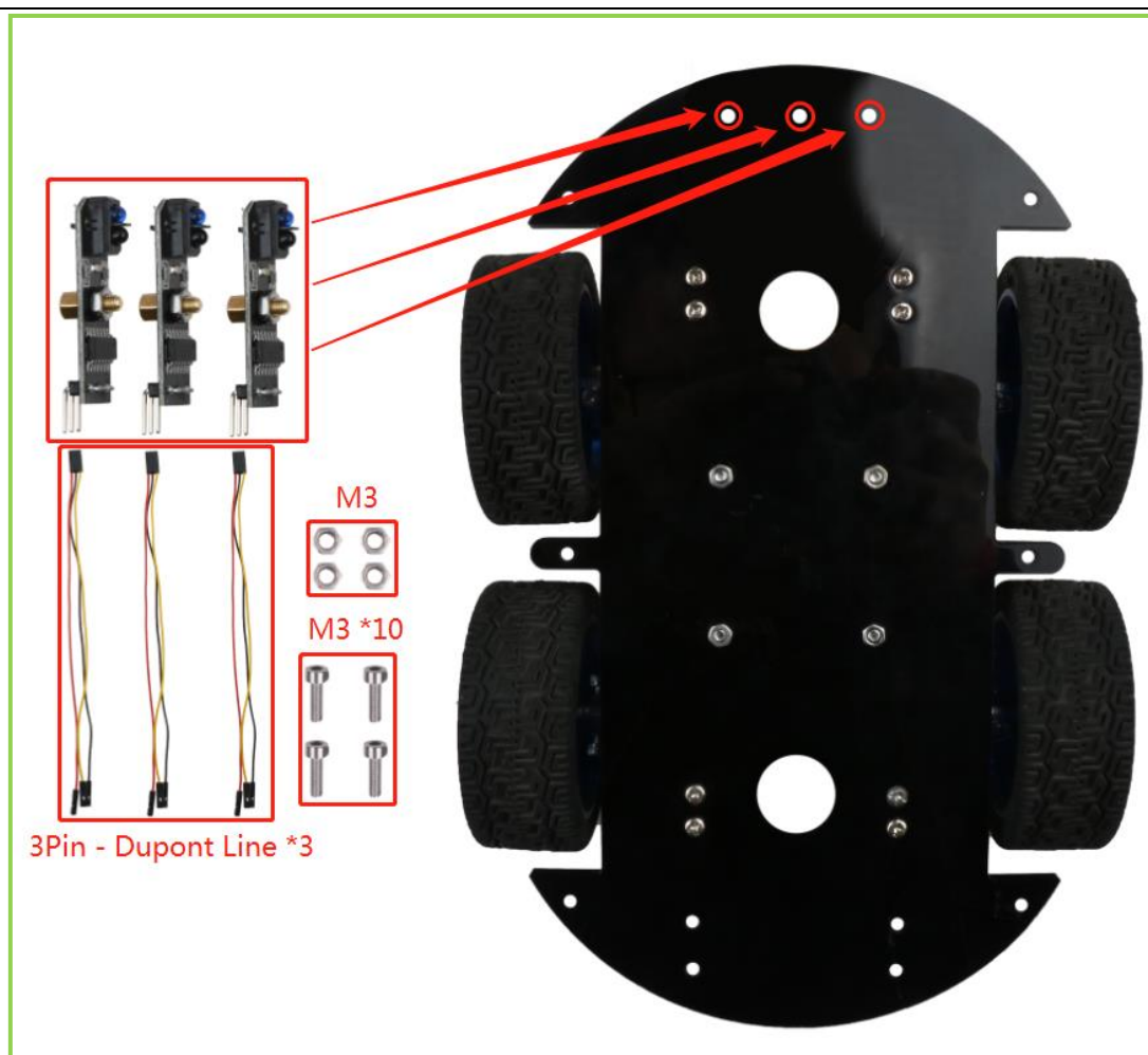
Figure 3.1.13 Shematic diagram of tracking moduble installation
