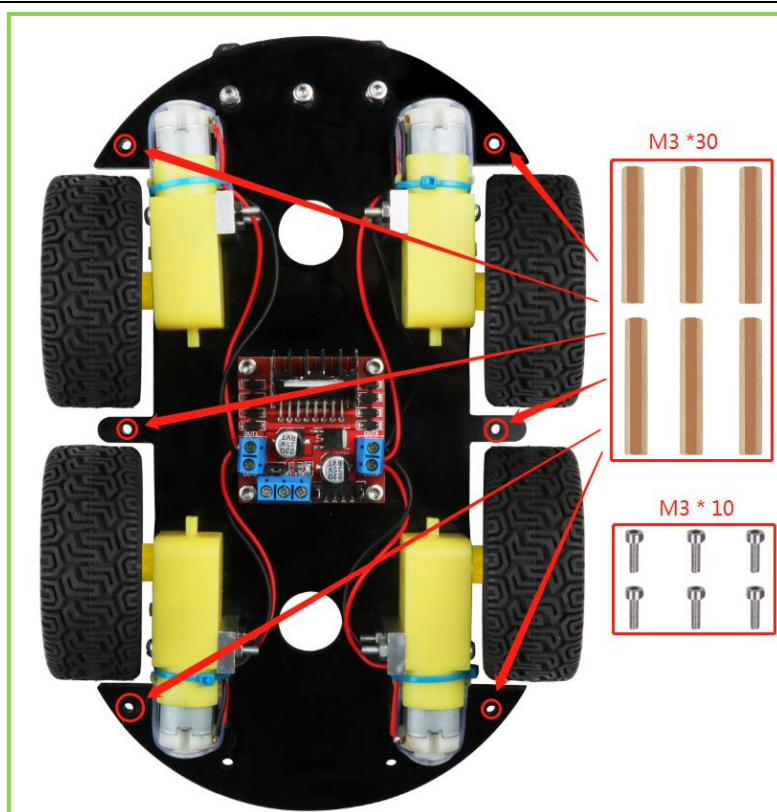
Figure 3.1.17 Schematic diagram of copper column installstion
