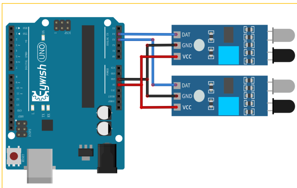
Figure .3.2.11 Connection of Arduino and Sensor
