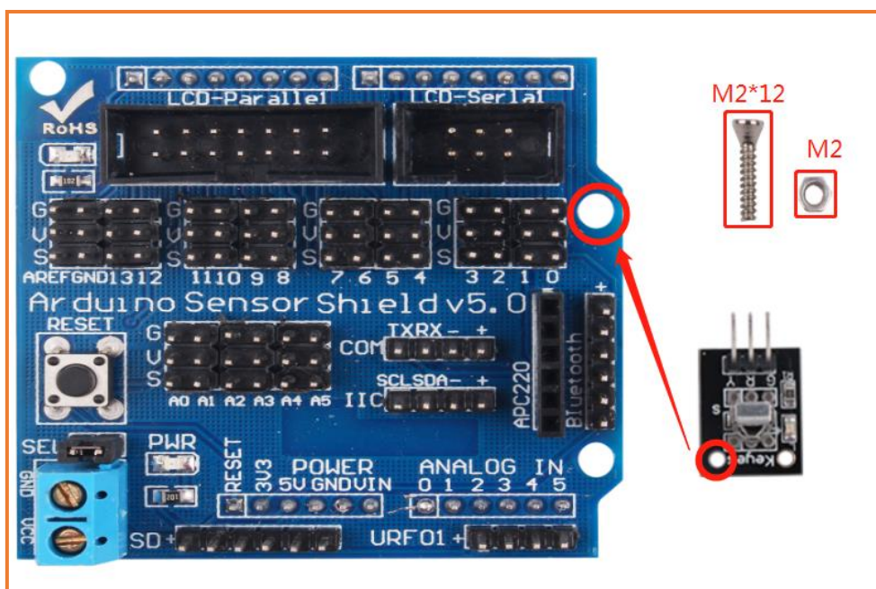
Figure 3.1.33 Shematic diagram of infrared remote control receiver installation
