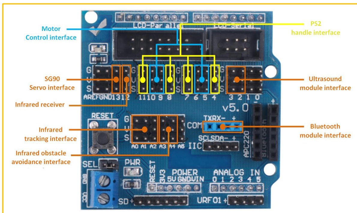
Figure 3.1.37 Expansion Board Connection Diagram
