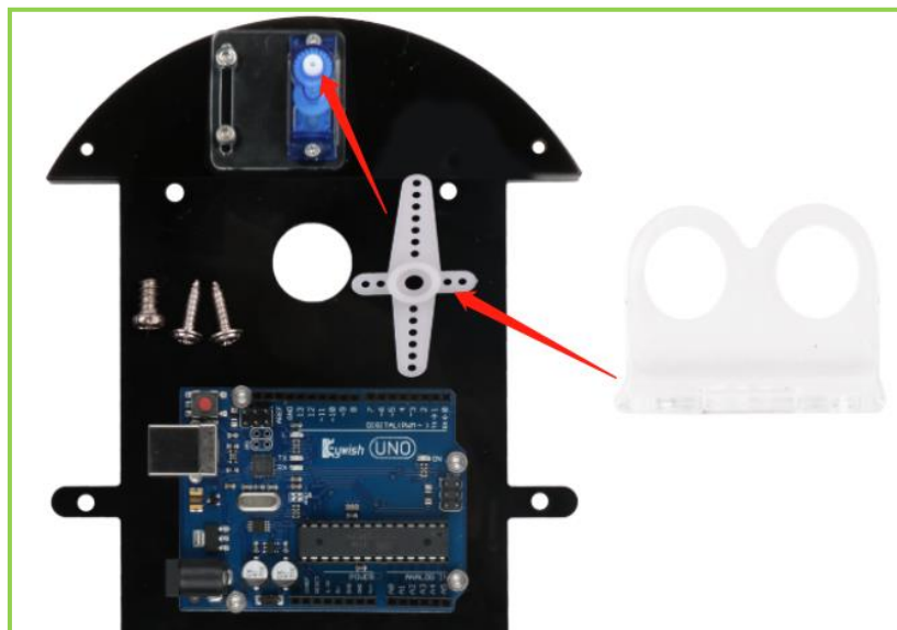
Figure 3.1.25 Schematic diagram of rudder wing and ultrasonic bracket installation
