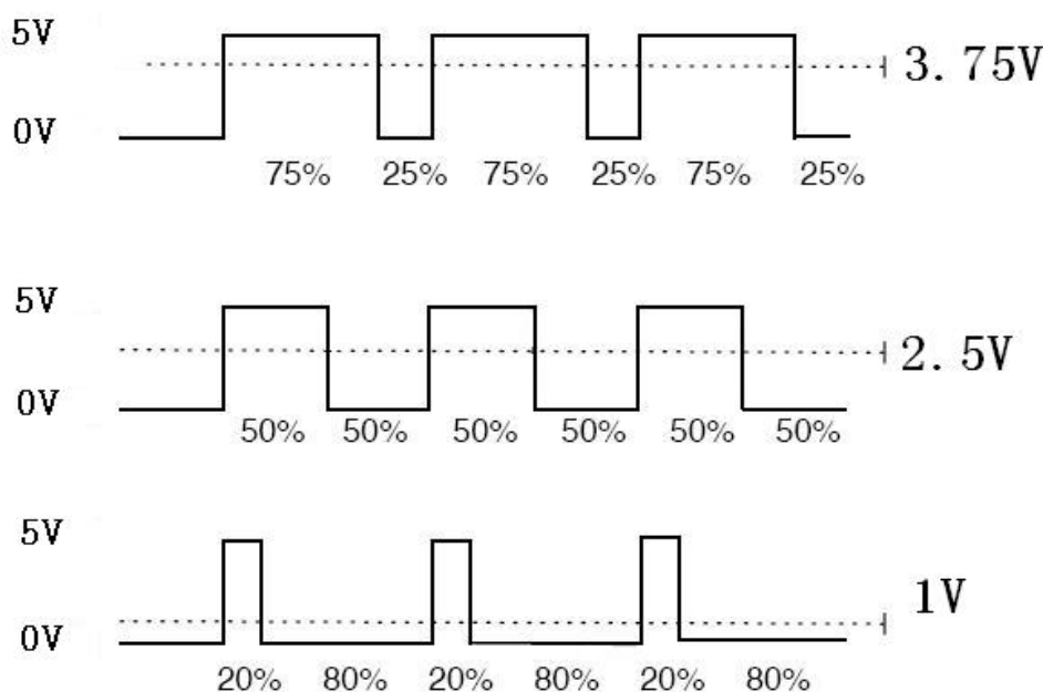
Figure .2.4.6 Relation between Pulse and Voltage
