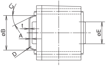
Figure 5.14 Frame Size 1100
