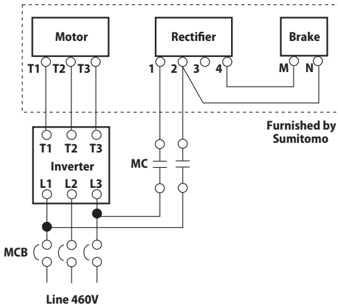
Figure 5.38 Fast Brake Action, 460V
