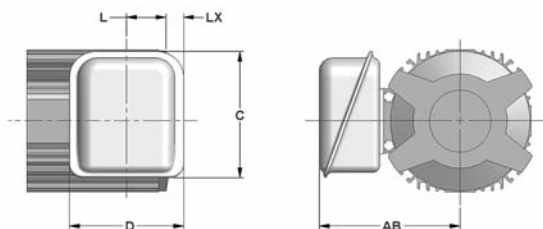
Figure 5.22 Non-UL Indoor Duty
