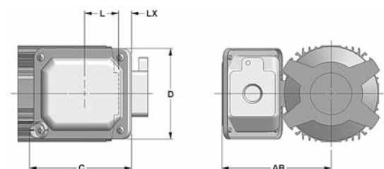
Figure 5.24 Non-UL &amp; UL Washdown Duty
