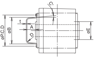
Figure 5.15 Frame Sizes 1200 ~1600
