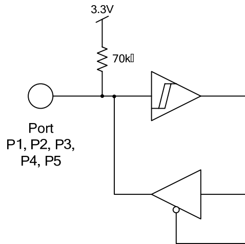
Figure 9. Port Structure of IRMCx300
