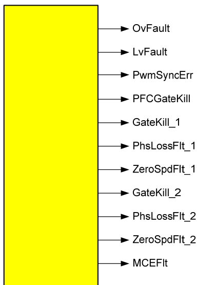
Figure 72. FAULTS Block
