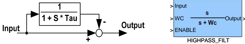
Figure 19. HIGHPASS_FILT Block
