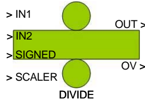
Figure 44. DIVIDE Block
