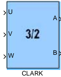
Figure 23. CLARK Block
