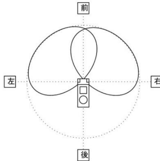
Attached Microphone Stereo Recording
