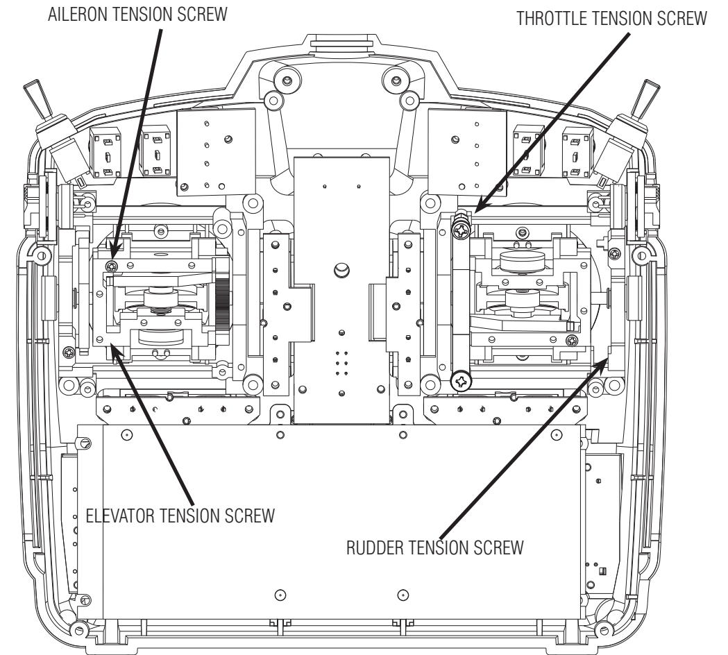
Back of Transmitter (Mode 2)
