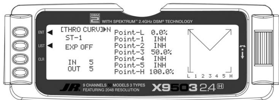
Figure 2: Throttle Curve, Stunt 1
