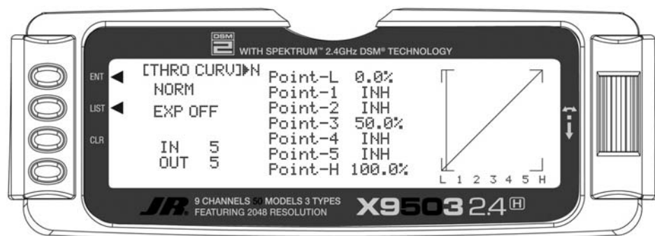
Figure 1: Throttle Curve Normal
